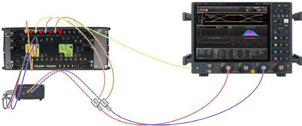
Figure 7. N5991U42A test solution for USB4 Version 2.0 receiver calibration
