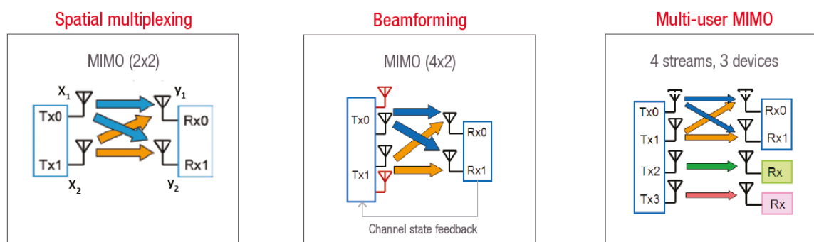
Figure 1. MIMO techniques
