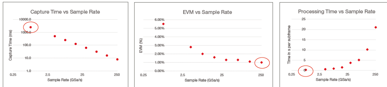
Figure 4. Speed versus performance in 5G NR EVM
