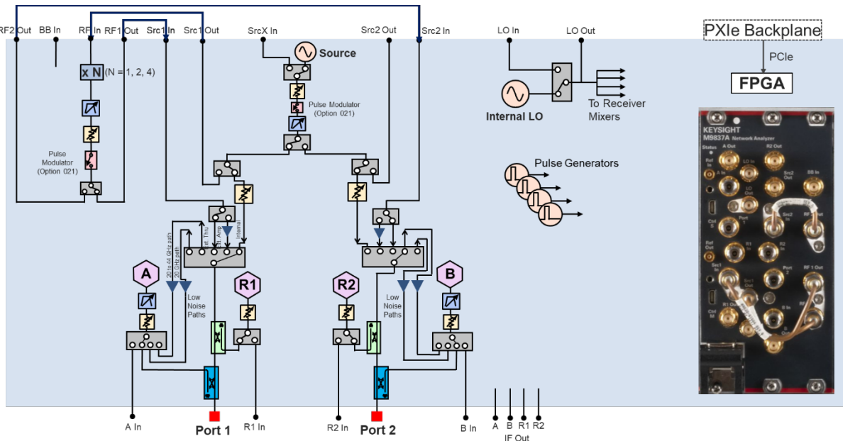
M9837A Option 205 (2-port base model without upconverter)
