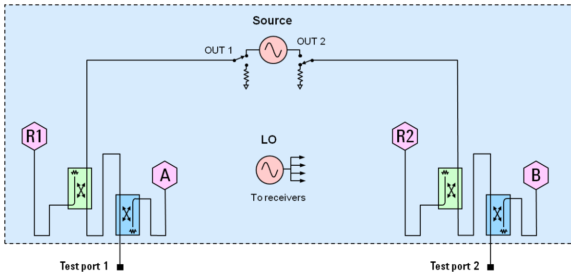
N5227B Option 210 (2-port metrology configuration)
