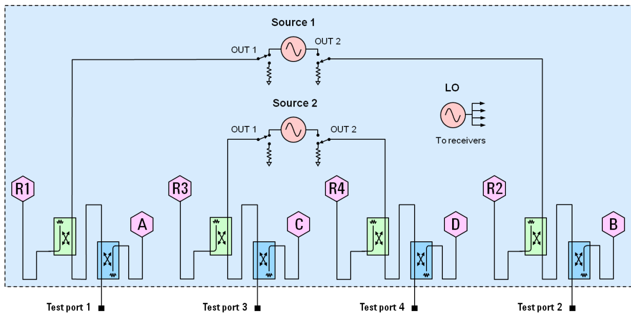
N5227B Option 410 (4-port metrology configuration)
