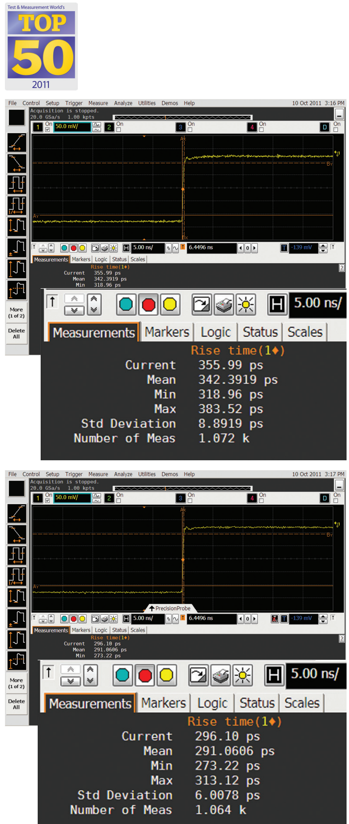
Figures 1 and 2. Cable loss degrades rise times and causes measurement non-repeatability. Figure 1 shows the rise time of a signal with a cable that's loss is uncharacterized and not compensated. Figure 2 shows the same measurement with characterization and compensation. Notice the rise time is >15% faster and the measurement is nearly 50% more repeatable.
