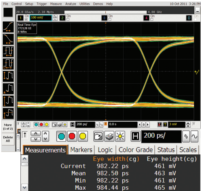
Figure 15. Real time eye with uncorrected cable loss
