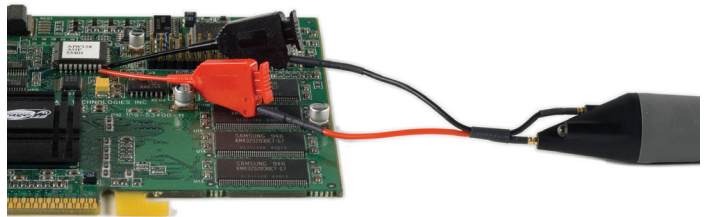
Figure 4. Image of custom probe
