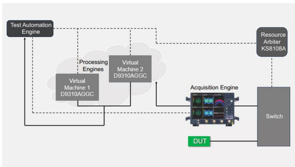
Figure 1. Keysight D9310AGGC Measurement Server setup
