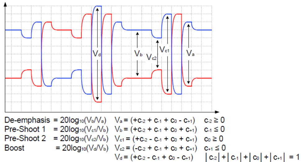
Figure 114 Definition of Tx Voltage Levels and Equalization Ratios
