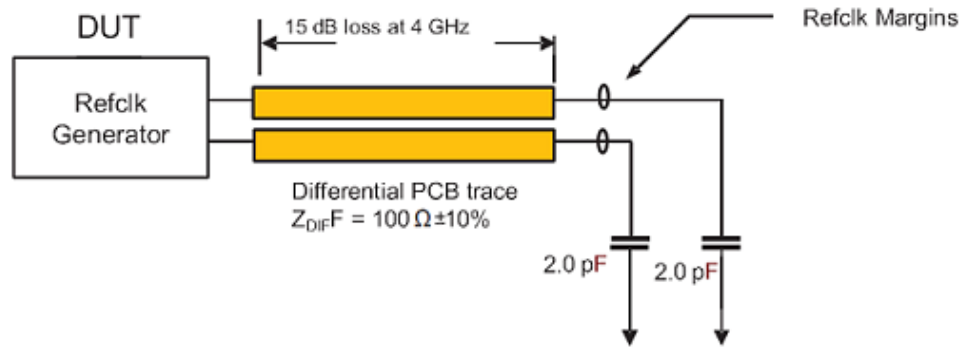
Figure 27 Driver Compliance Test Load
