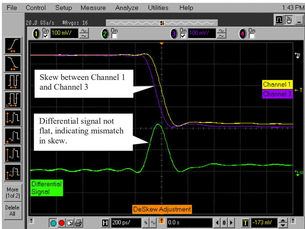
Figure 21 Channel Skew.
