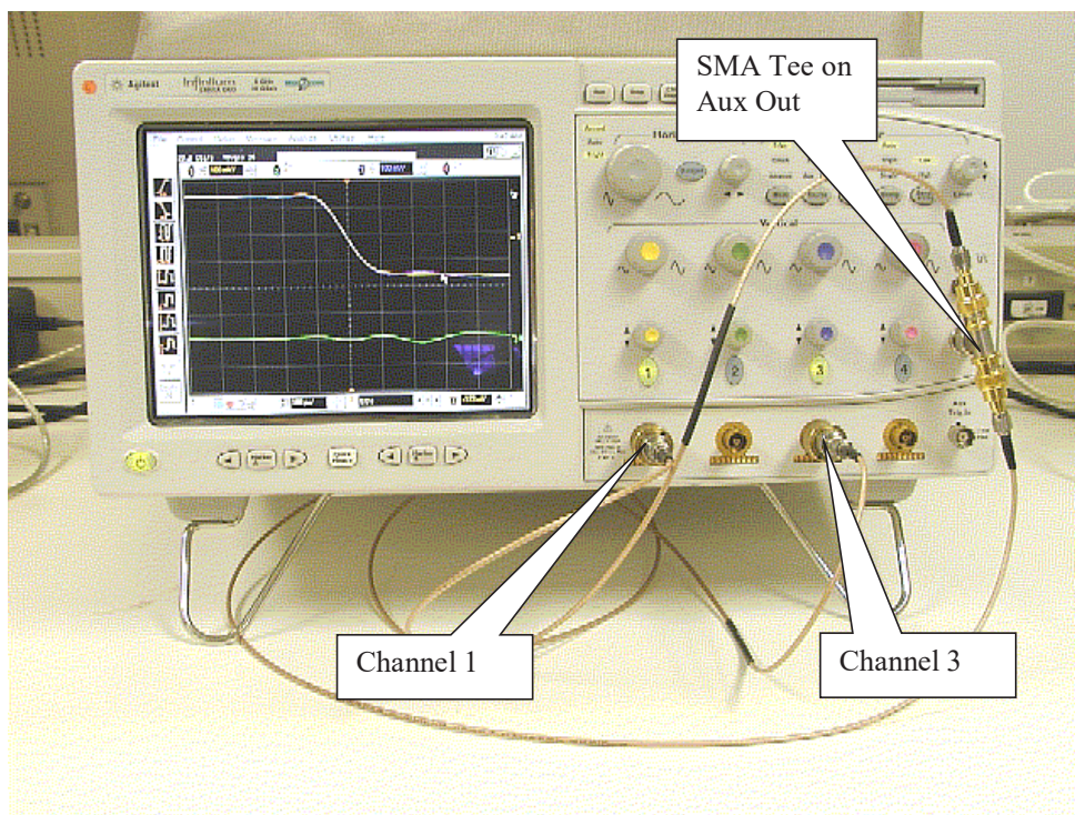
Figure 19 De-skew Connection.
