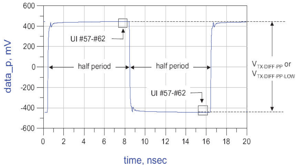
Figure 176 V_{TX-DIFF-PP} Measurement
