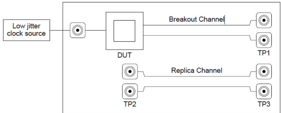
Figure 173 Driver Compliance Test Load
