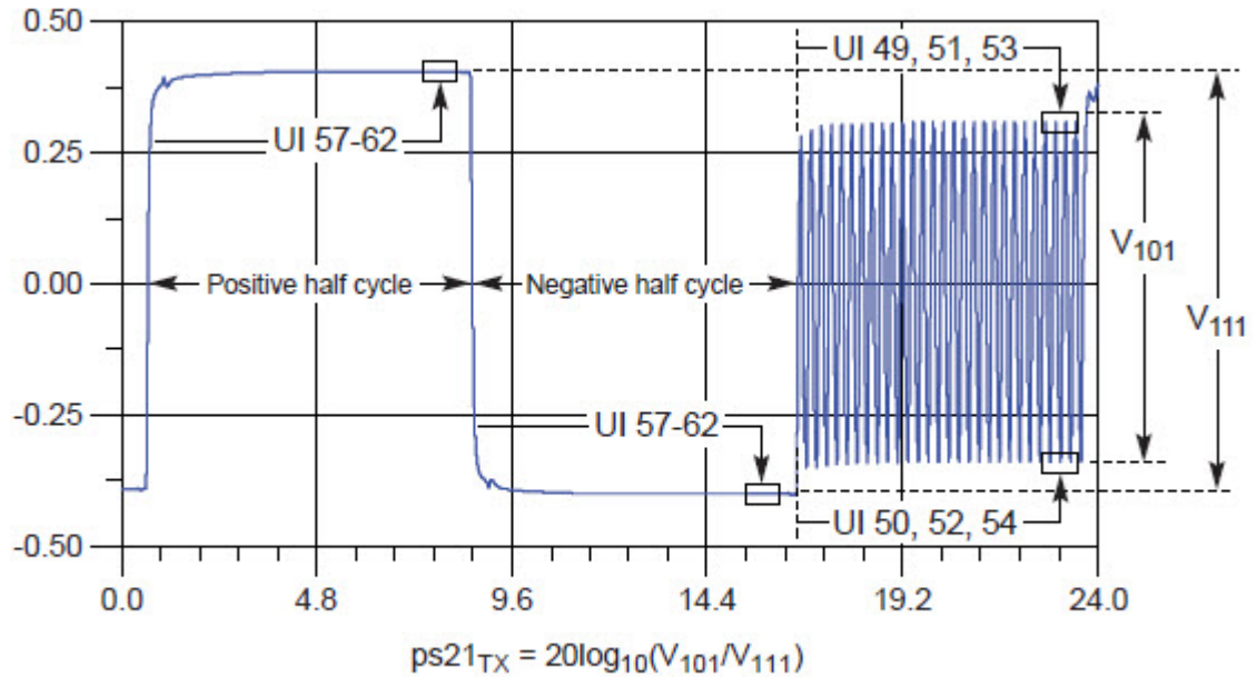
Figure 50 Compliance Pattern and Resulting Package Loss Test Waveform
