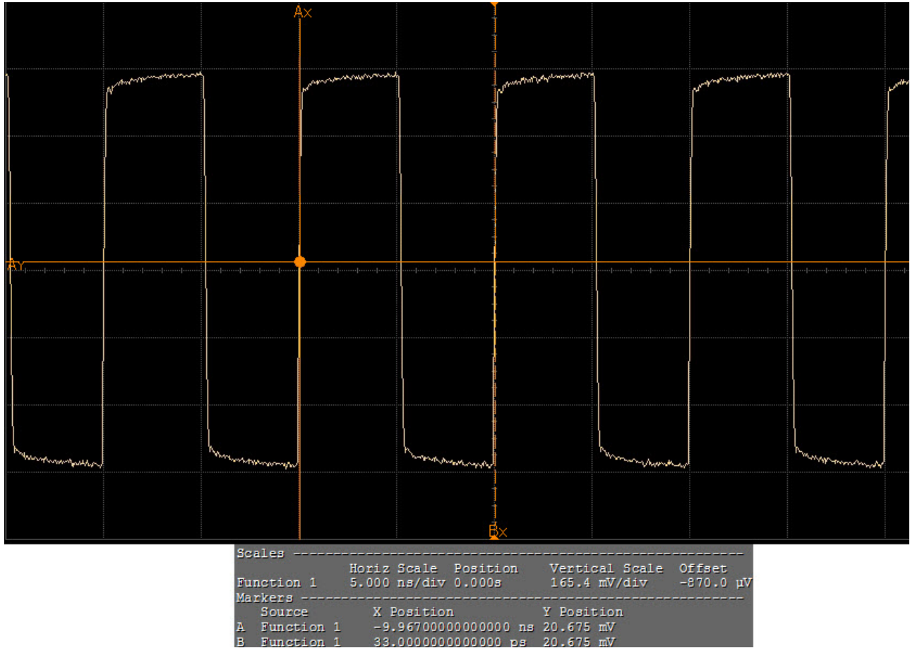
Figure 129 Reference Image for Average Clock Period
