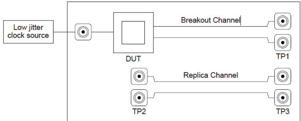
Figure 94 Driver Compliance Test Load
