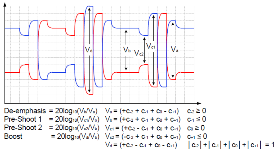
Figure 109 Definition of Tx Voltage Levels and Equalization Ratios
