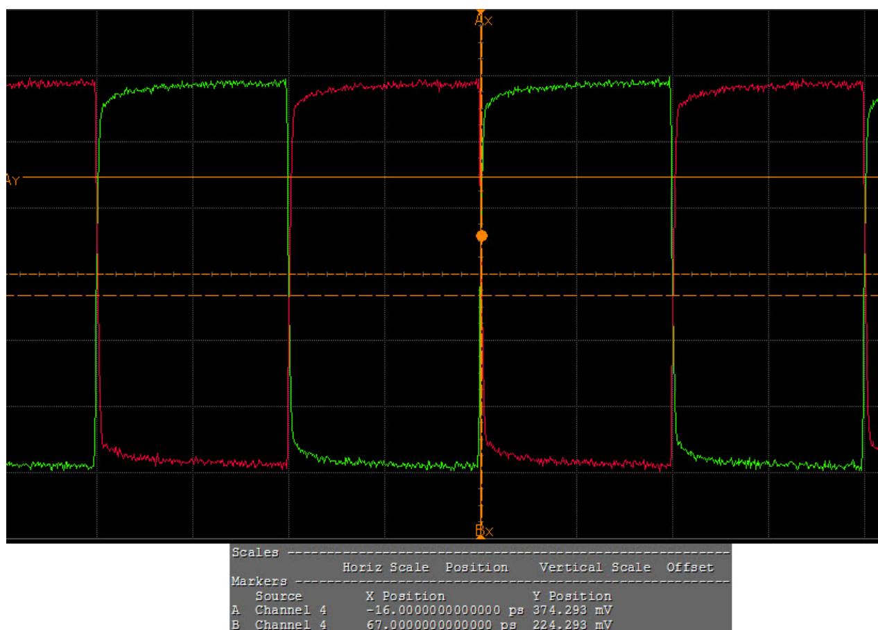
Figure 18 Reference Image for Rise-Fall Matching
