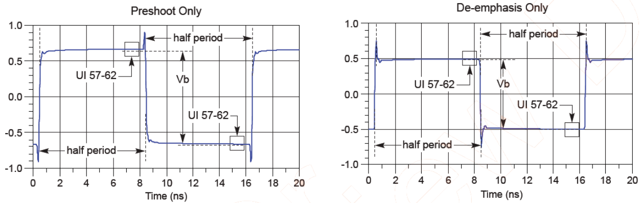
Figure 195 Waveform measurement points for preshoot and de-emphasis
