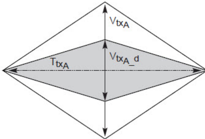
Figure 118 Add-in Card Transmitter Path Compliance Eye Diagram
