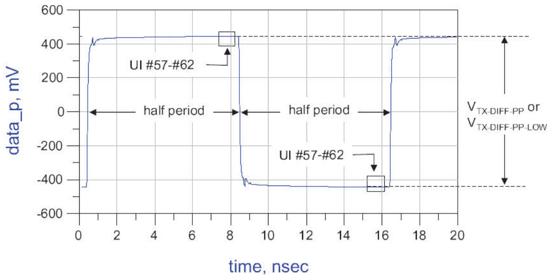
Figure 48 V_{TX-FS-NO-EQ} Measurement
