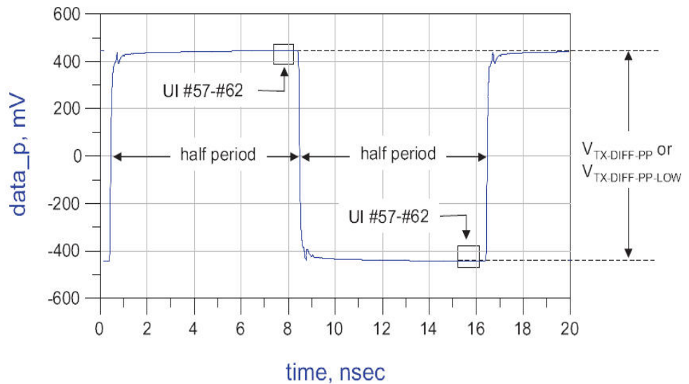
Figure 4 V_{TX-DIFF-PP-LOW} Measurement
