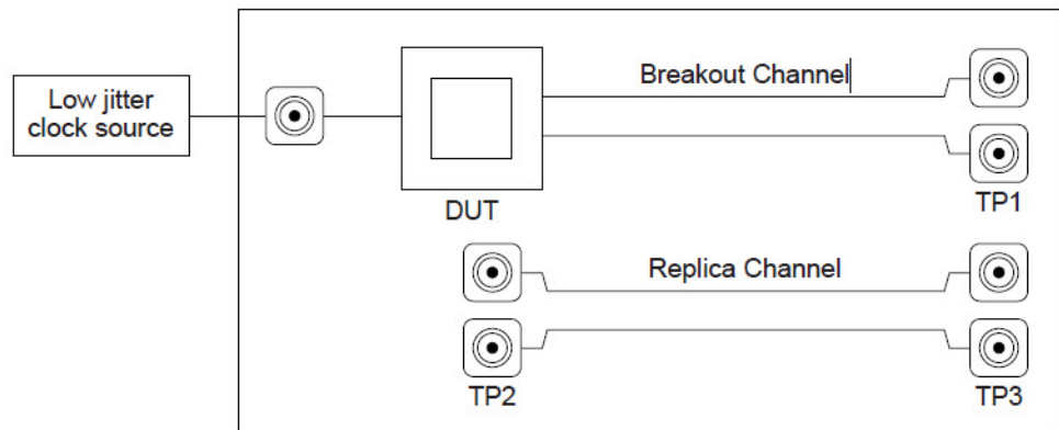
Figure 32 Driver Compliance Test Load
