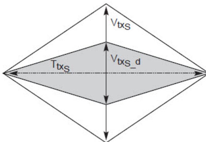
Figure 76 System Board Transmitter Path Composite Compliance Eye Diagram
