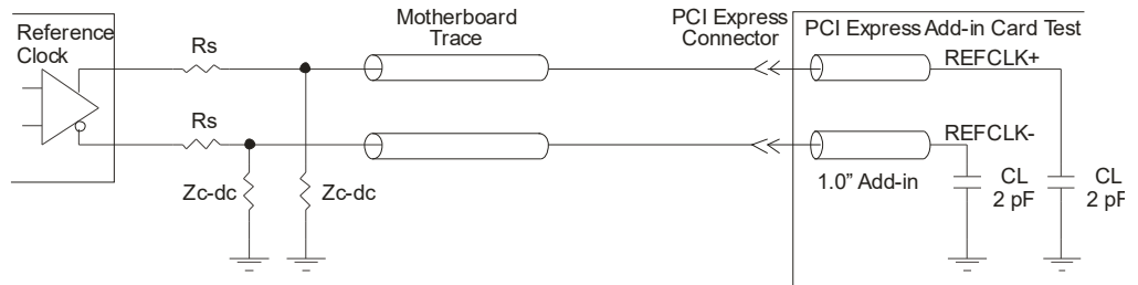
Figure 130 Driver Compliance Test Load
