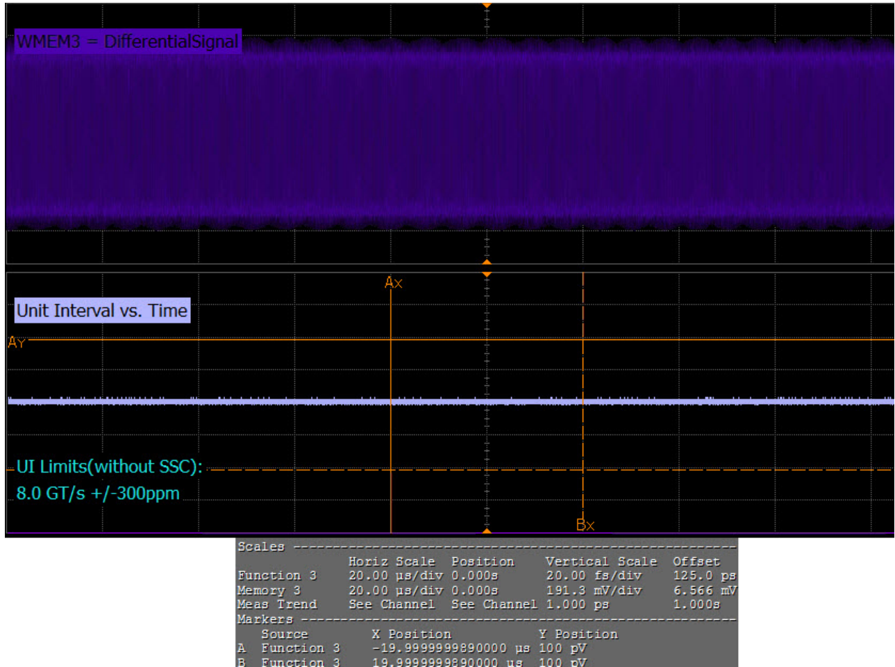
Figure 47 Reference Image for Unit Interval Test
