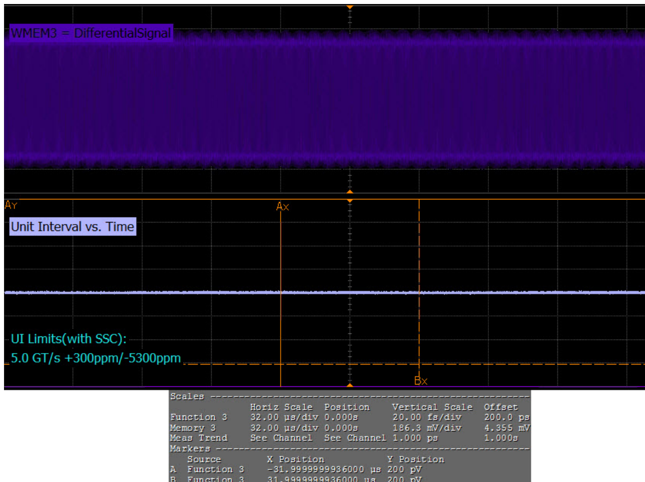
Figure 60 Reference Image for Unit Interval Test
