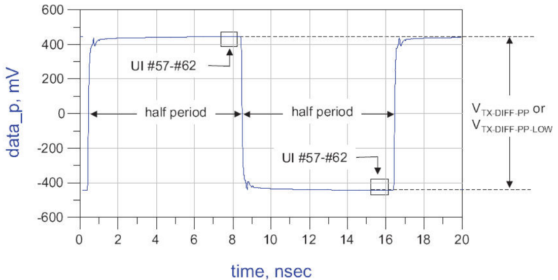
Figure 49 V_{TX-FS-NO-EQ} Measurement
