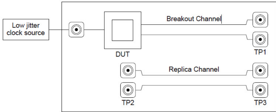
Figure 138 Driver Compliance Test Load
