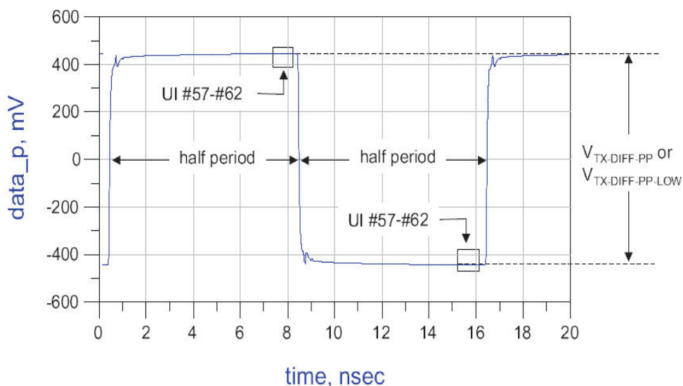
Figure 141 V_{TX-DIFF-PP} Measurement
