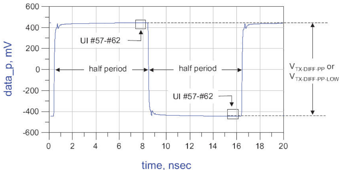
Figure 87 V_{TX-FS-NO-EQ} Measurement
