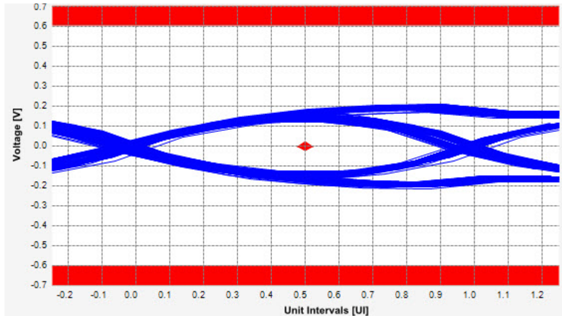
Figure 117 Reference Image for Peak Differential Output Voltage Test
