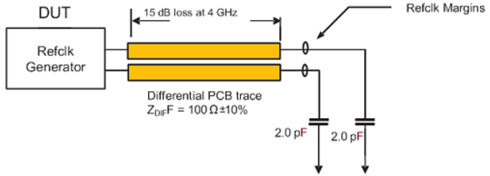
Figure 89 Driver Compliance Test Load
