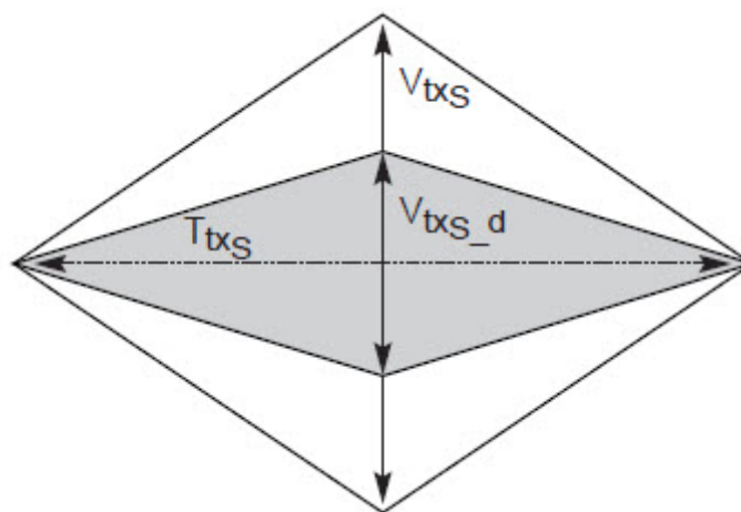
Figure 129 System Board Transmitter Path Composite Compliance Eye Diagram
