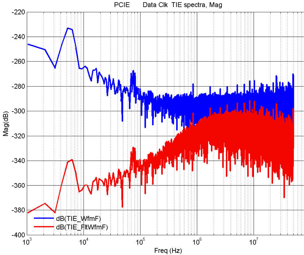
Figure 77 Reference Image for Data Clock TIE Spectra RMS Jitter Test
