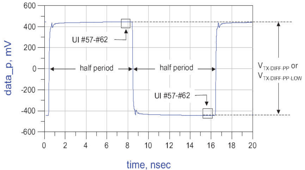
Figure 82 V_{TX-DIFF-PP} Measurement
