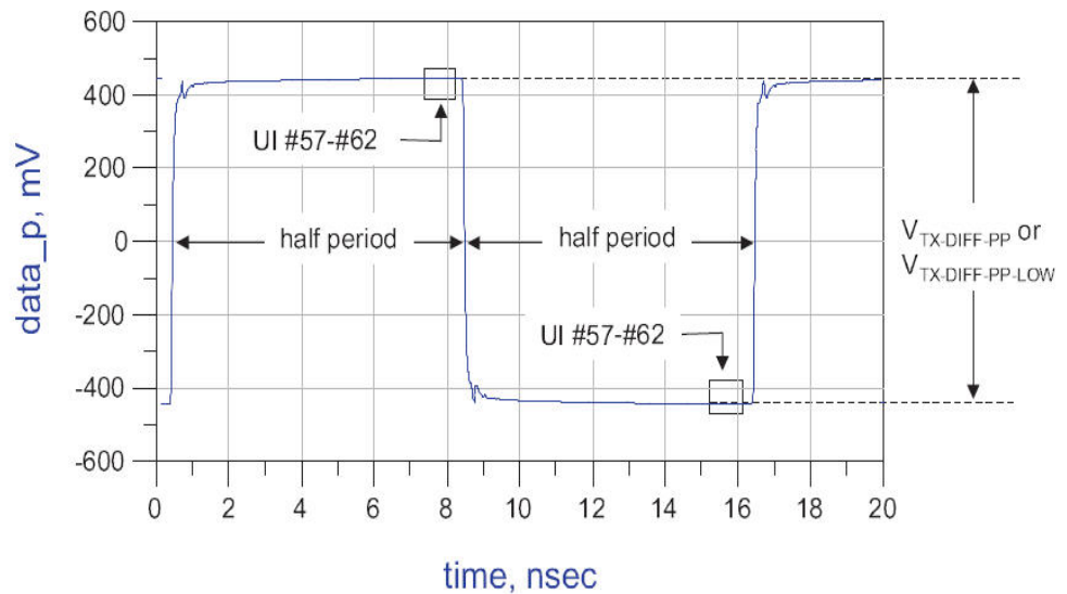
Figure 83 V_{TX-DIFF-PP-LOW} Measurement
