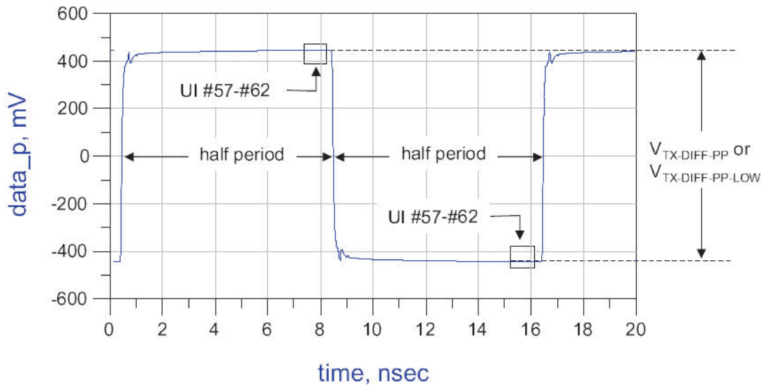
Figure 88 V_{TX-FS-NO-EQ} Measurement
