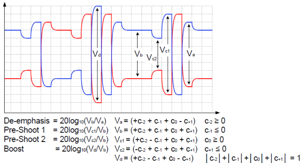
Figure 107 Definition of Tx Voltage Levels and Equalization Ratios
