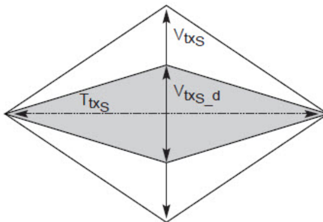
Figure 47 System Board Transmitter Path Composite Compliance Eye Diagram
