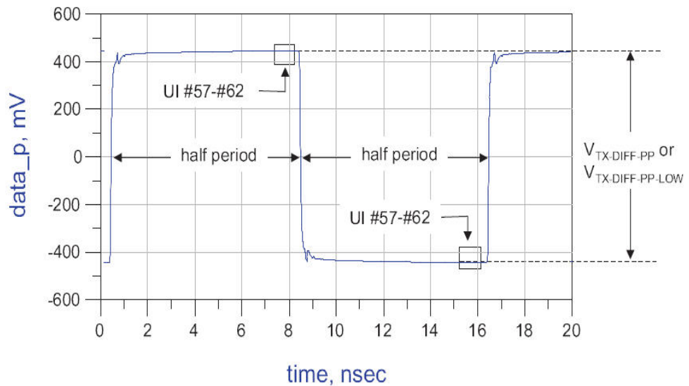
Figure 177 V_{TX-DIFF-PP-LOW} Measurement
