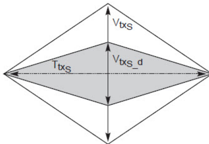
Figure 45 System Board Transmitter Path Composite Compliance Eye Diagram
