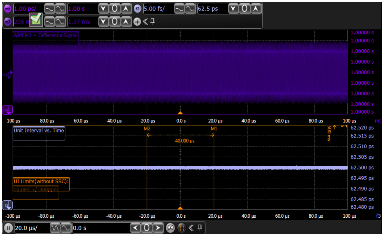
Figure 157 Reference Image for Unit Interval Test
