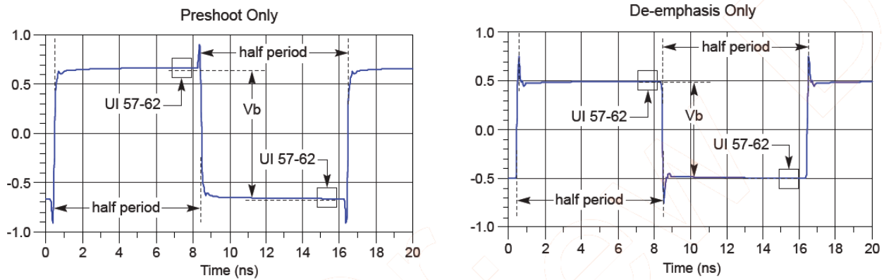
Figure 200 Waveform measurement points for preshoot and de-emphasis
