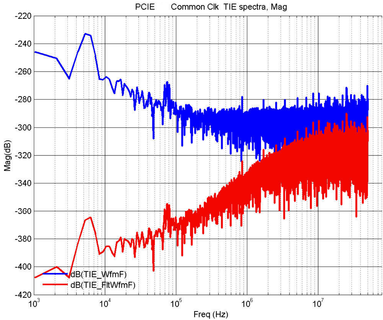
Figure 30 Reference Image for Common Clock TIE Spectra RMS Jitter Test
