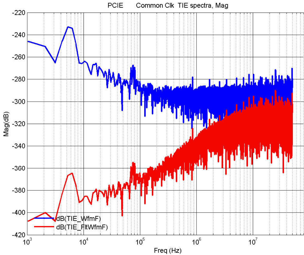
Figure 74 Reference Image for Common Clock TIE Spectra RMS Jitter Test
