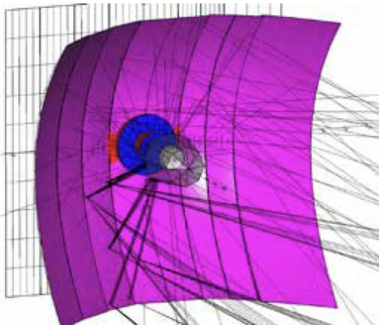
Figure 1. Headlamp and faceted reflector modeled in LucidShape
