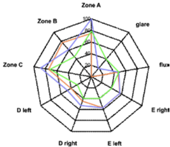
Figure 7. Vehicle headlamp benchmark with CIE TC4-45 assessments
