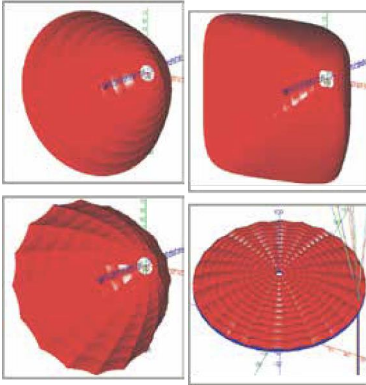
Figure 3. Procedural surfaces for reflector and lens design
