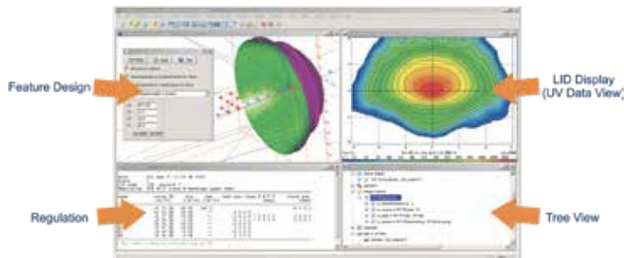
Figure 5. Lighting design in LucidShape with simulation result and photometric test table
