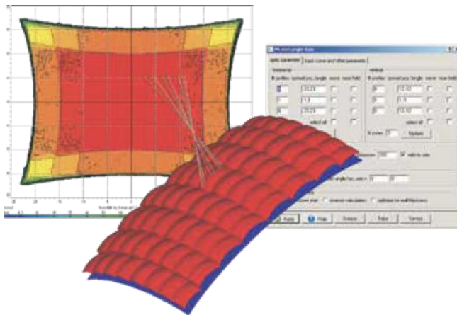
Figure 2. Tail lamp with pillow optic lens
