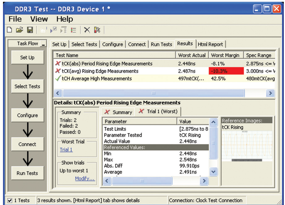
Figure 7. The DDR3 and LPDDR3 test application documents your test parameters, pass or fail status, test specification range, measured values and the pass/fail margin.
