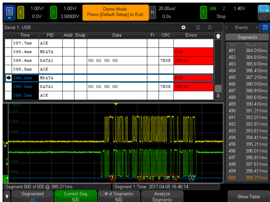
Figure 93 Using the scope's Segmented Memory acquisition to selectively capture more USB traffic.
