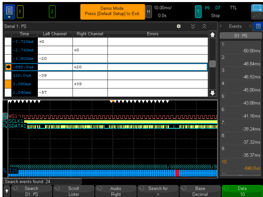
Figure 82 Automatic Search & Navigation on I 2 S data.
