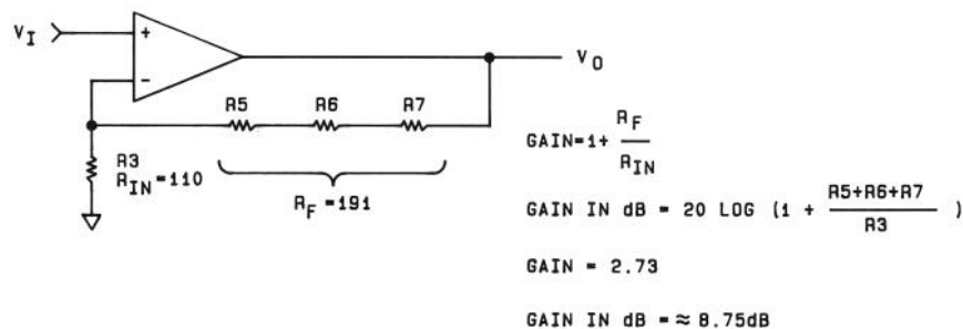
FIGURE 8-34. 10 dB INPUT BUFFER AMPLIFIER GAIN MODEL
