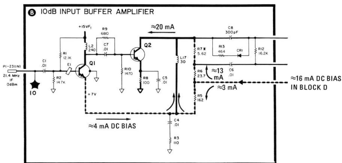
FIGURE 8-35. DC BIAS PATH DURING CRYSTAL POLE OPERATION
