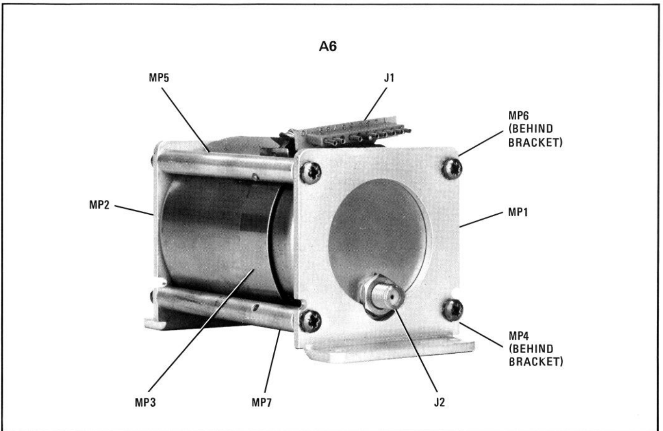
FIGURE 8-22. A6 YIG OSCILLATOR
