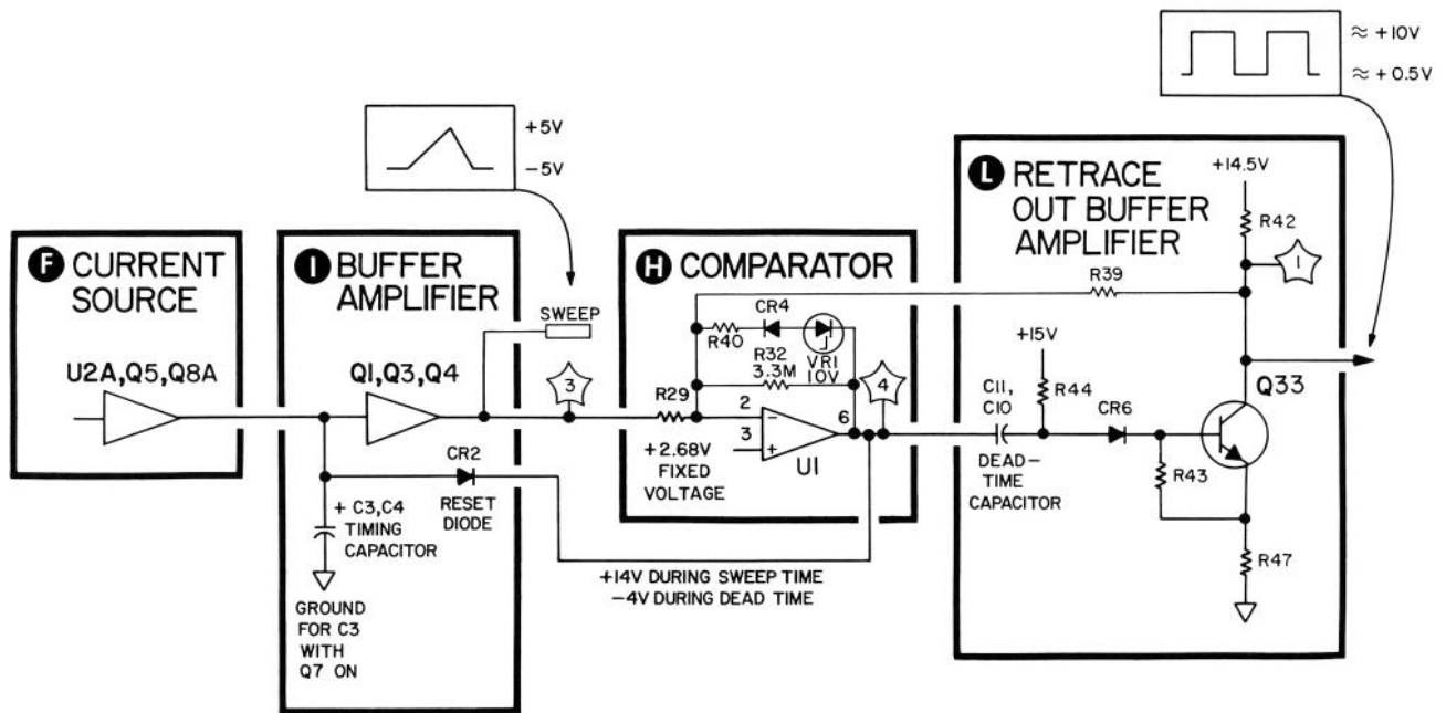
FIGURE 8-28. SIMPLIFIED SCHEMATIC OF SWEEP GENERATOR IN AUTO MODE
