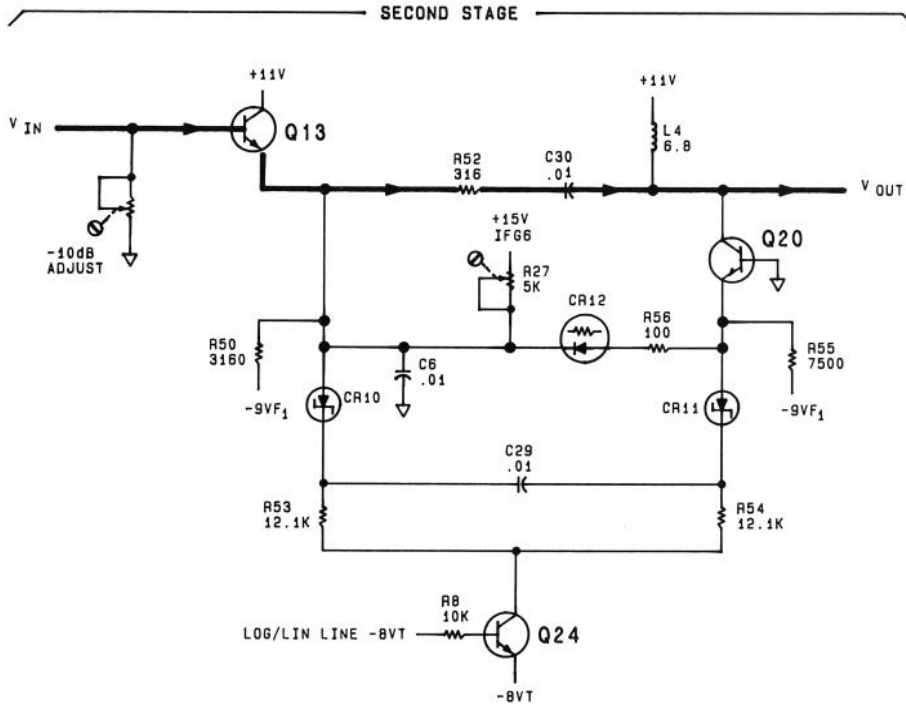
FIGURE 8-51. UNITY GAIN OPERATION IN LINEAR MODE, SIMPLIFIED SCHEMATIC
