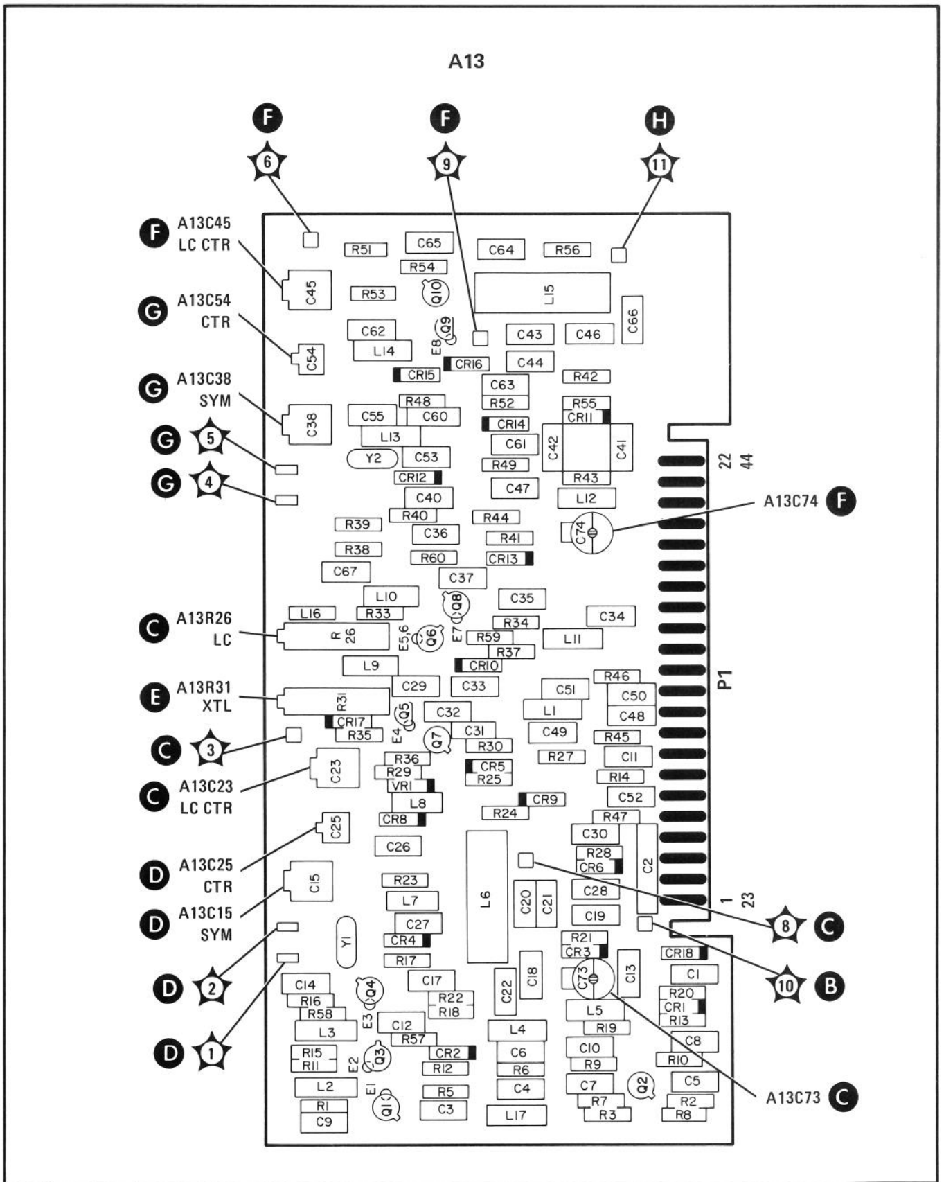
FIGURE 7-20. A13 BANDWIDTH FILTER NO. 2, COMPONENT LOCATIONS (2147A & BELOW)
