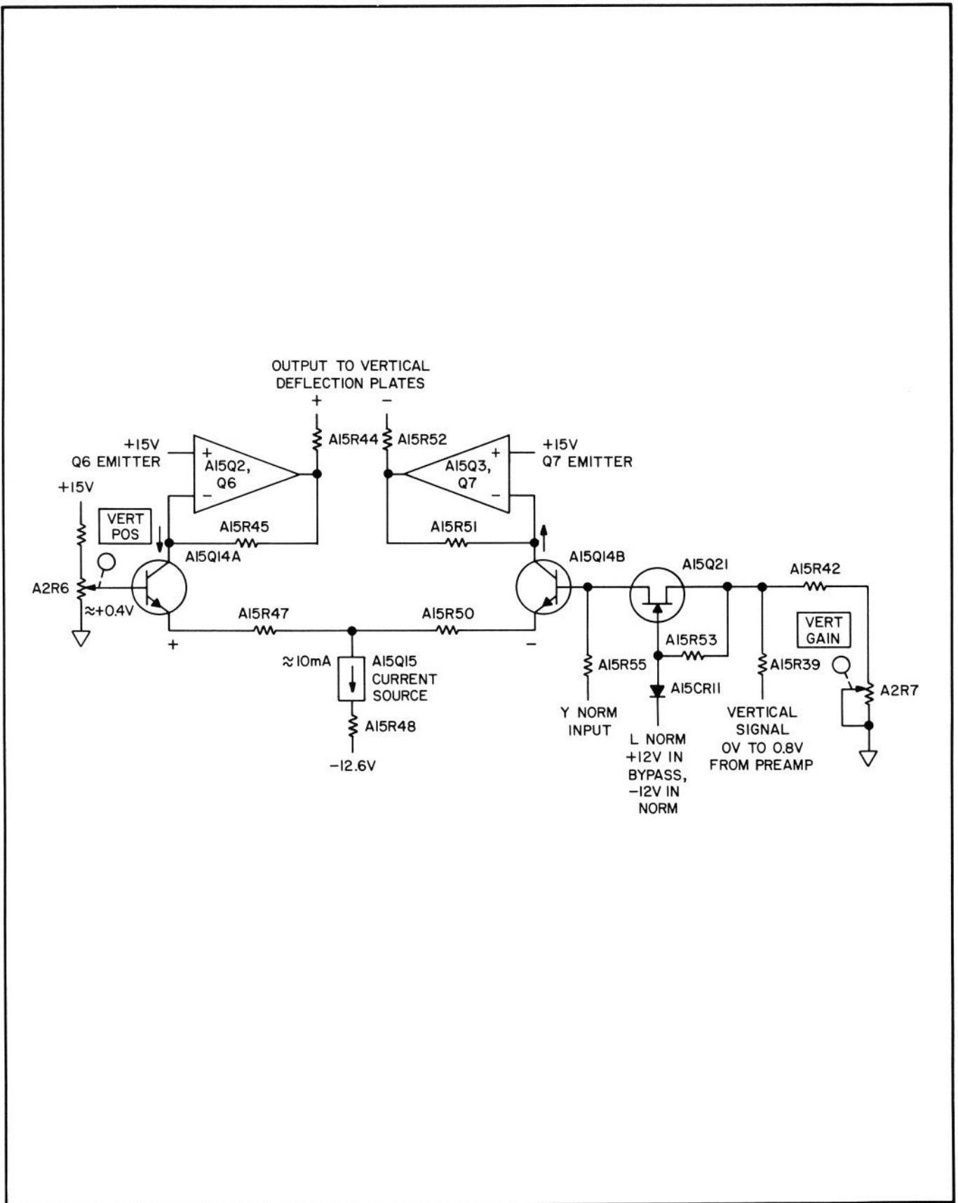
FIGURE 8-55. SIMPLIFIED VERTICAL DRIVER CIRCUIT
