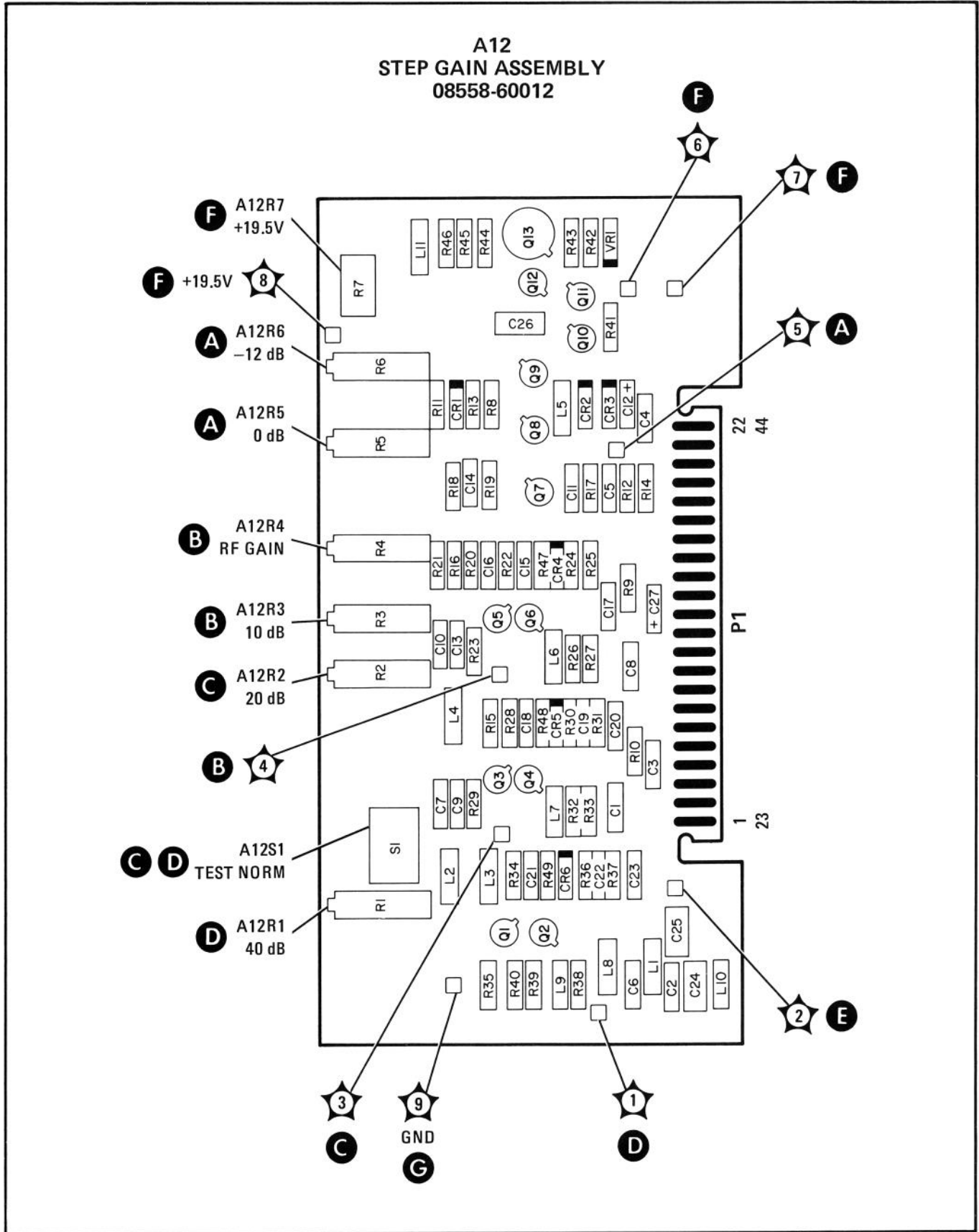
FIGURE 8-46. A12 STEP GAIN ASSEMBLY, COMPONENT LOCATIONS
