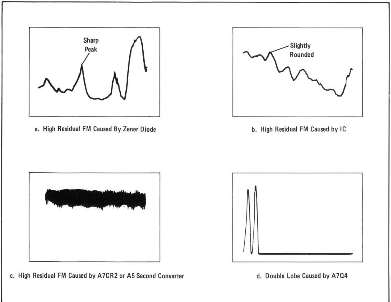
FIGURE 8-3. CRT DISPLAYS FOR RESIDUAL FM TROUBLESHOOTING
