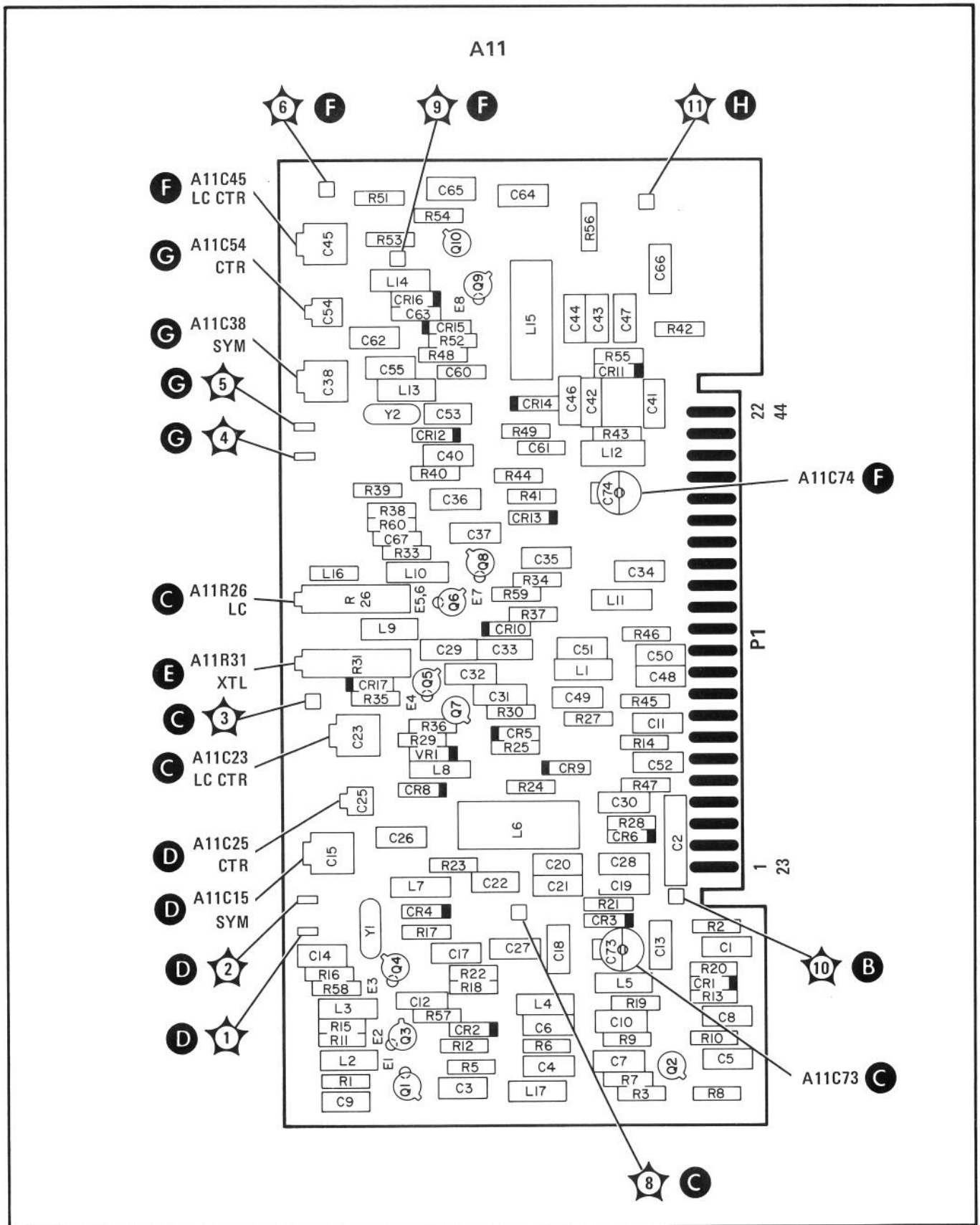
FIGURE 7-18. A11 BANDWIDTH FILTER NO. 1, COMPONENT AND TEST POINT LOCATIONS (2147A & BELOW)
