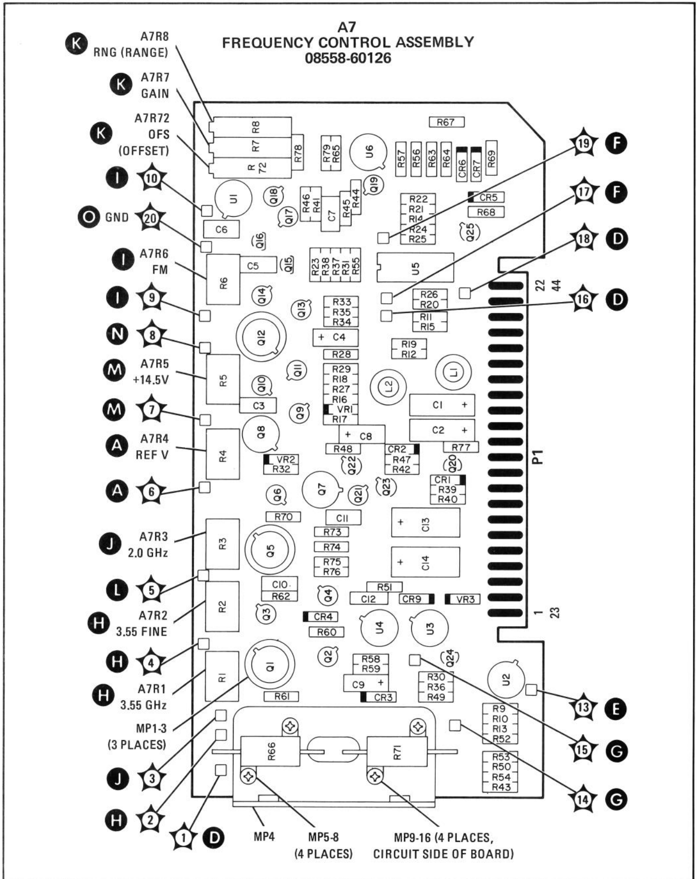
FIGURE 8-26. A7 FREQUENCY CONTROL ASSEMBLY, COMPONENT LOCATIONS
