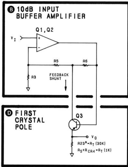
FIGURE 8-37. 10 dB INPUT BUFFER AMPLIFIER DURING CRYSTAL FILTER OPERATION
