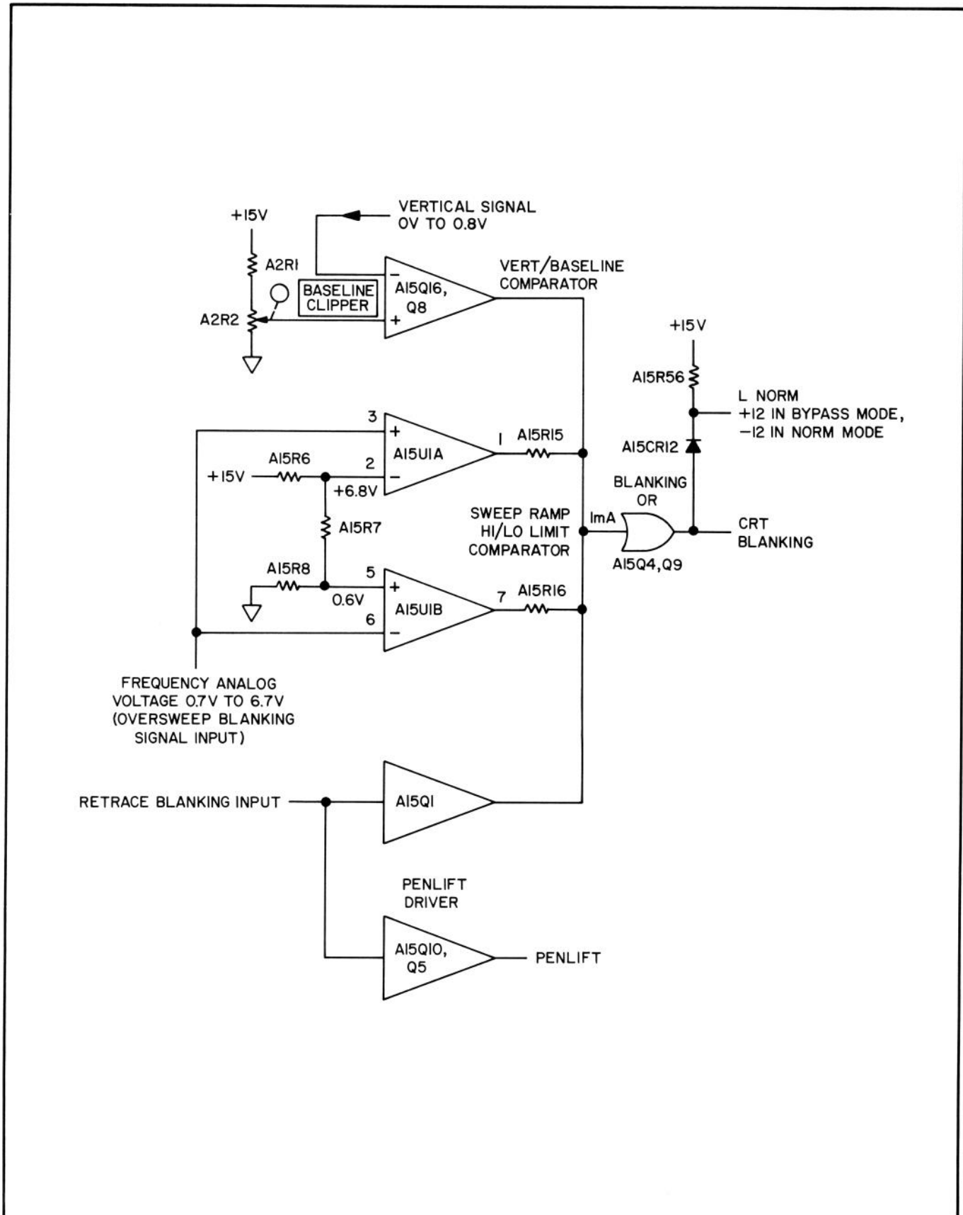
FIGURE 8-56. SIMPLIFIED BLANKING CIRCUIT
