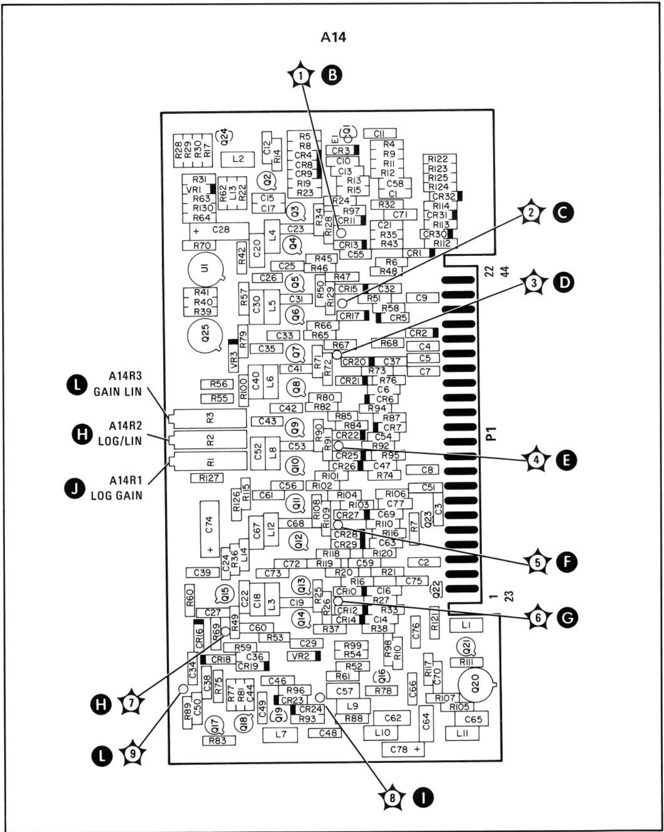
FIGURE 7-5. A14 LOG AMPLIFIER, COMPONENT AND TEST POINT LOCATIONS (2142A & BELOW)
