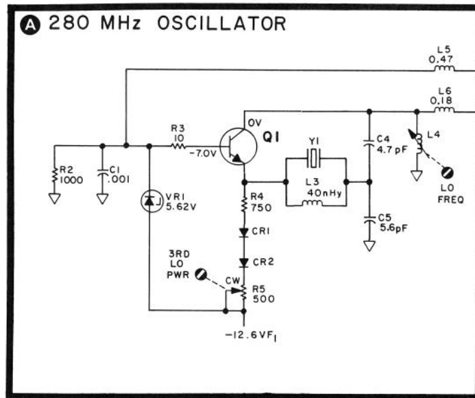
FIGURE 7-8. P/O A9 THIRD CONVERTER AND A10 SECOND IF ASSEMBLIES, SCHEMATIC DIAGRAM (2118A & BELOW)
