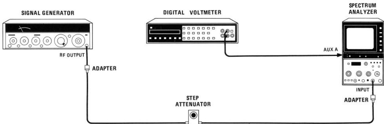
FIGURE 4-19. AMPLITUDE LOG DISPLAY ACCURACY TEST SETUP
