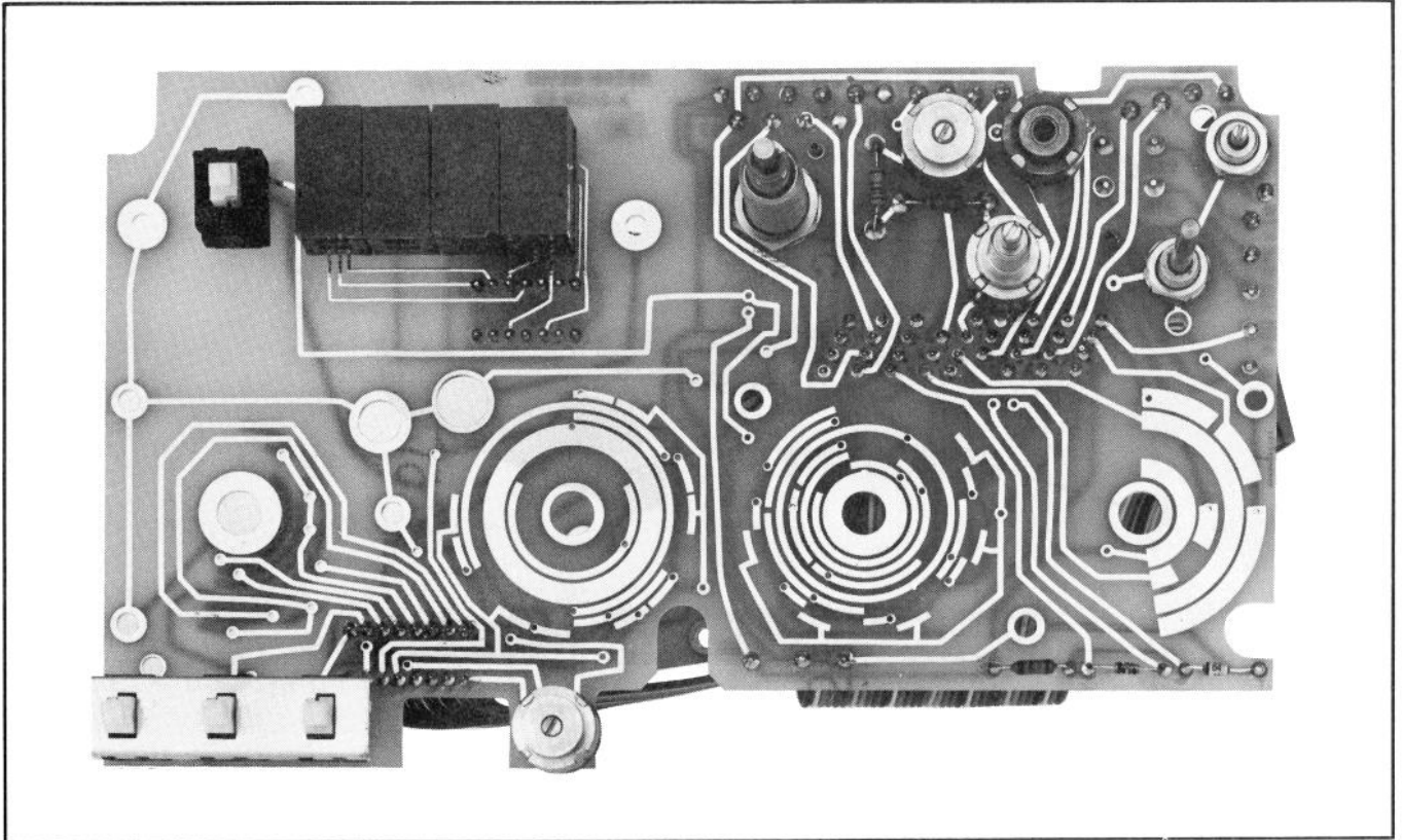
FIGURE 8-16. FRONT VIEW OF SWITCHBOARD ASSEMBLY A2A1
