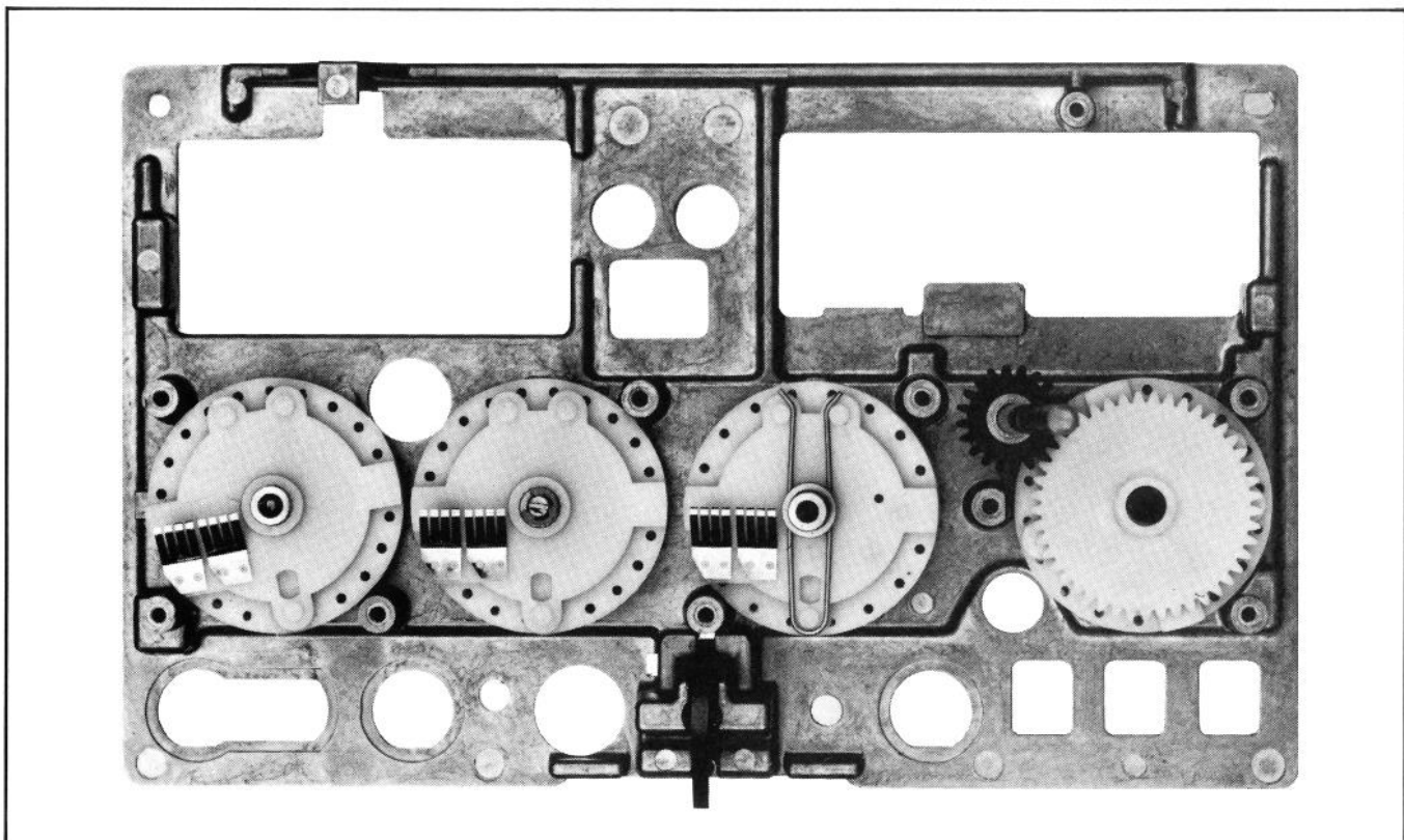
FIGURE 8-15. PROPER POSITIONING OF ROTORS ON FRONT SWITCH DIECAST
