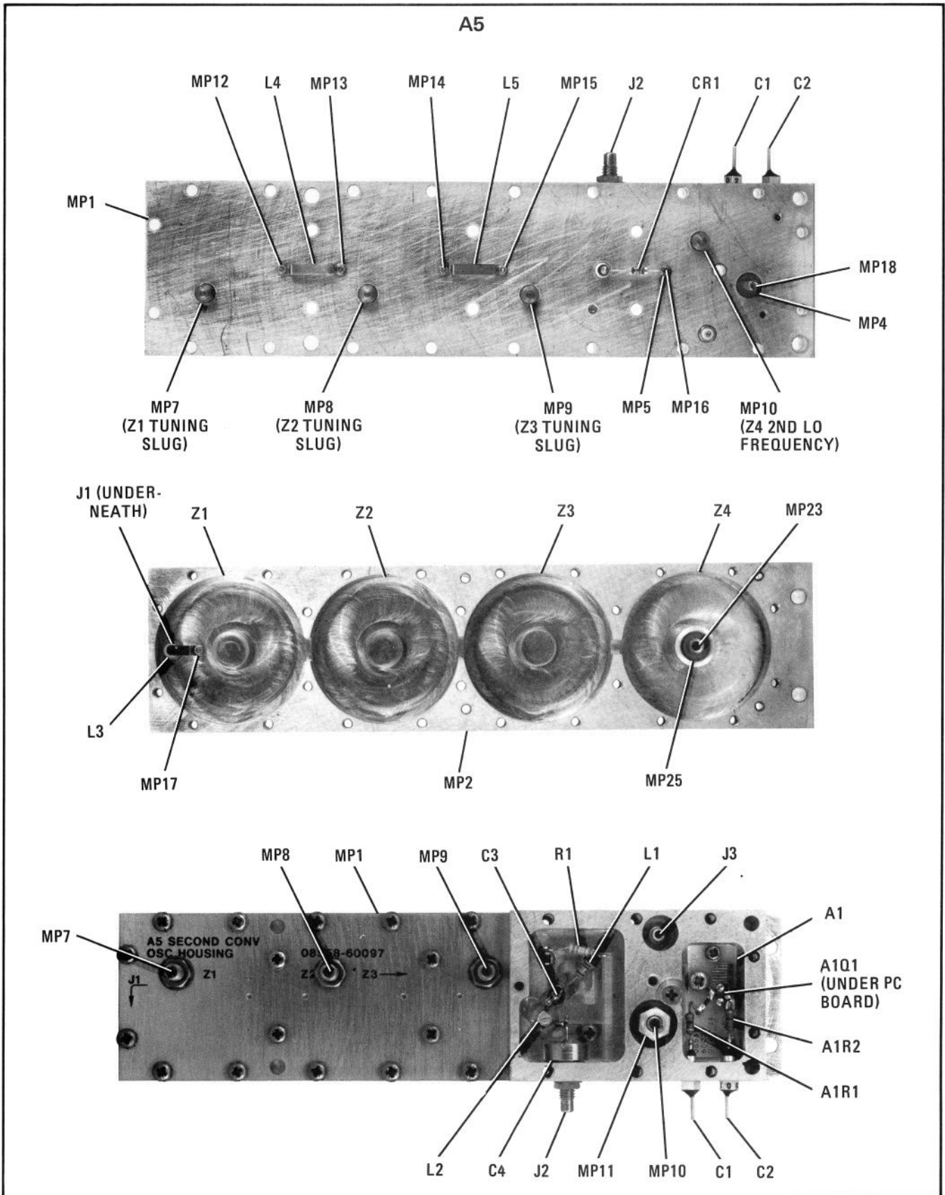
FIGURE 8-24. A5 SECOND CONVERTER ASSEMBLY, COMPONENT LOCATIONS
