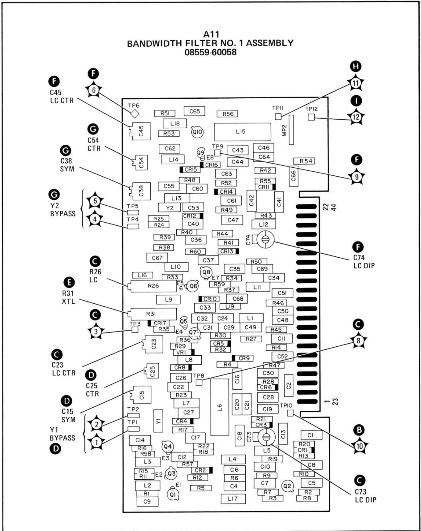
FIGURE 8-43. A11 BANDWIDTH FILTER NO. 1, COMPONENT LOCATIONS
