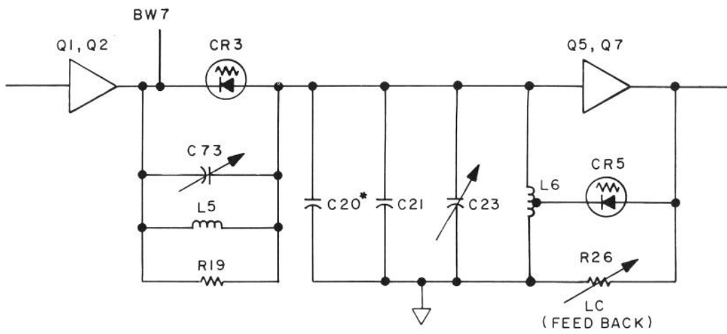
FIGURE 7-17. LC POLE, SIMPLIFIED SCHEMATIC (2147A & BELOW)
