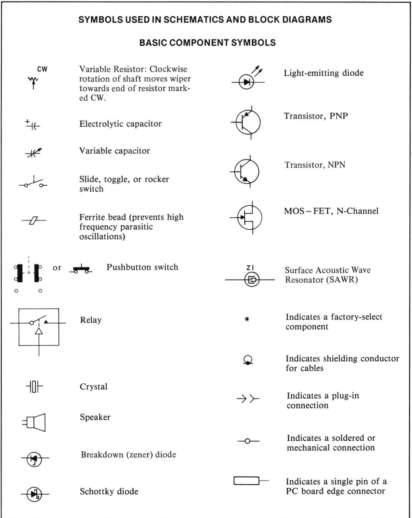
FIGURE 8-1. SYMBOLS USED IN SCHEMATICS AND BLOCK DIAGRAMS (1 OF 4)
