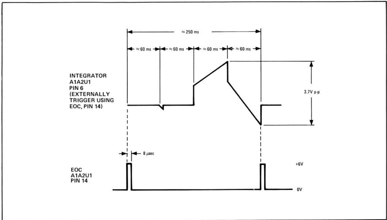
FIGURE 8-8. INTEGRATOR AND EOC WAVEFORMS FOR FREQUENCY MHz DISPLAY OF 1296 MHz
