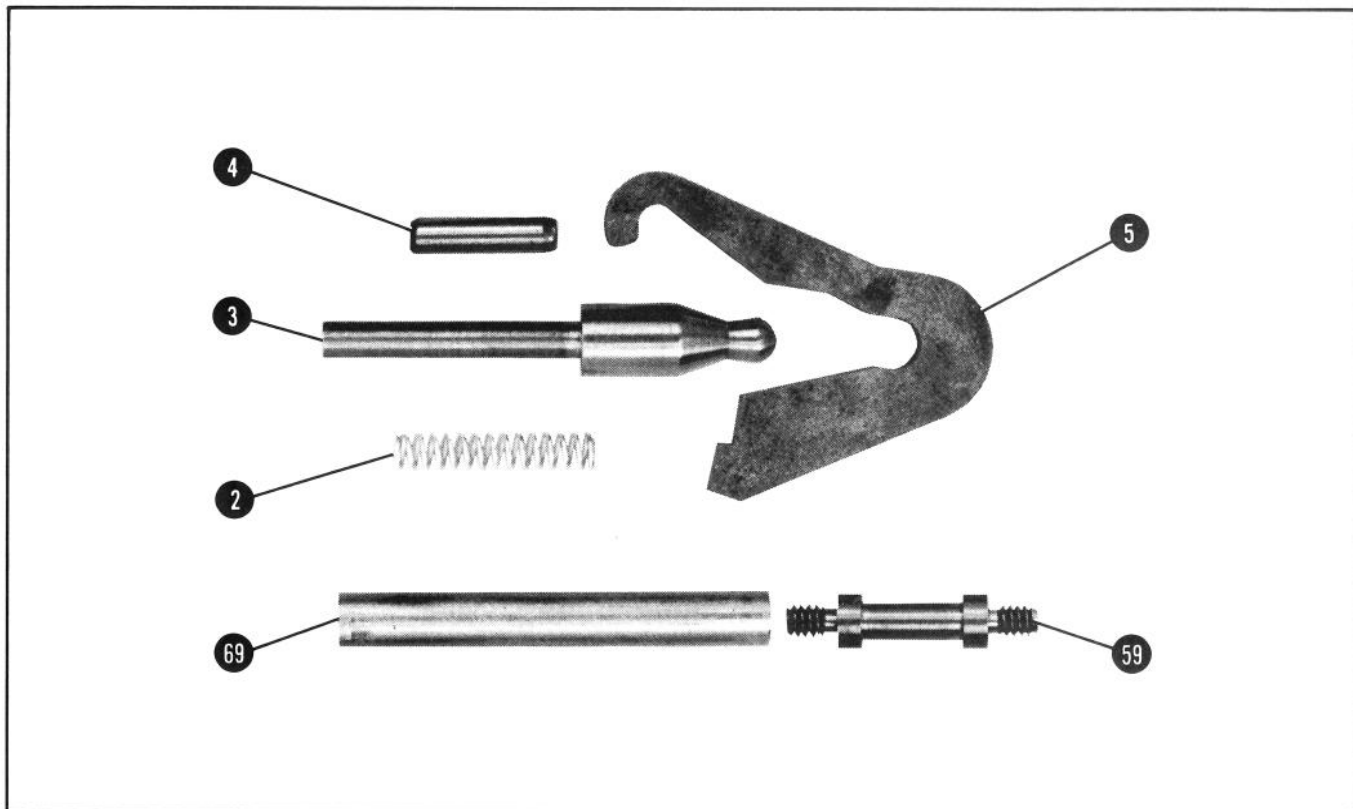
FIGURE 8-14. MACHINED PARTS
