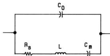
FIGURE 8-38. CRYSTAL MODEL
