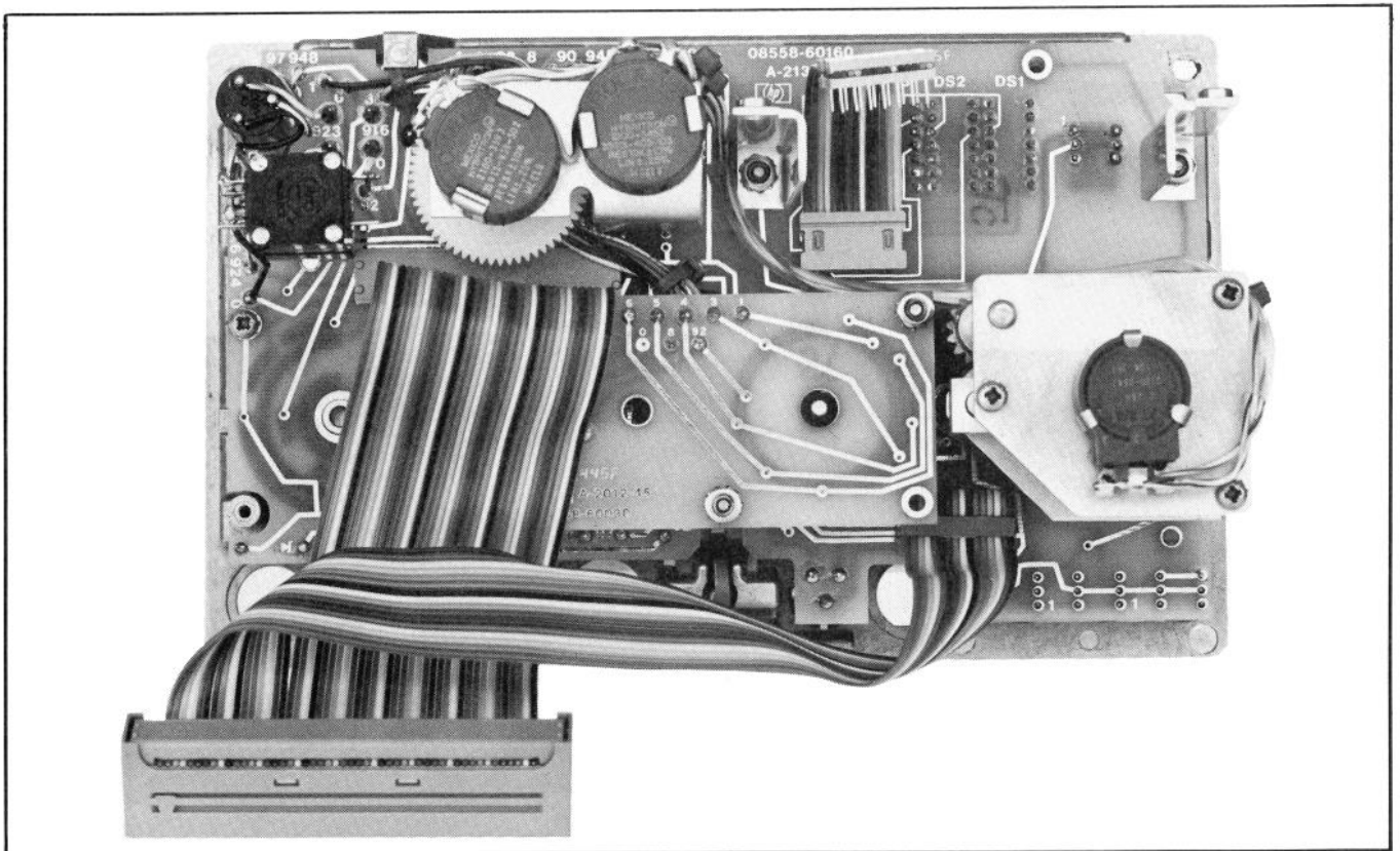
FIGURE 8-17. REAR VIEW OF FRONT SWITCH ASSEMBLY A2
