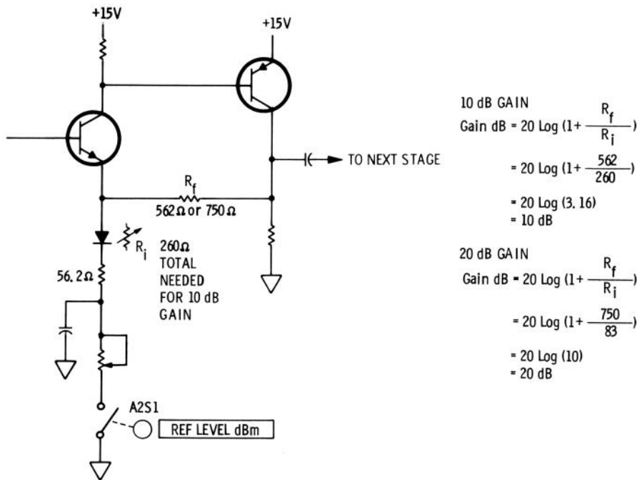
FIGURE 8-45. EQUIVALENT CIRCUIT FOR STEP GAIN AMPLIFIERS
