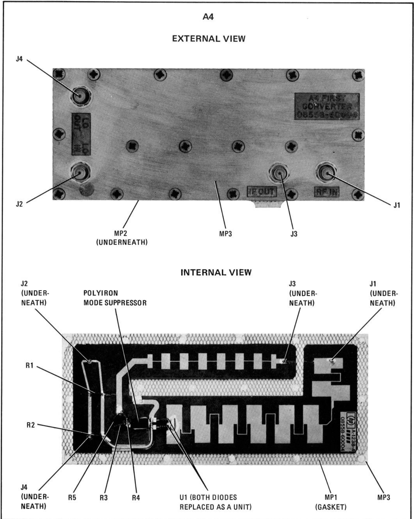
FIGURE 8-23. A4 FIRST CONVERTER ASSEMBLY, COMPONENT LOCATIONS
