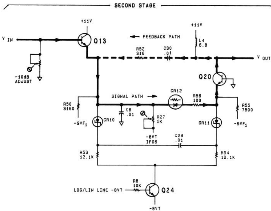
FIGURE 8-52. 10 dB GAIN OPERATION IN LINEAR MODE, SIMPLIFIED SCHEMATIC
