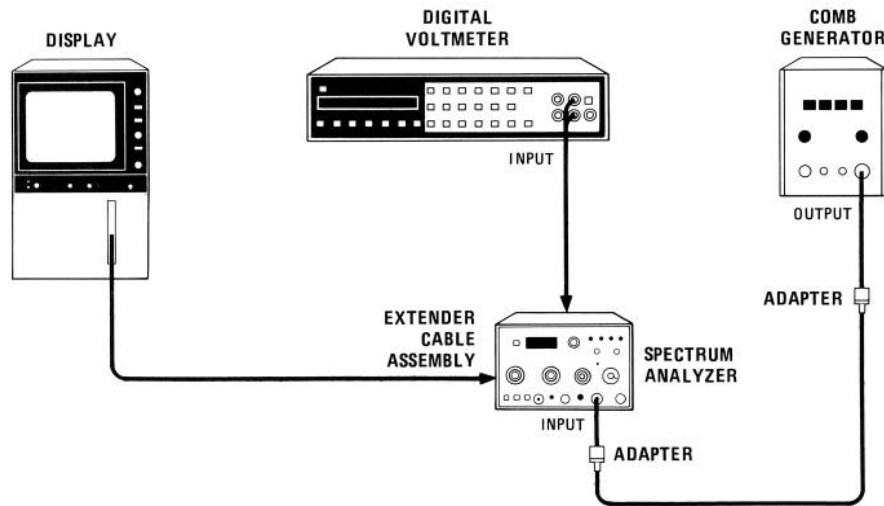
FIGURE 5-15. FREQUENCY CONTROL AND DPM ADJUSTMENTS TEST SETUP
