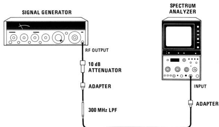
FIGURE 4-13. HARMONIC DISTORTION TEST SETUP
