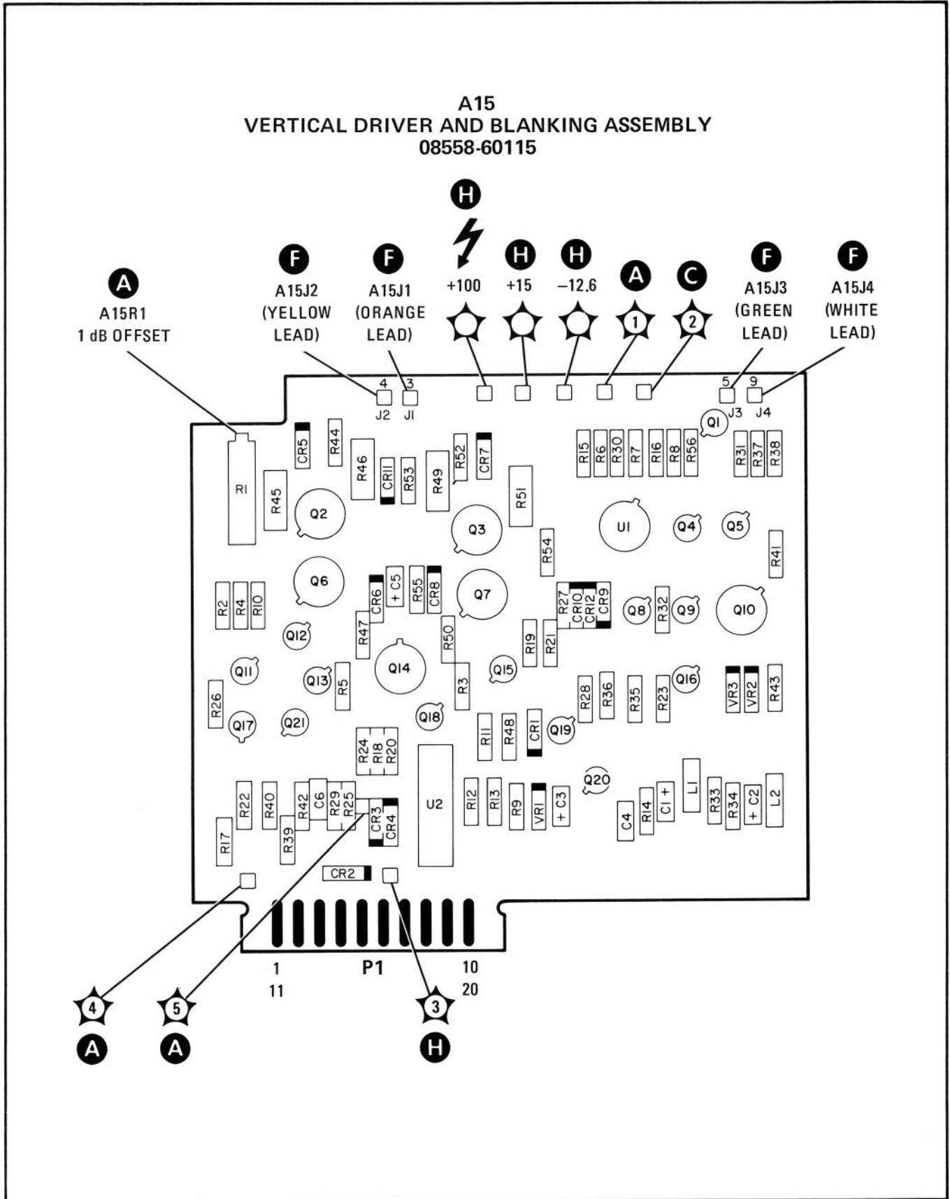
FIGURE 8-57. A15 VERTICAL DRIVER AND BLANKING ASSEMBLY, COMPONENT LOCATIONS
