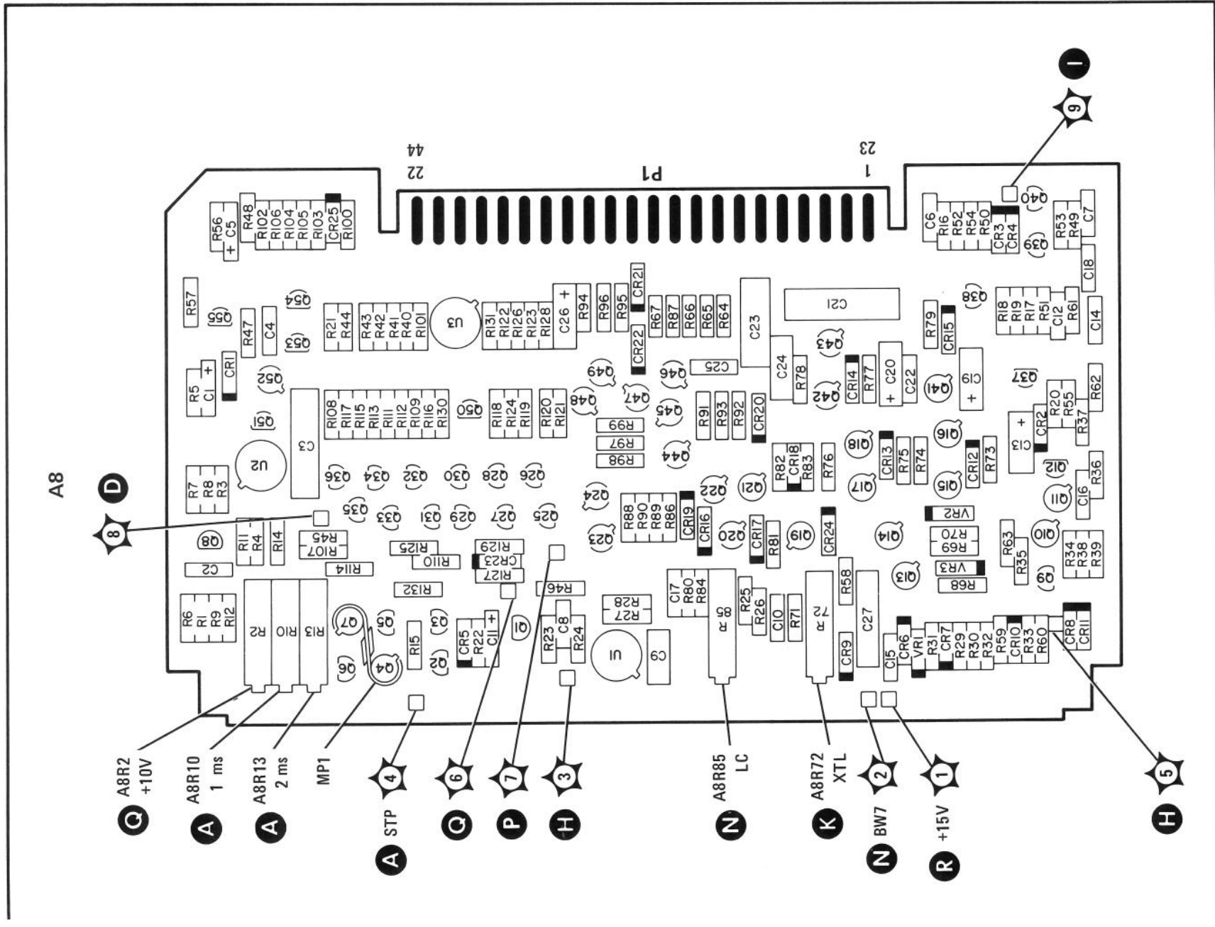
FIGURE 7-15. A8 SWEEP GENERATOR ASSEMBLY, COMPONENT AND TEST POINT LOCATIONS (2215A & BELOW)
