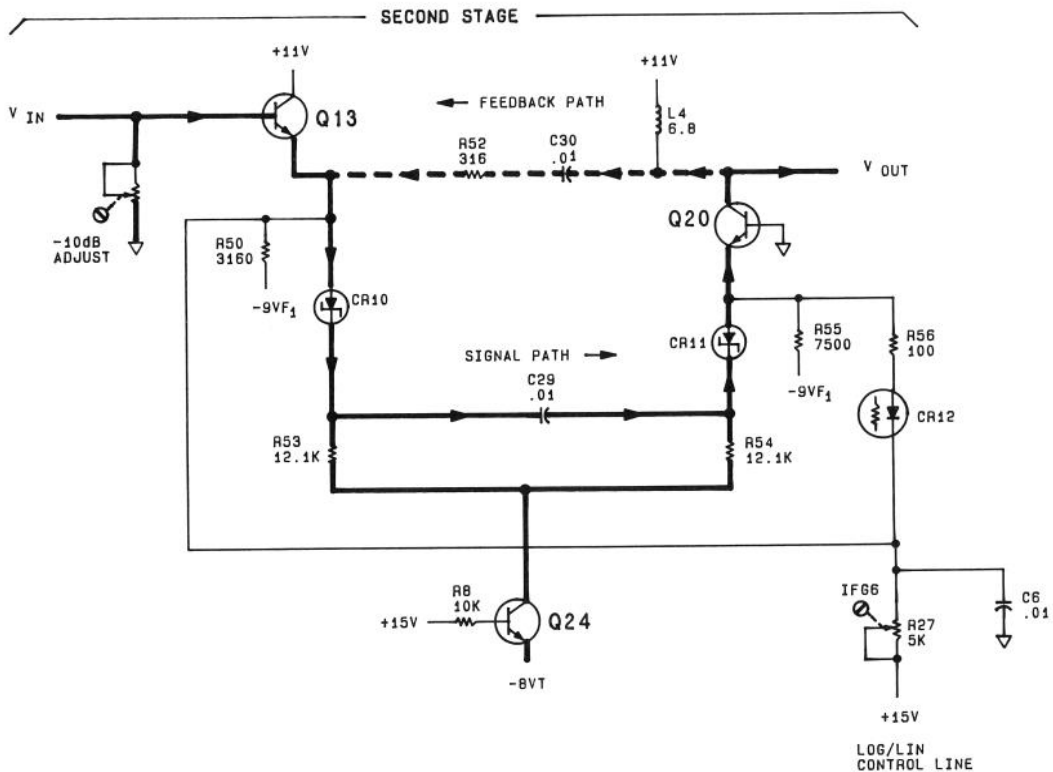
FIGURE 8-50. LOG MODE OPERATION, SIMPLIFIED SCHEMATIC
