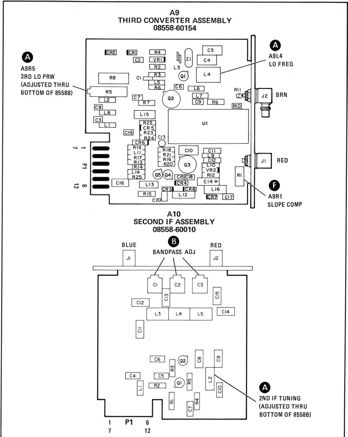
FIGURE 8-32. A9 THIRD CONVERTER AND A10 SECOND IF ASSEMBLIES, COMPONENT LOCATIONS
