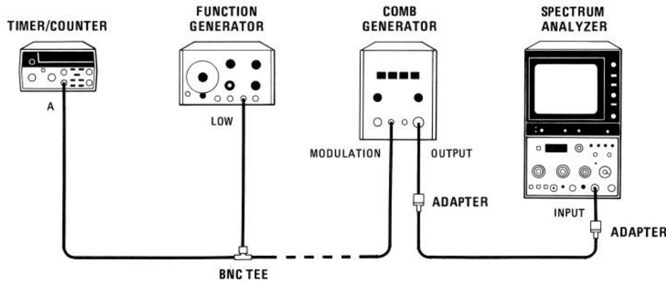
FIGURE 4-1. FREQUENCY SPAN ACCURACY TEST SETUP
