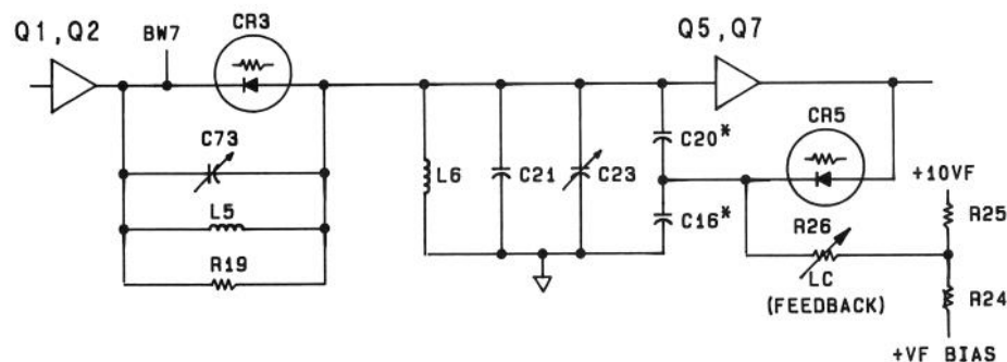
FIGURE 8-42. FIRST LC POLE, SIMPLIFIED SCHEMATIC
