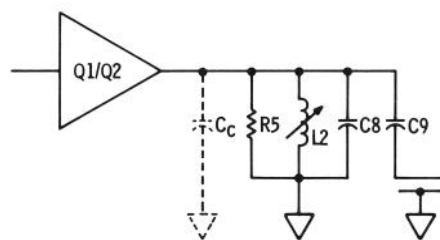
FIGURE 8-31. BANDPASS AMPLIFIER TANK CIRCUIT, SIMPLIFIED SCHEMATIC
