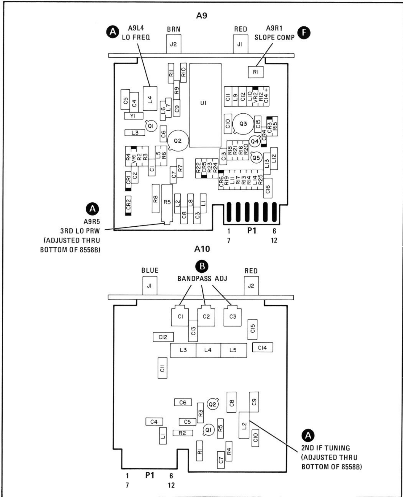
FIGURE 7-9. A9 THIRD CONVERTER AND A10 SECOND IF ASSEMBLIES, COMPONENT LOCATIONS
