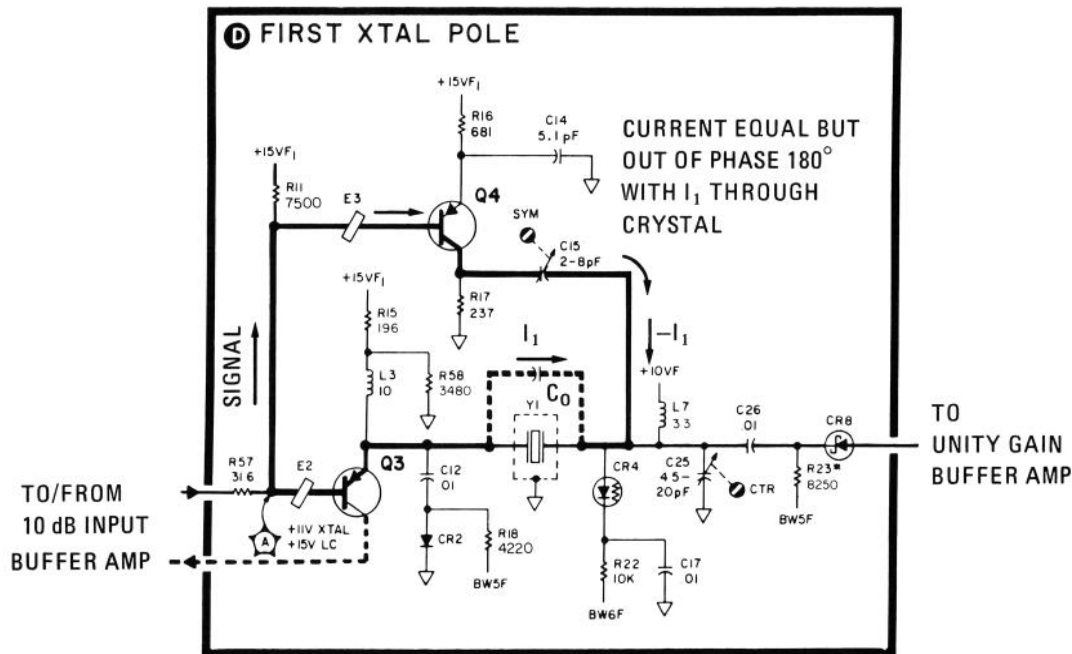
FIGURE 8-40. COMPENSATION AMPLIFIER
