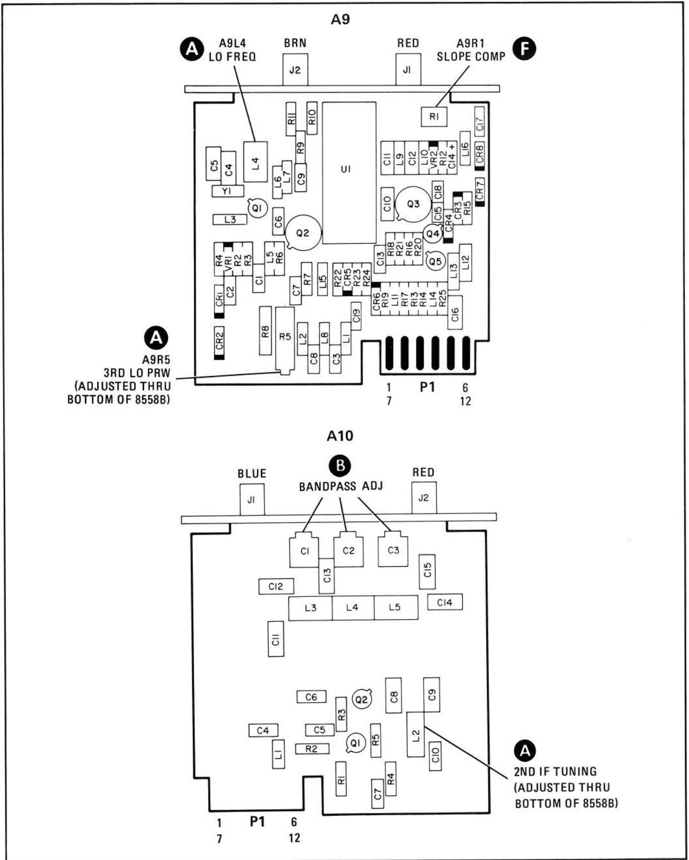
FIGURE 7-7. A9 THIRD CONVERTER AND A10 SECOND IF ASSEMBLIES, COMPONENT LOCATIONS (2118A & BELOW)
