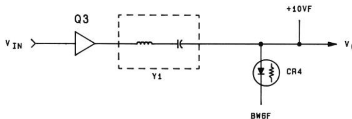
FIGURE 8-39. FIRST CRYSTAL POLE, SIMPLIFIED SCHEMATIC
