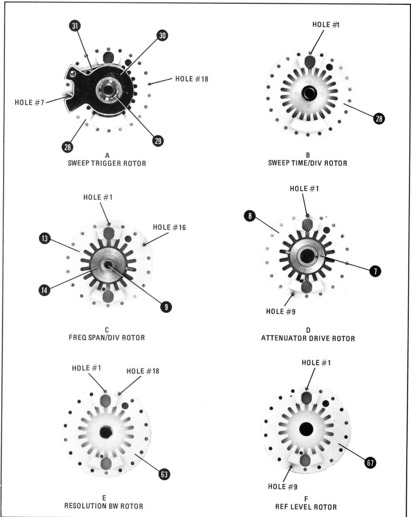
FIGURE 8-13. ROTOR ASSEMBLIES
