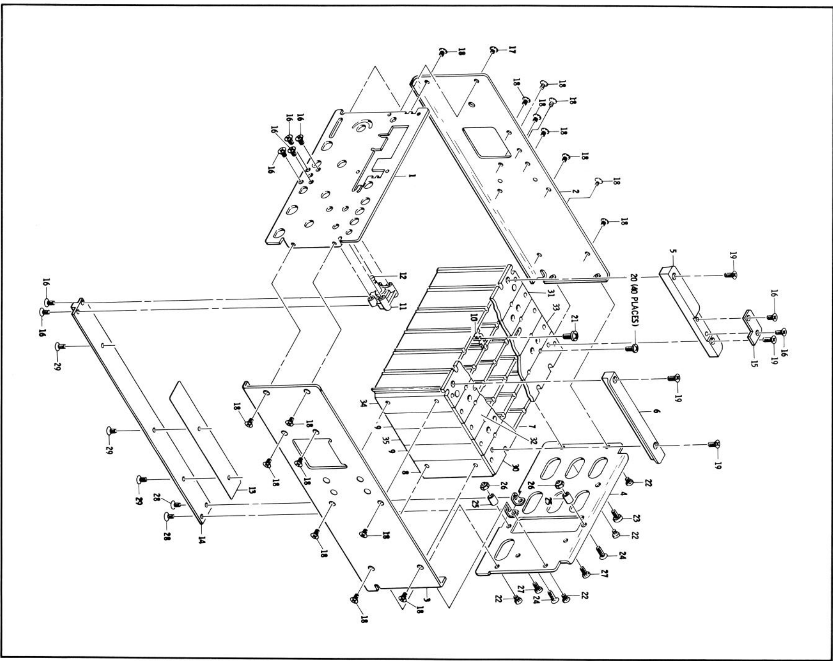
FIGURE 7-1. MECHANICAL CHASSIS PARTS (2 OF 2) (2145A & BELOW)
