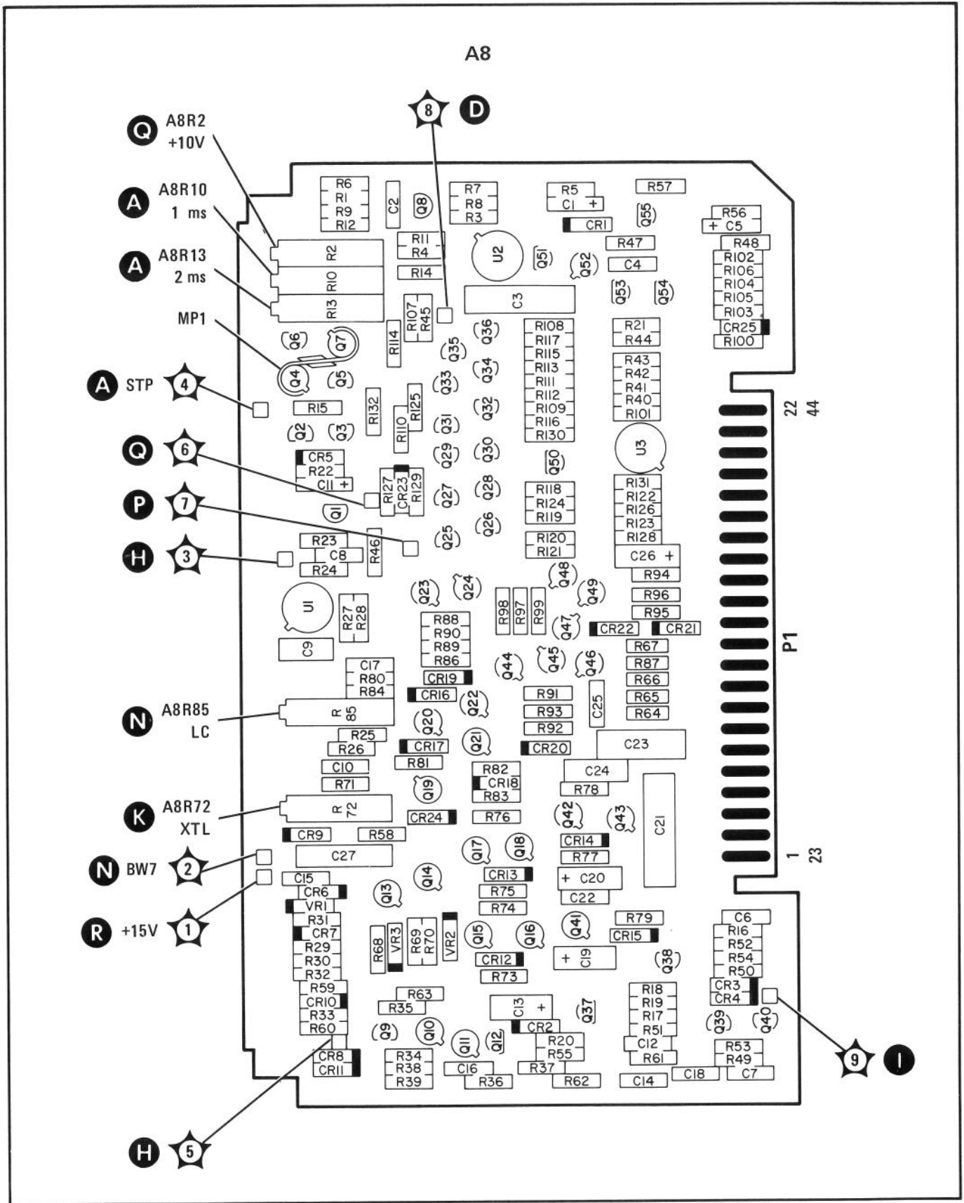
FIGURE 7-15. A8 SWEEP GENERATOR ASSEMBLY, COMPONENT AND TEST POINT LOCATIONS (2215A & BELOW)
