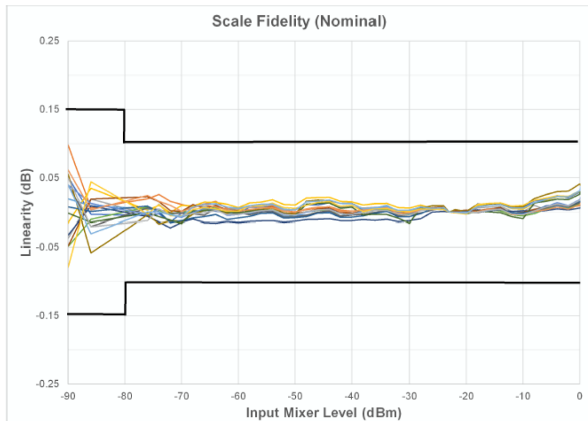
Nominal Display Scale Fidelity [Plot]
