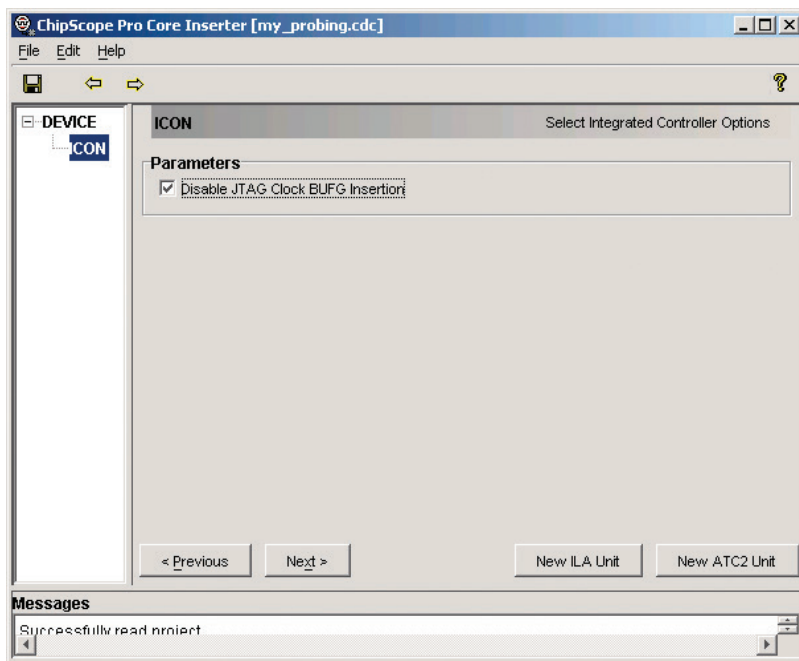
Figure 16. ICON settings
