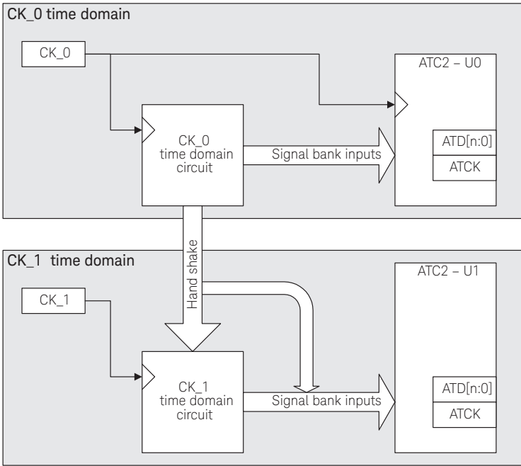
Figure 23. One state core and one timing core
