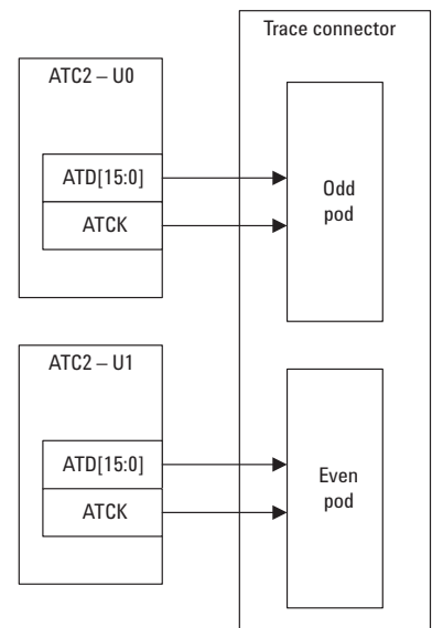
Figure 3. ATC2 core connected to logic analysis acquisition connector
