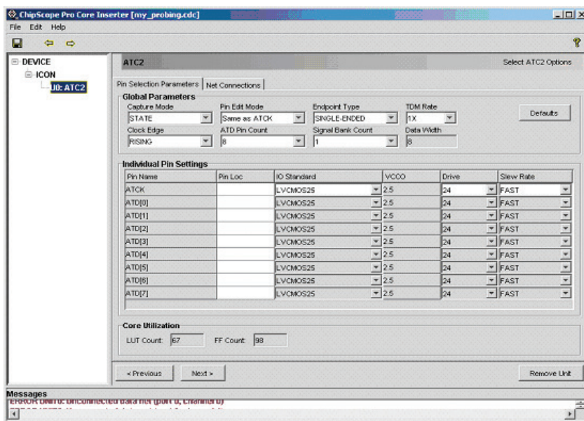
Figure 18. Unconfigured ATC2 core
