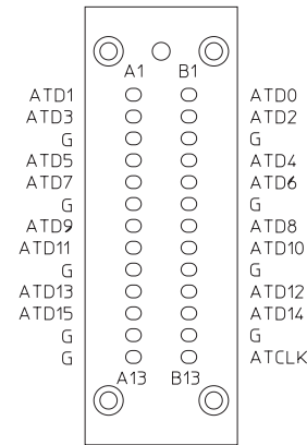
Figure 6. Half soft touch connector
