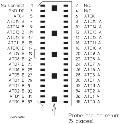
38-Channel Footprint
