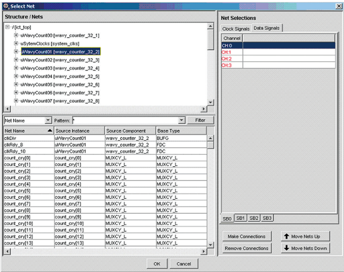
Figure 21. Data Signals tab
