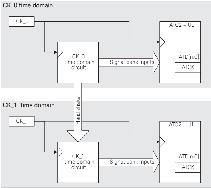
Figure 22. Two state cores for two time bases
