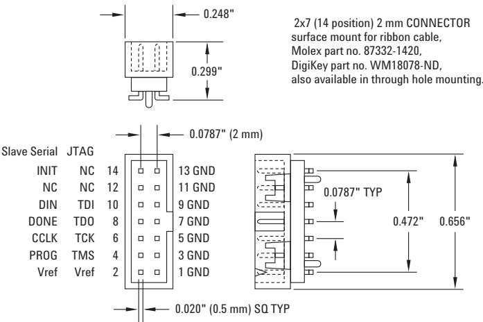
Figure 1. Xilinx target interface connector (reprinted from "Xilinx Parallel Cable IV," with permission from Xilinx Corporation)
