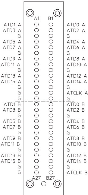
Figure 5. Soft touch single-ended connector
