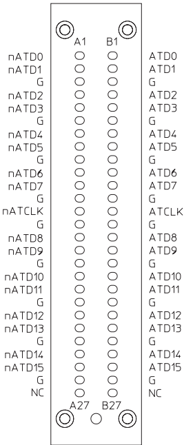
Figure 4. Soft touch differential connector
