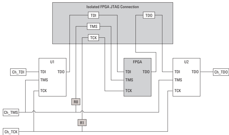
Figure 2. Isolated FPGA
