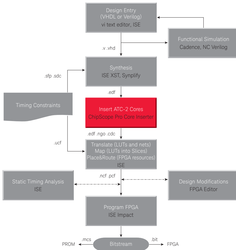
Figure 9. Design flow with core insertion
