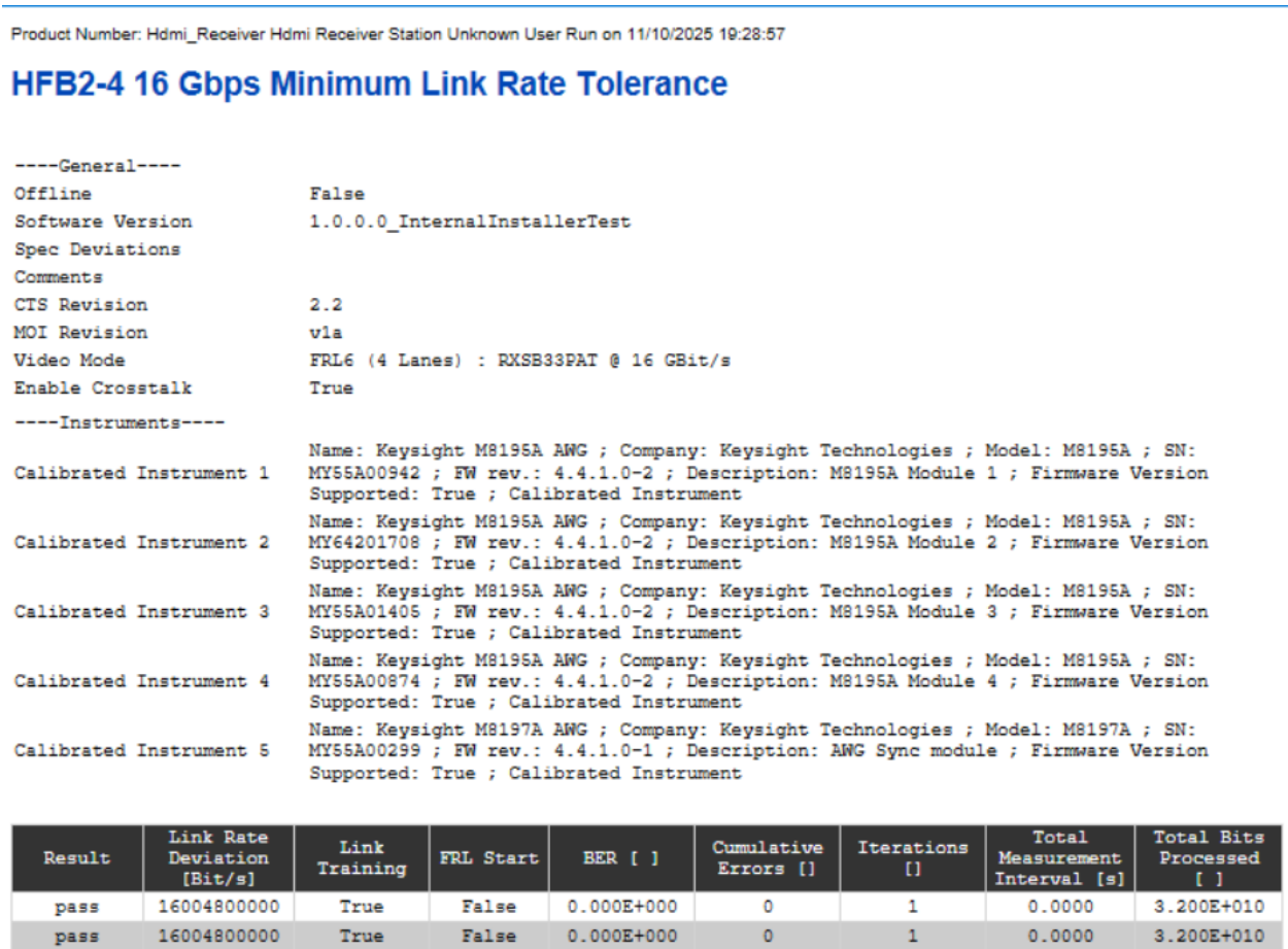
Figure 7. Minimum Link Rate Tolerance Test report
