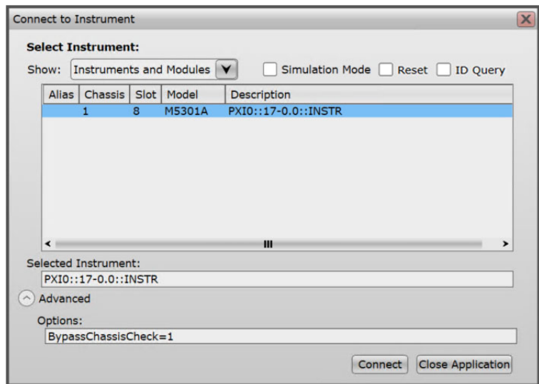
Figure 11 Checking M5301A connection in M5301x SFP
