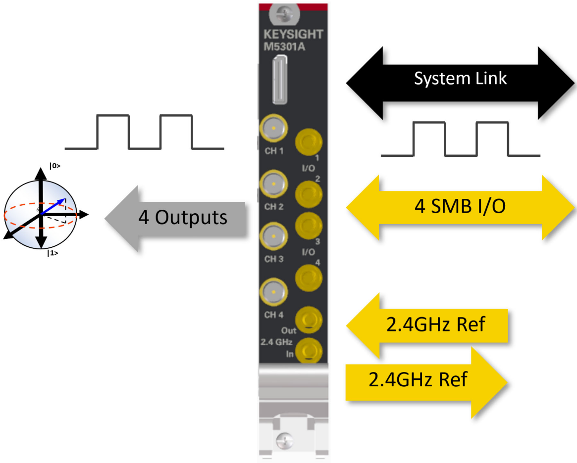
Figure 2 Functional depiction of the M5301A module
