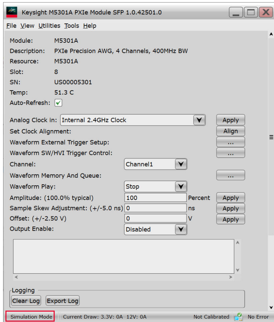
Figure 32 “Simulation Mode” in the status bar on the main window
