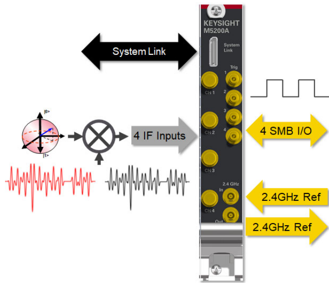
Figure 2 Functional depiction of the M5200A module
