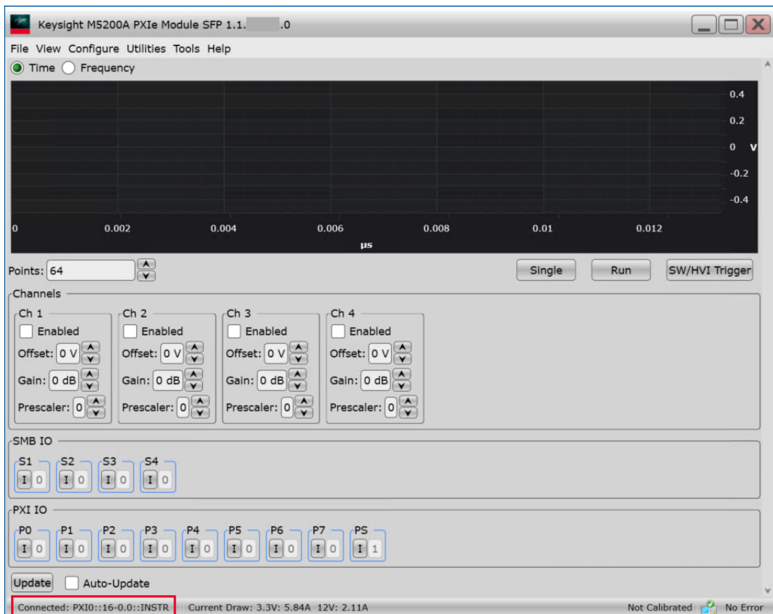
Figure 34 “Connected to <VISA address>” in the status bar on the main window
