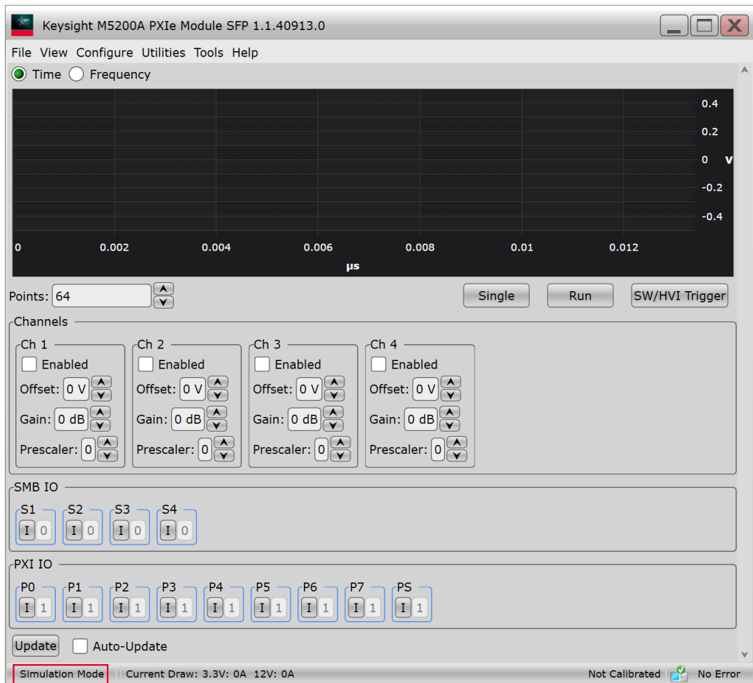
Figure 32 “Simulation Mode” in the status bar on the main window
