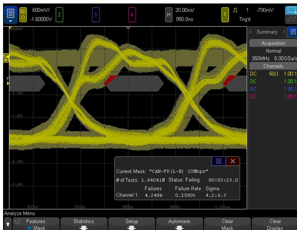
Figure 10. CAN FD eye-diagram mask testing.
