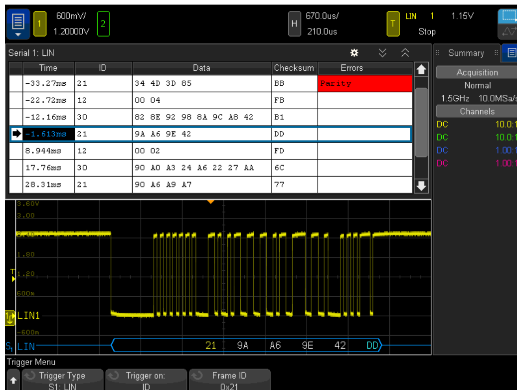
Figure 4. LIN decode on an InfiniiVision X-Series oscilloscope.
