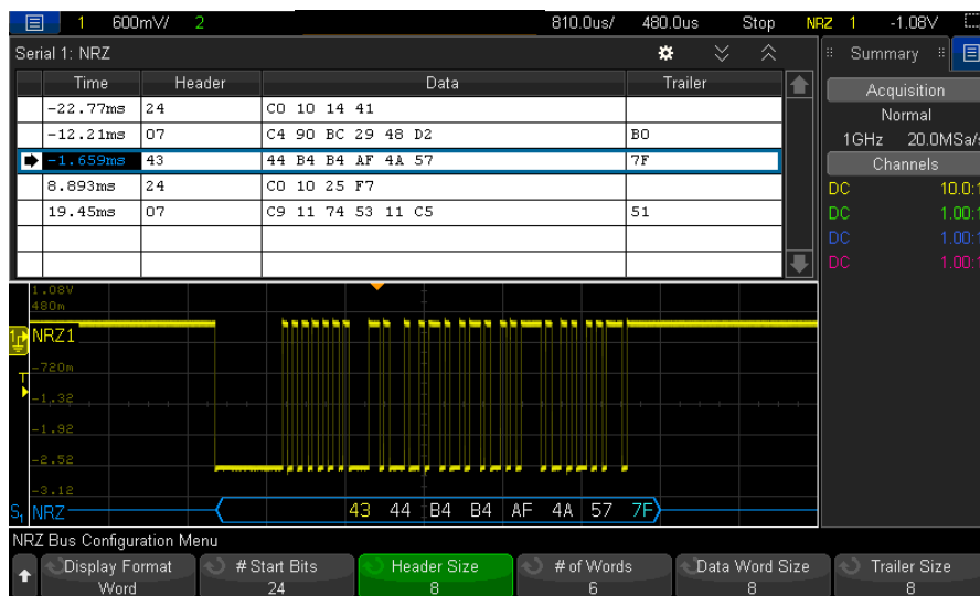
Figure 8. User-definable NRZ decode on an InfiniiVision X-Series oscilloscope.
