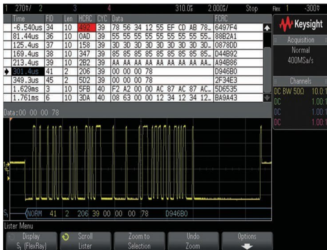
Figure 5. FlexRay decode on an InfiniiVision X-Series oscilloscope.
