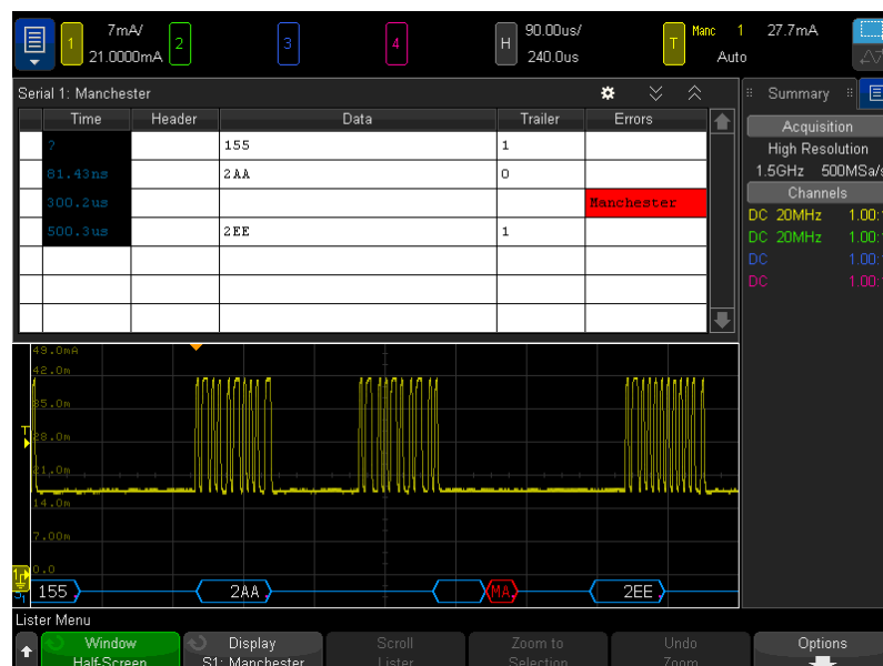
Figure 7. PSI5 decode on an InfiniiVision X-Series oscilloscope.
