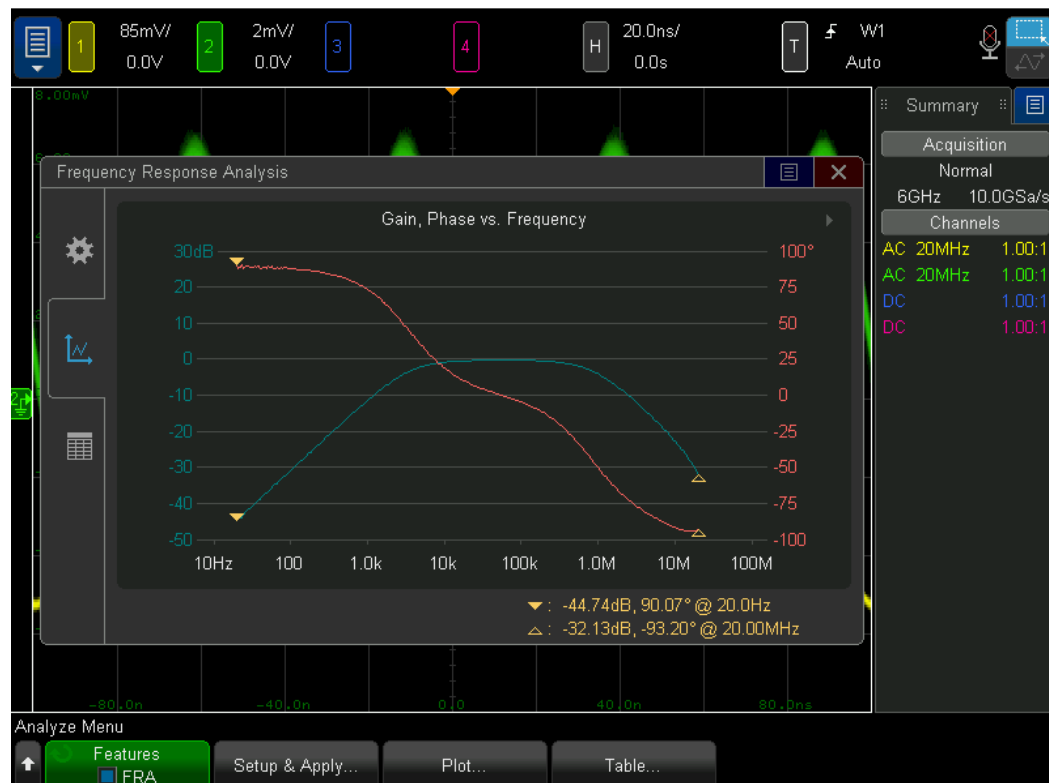
Figure 11. Frequency response analysis (gain & phase) on a bandpass filter.
