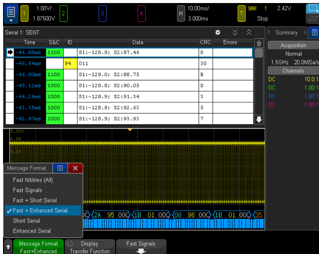
Figure 6. SENT decode on an InfiniiVision X-Series oscilloscope.
