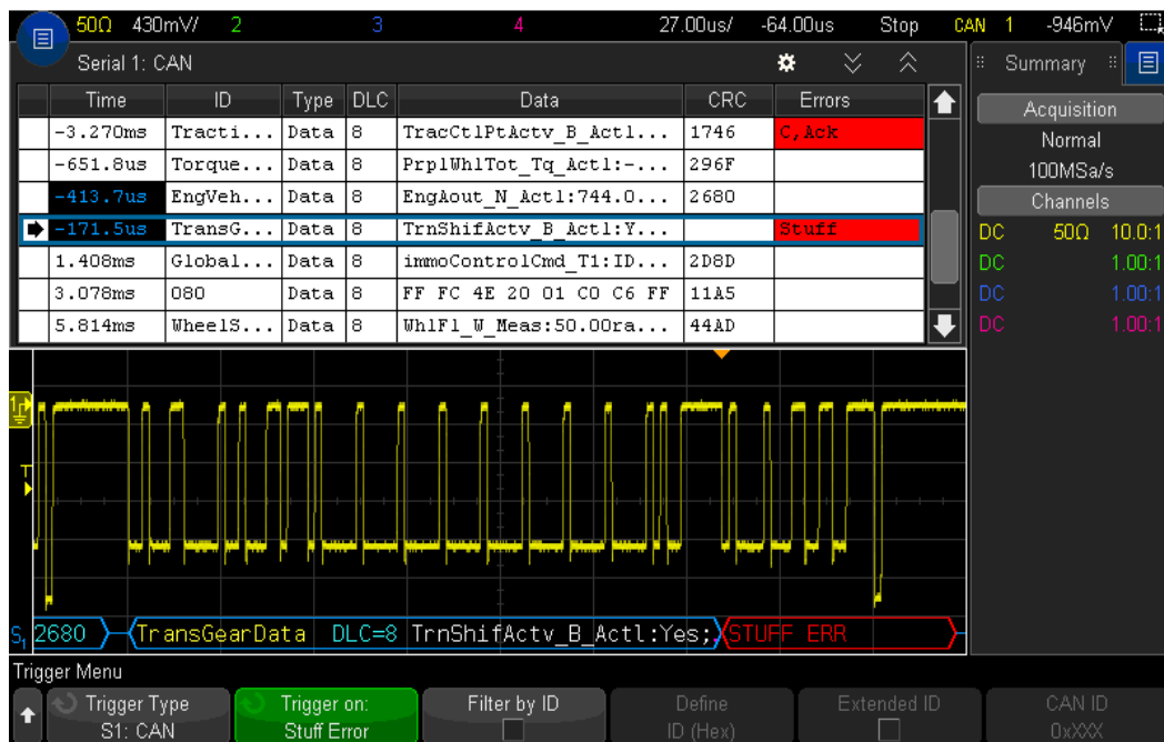
Figure 3. CAN decode on an InfiniiVision X-Series oscilloscope.
