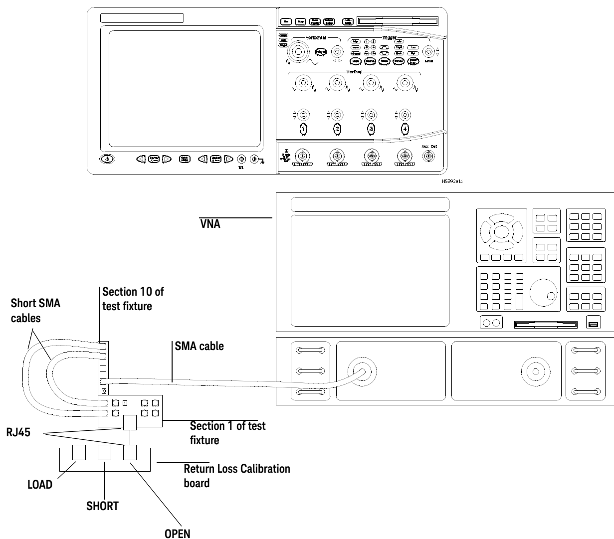
Figure 35 VNA Calibration
