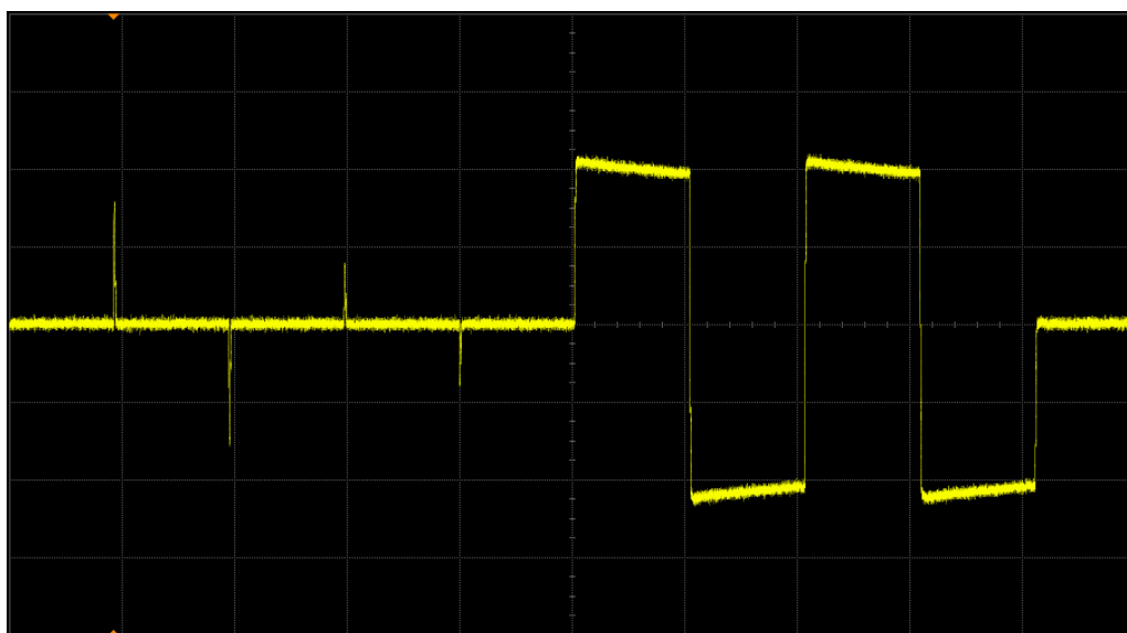
Figure 23 Example of Transmitter Test Mode 1 Waveform (1 Cycle)
