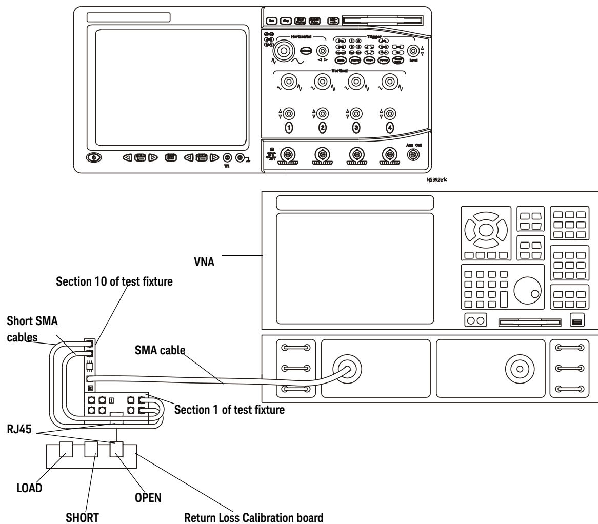
Figure 45 VNA Calibration
