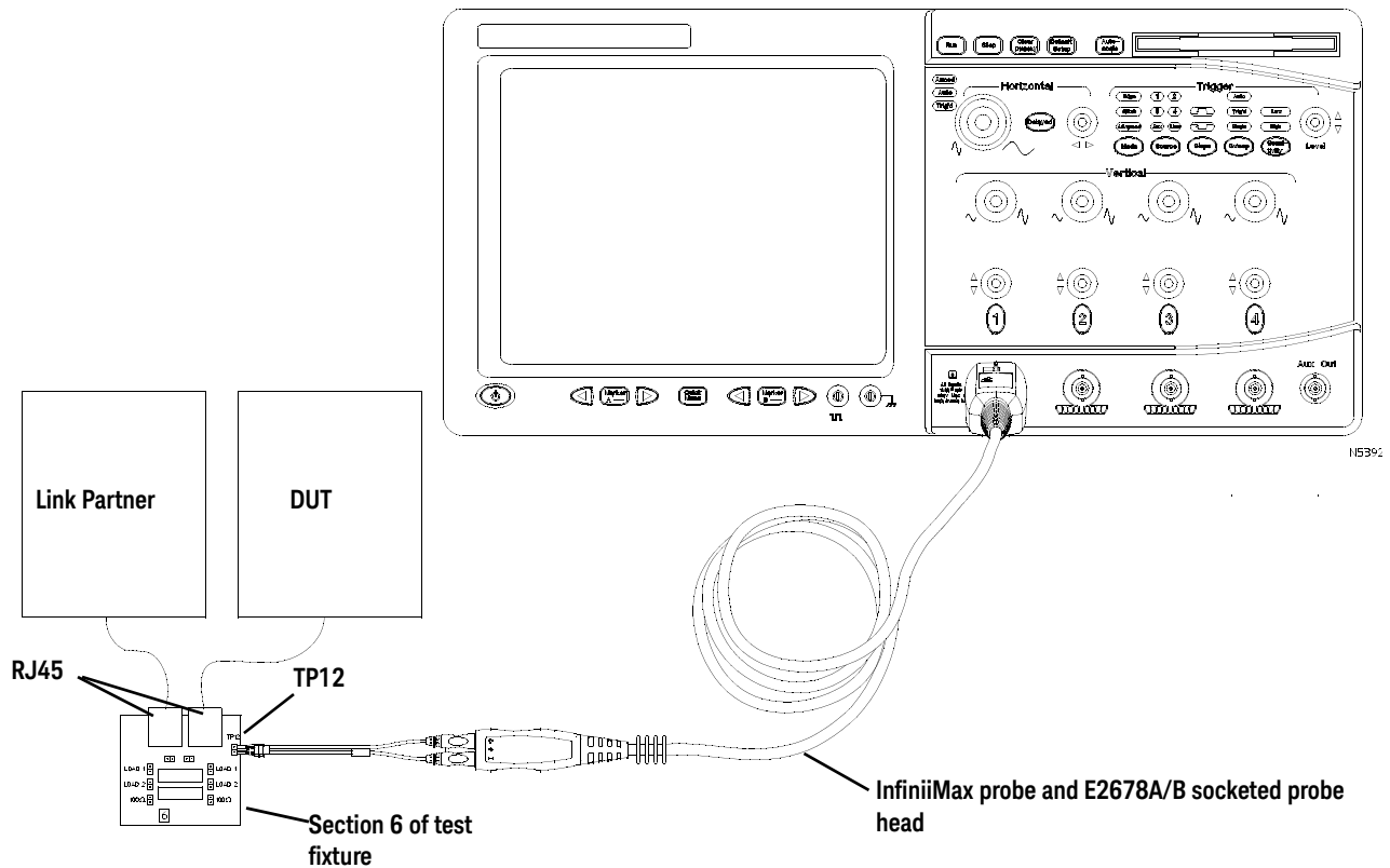
Figure 49 Probing for 10 Base-T Tests Without the TPM, With Link Partner
