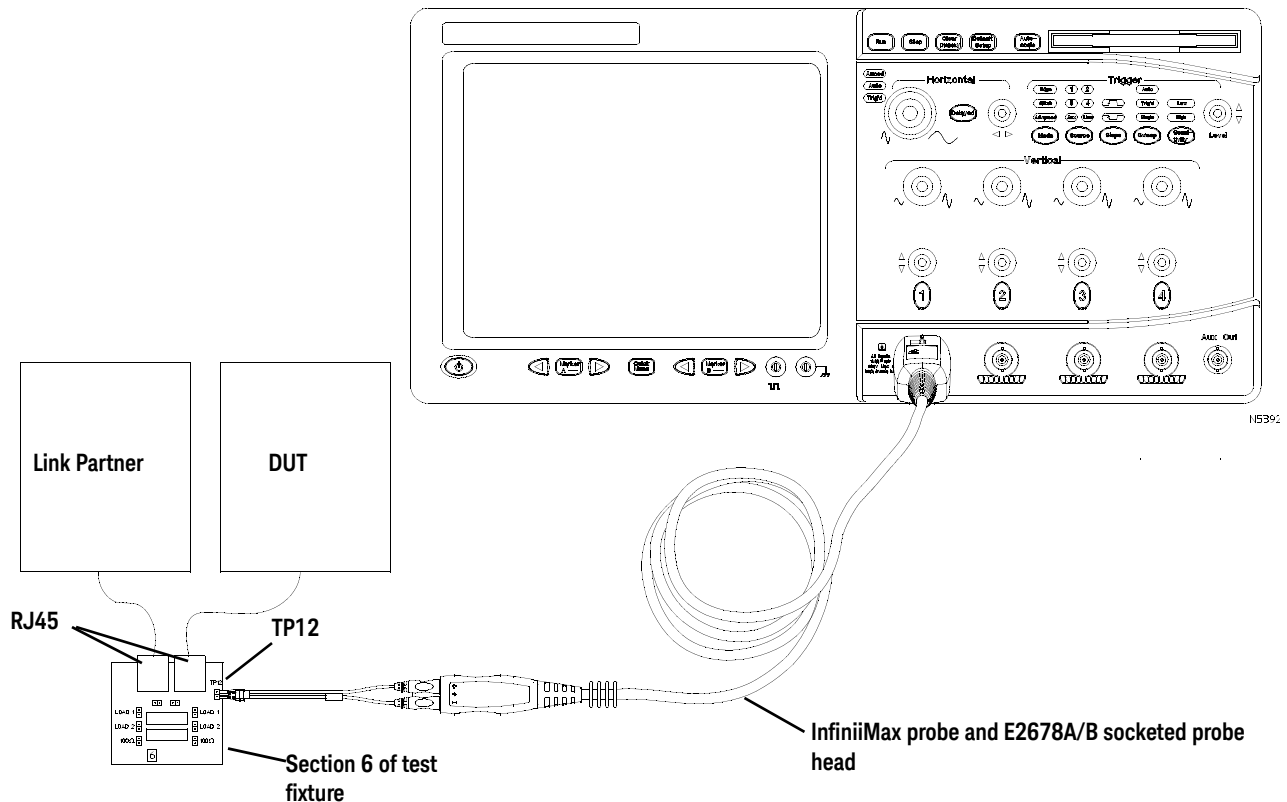
Figure 60 Probing for 10 Base-Te Tests Without TPM, With Link Partner
