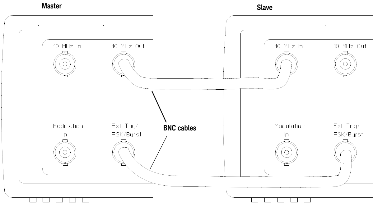
Figure 18 Rear Panel Cable Connections for the 33250A Generators
