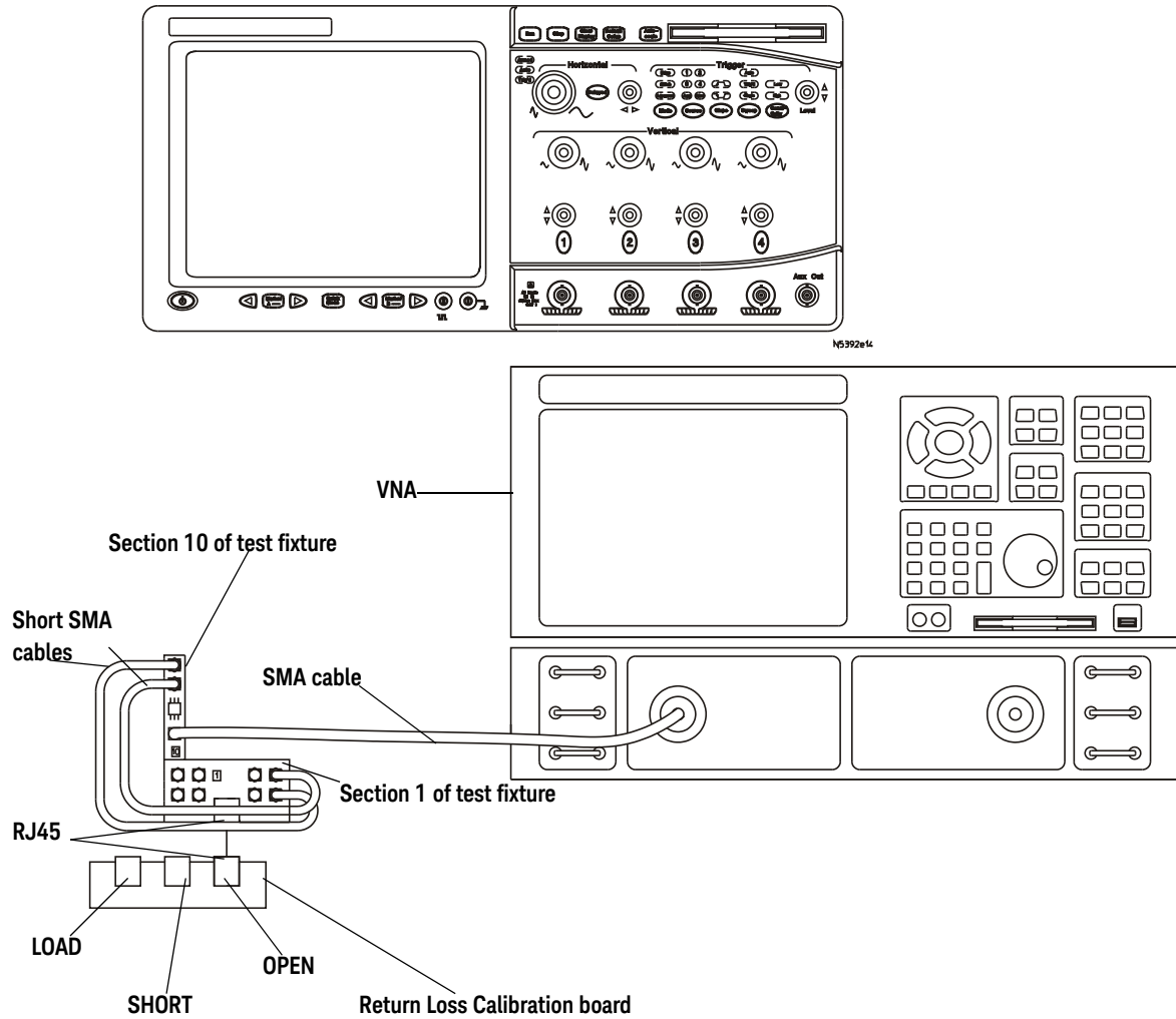
Figure 55 VNA Calibration
