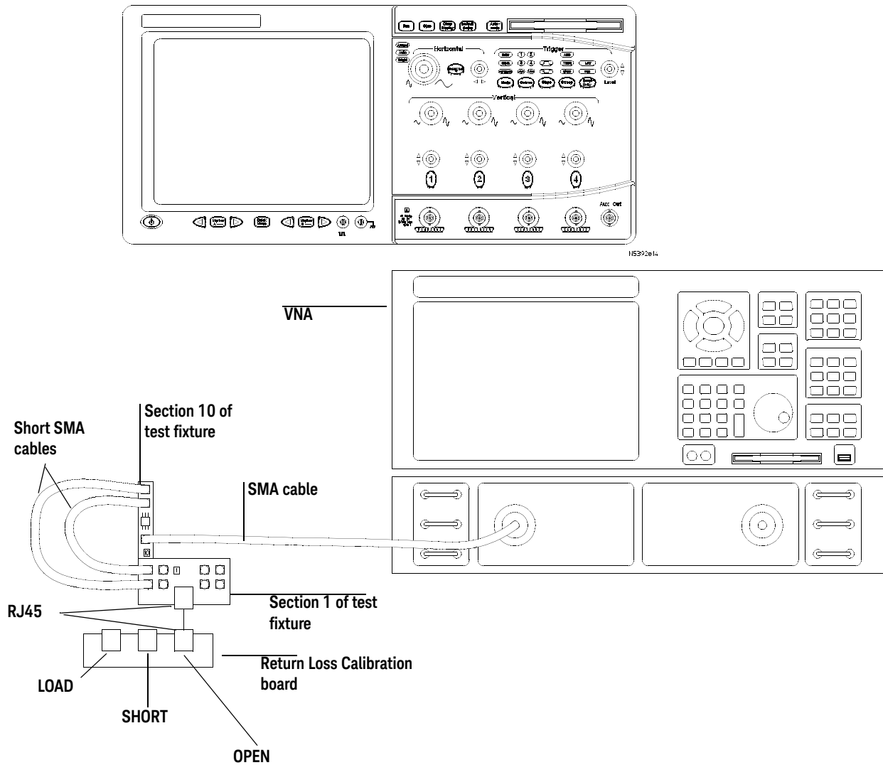
Figure 43 VNA Calibration
