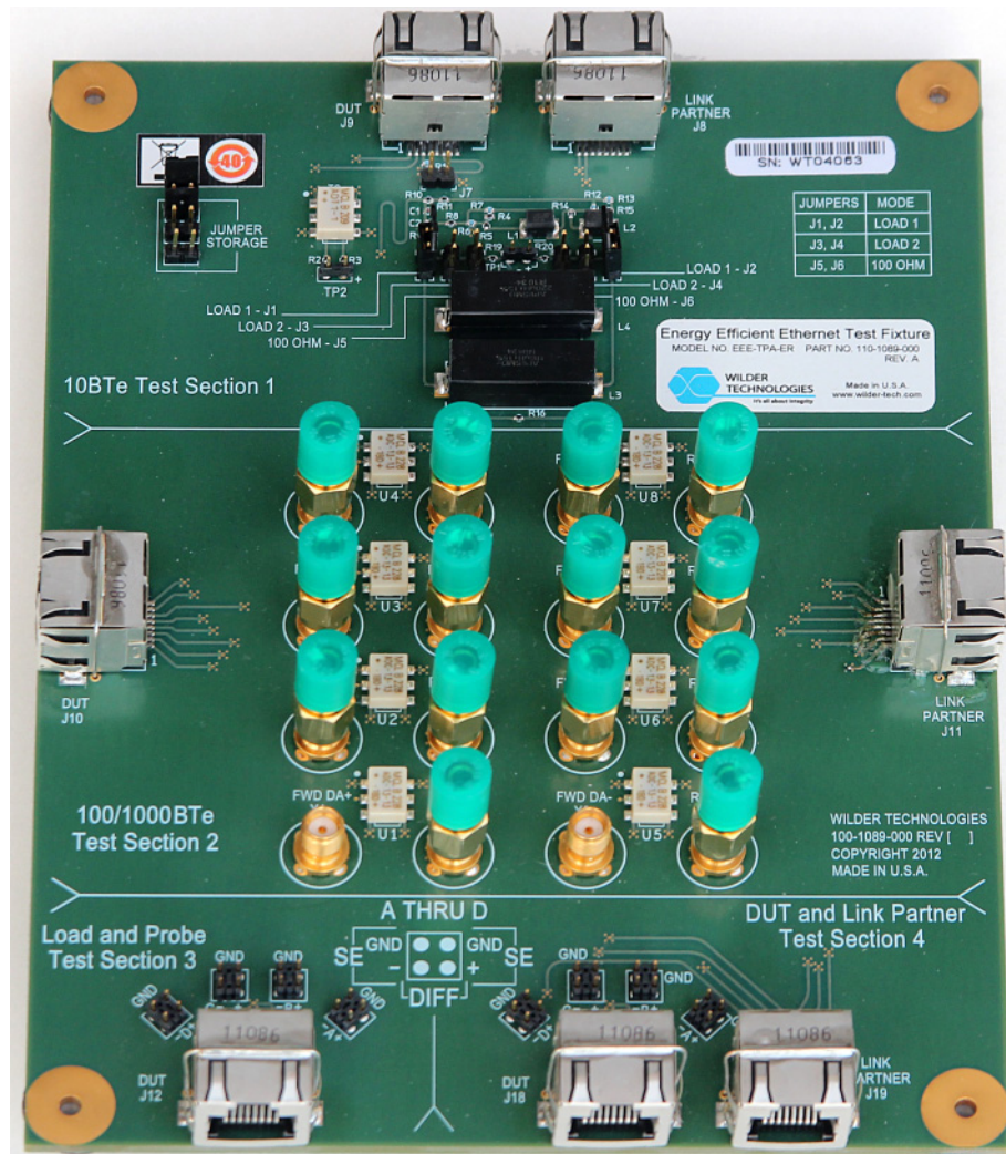
Figure 6 Wilder Technologies EEE Electrical Compliance Test Board
