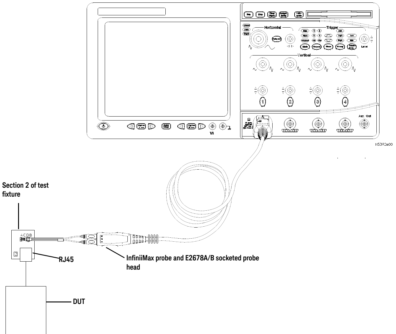
Figure 14 Probing for 1000 Base-T Test Mode 1 Tests
