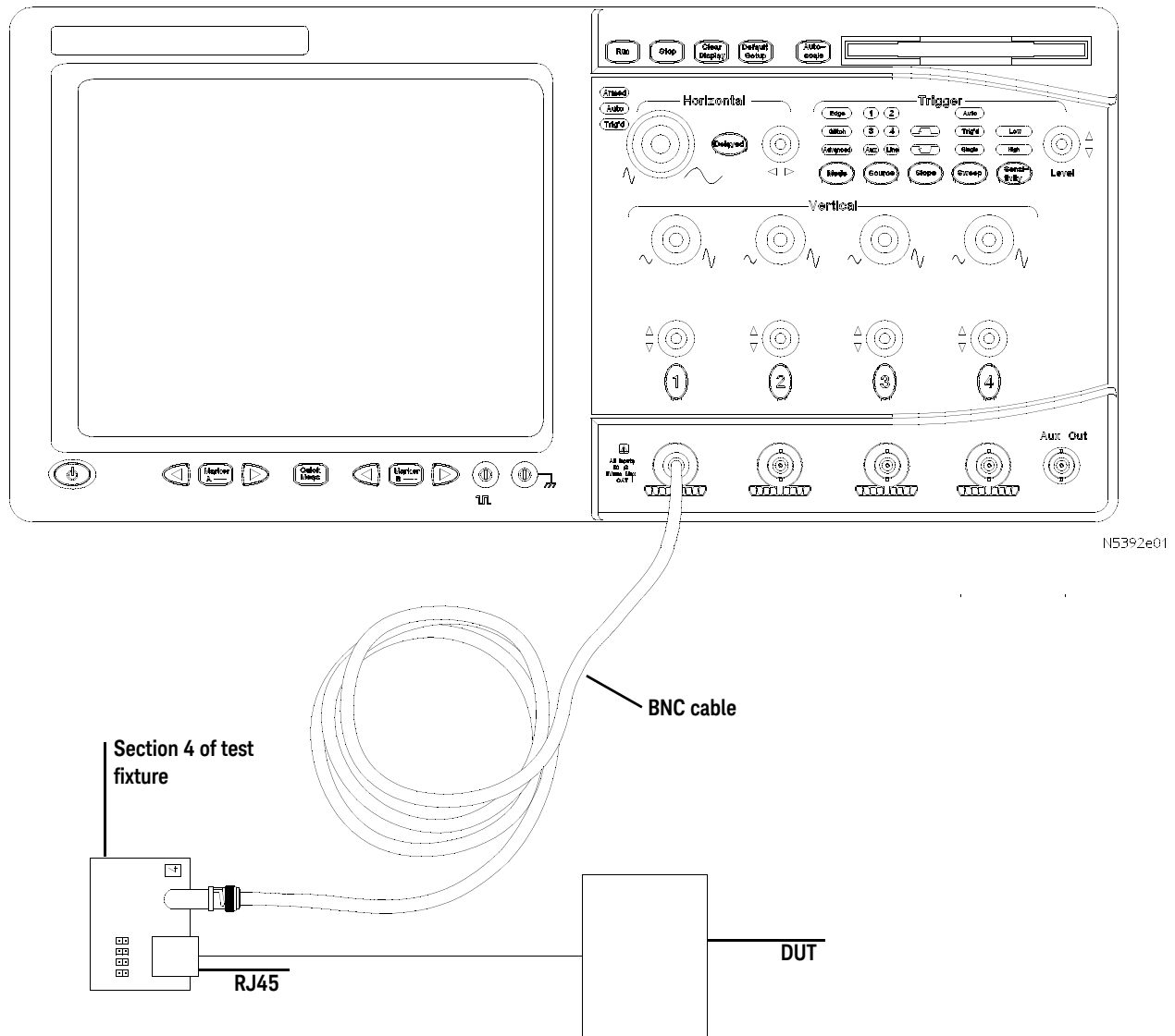
Figure 61 Probing for 10 Base-Tc Common Mode Output Voltage
