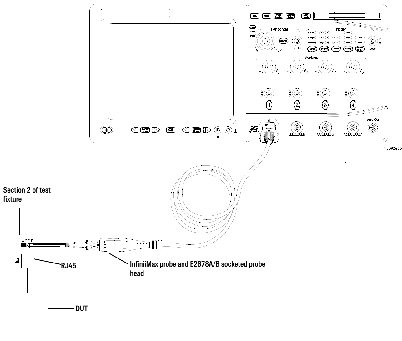
Figure 37 Probing for 100 Base-TX Tests, Without Link Partner
