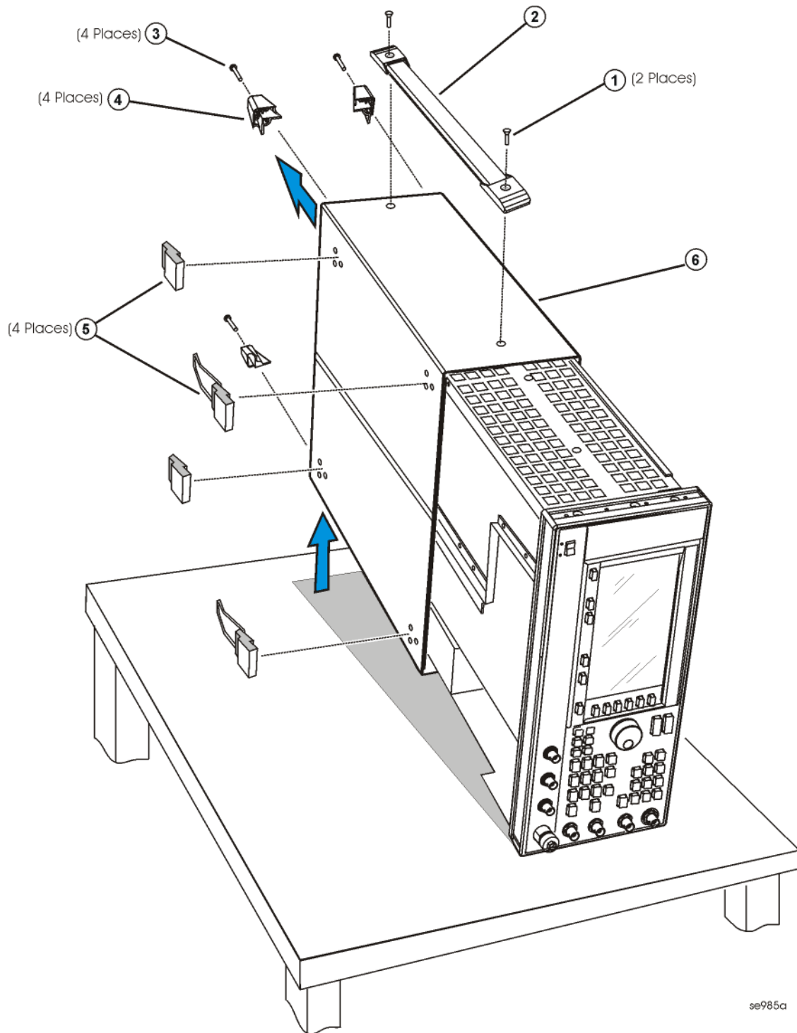
Figure 3 Outer Cover Removal
