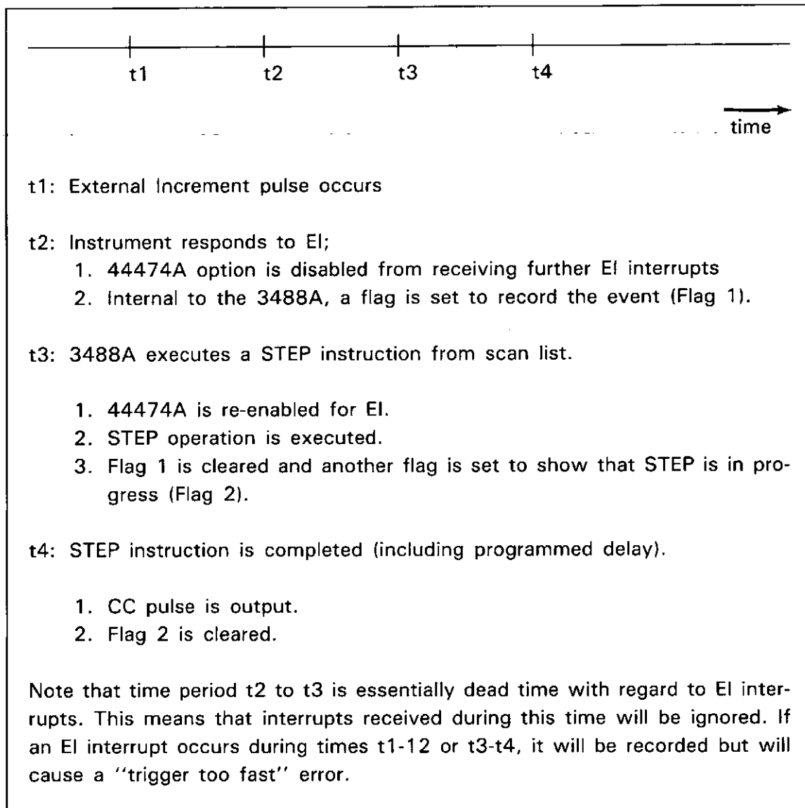
Figure 10-4. Scan Timing
