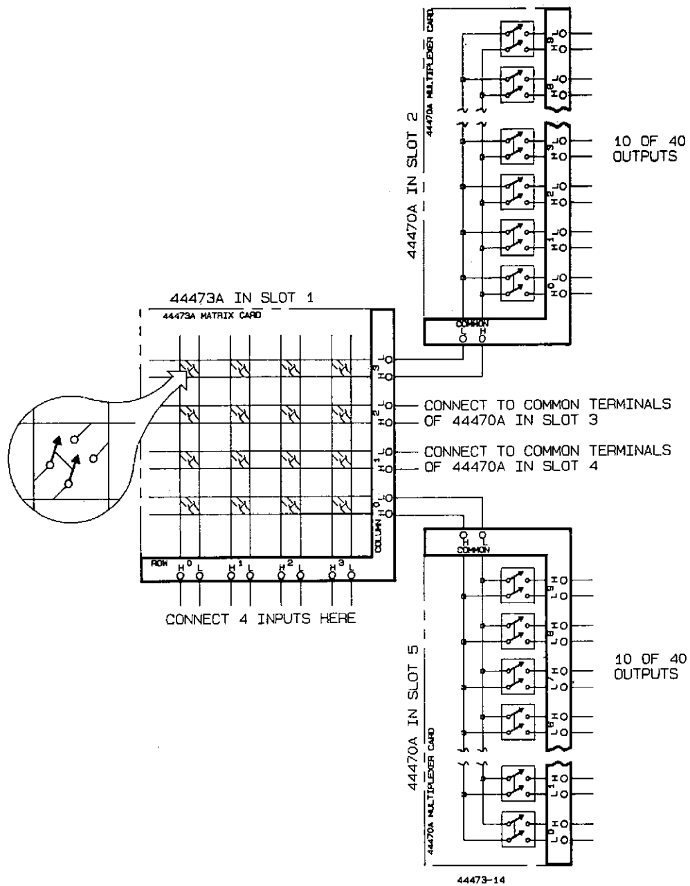
Figure 9-12. 4x40 Matrix
