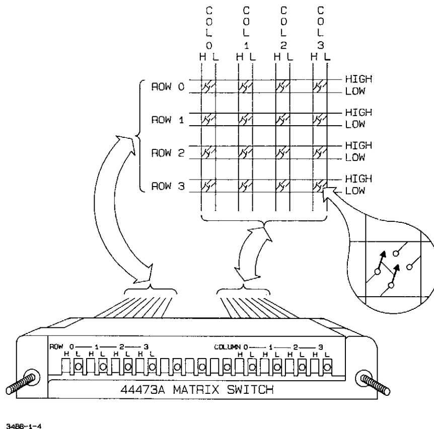
Figure 9-1. 44473A Simplified Schematic
