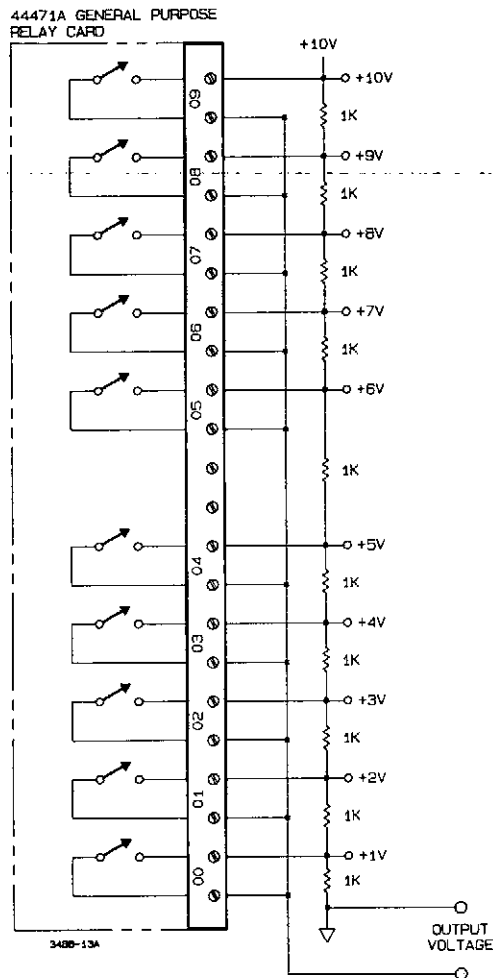
Figure 7-15. Voltage Divider
