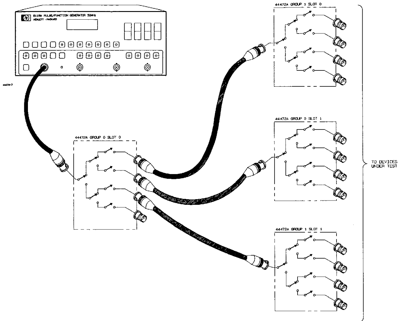
Figure 8-6. Tree Configuration
