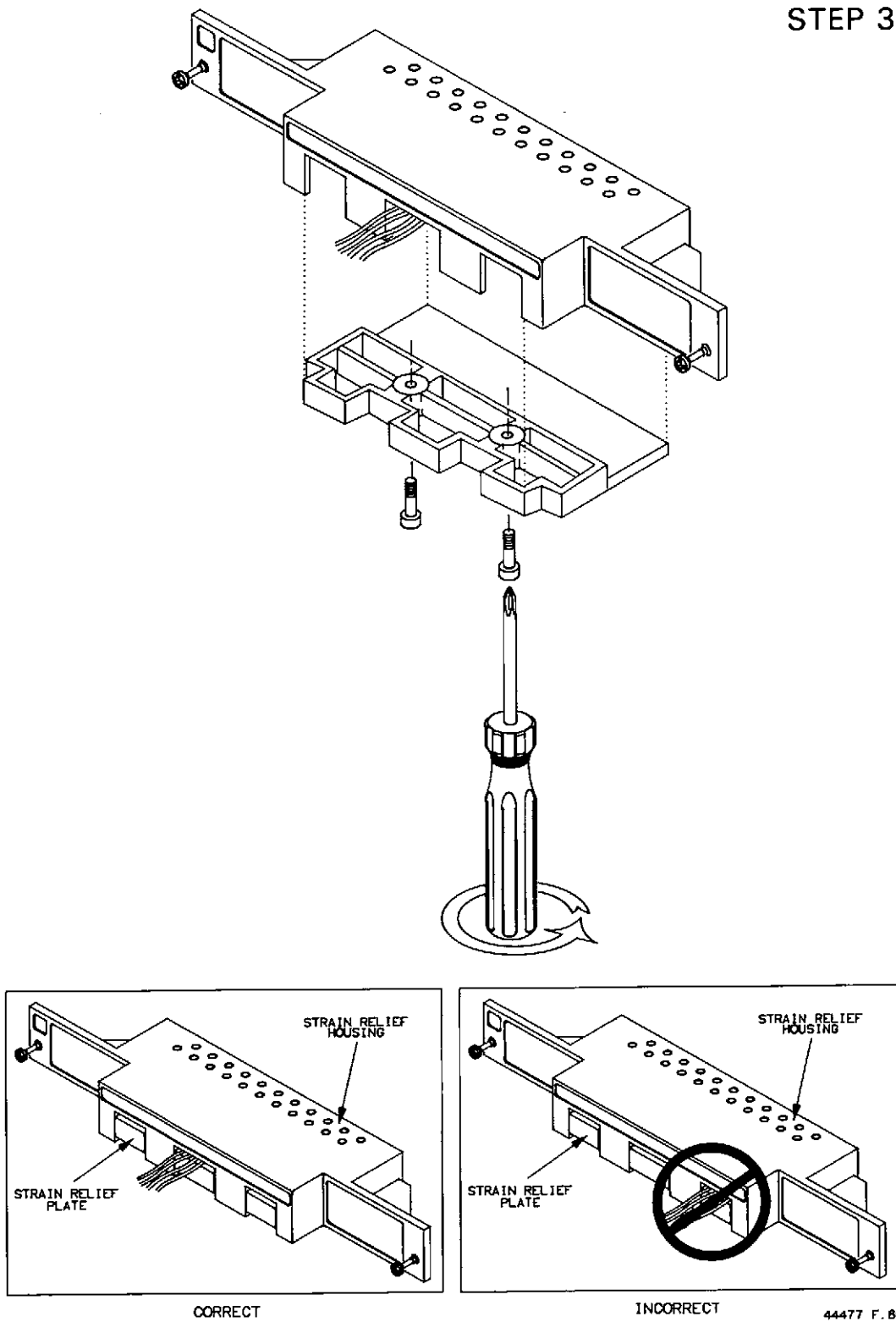
Figure 13-4. Installing the Terminal Block
