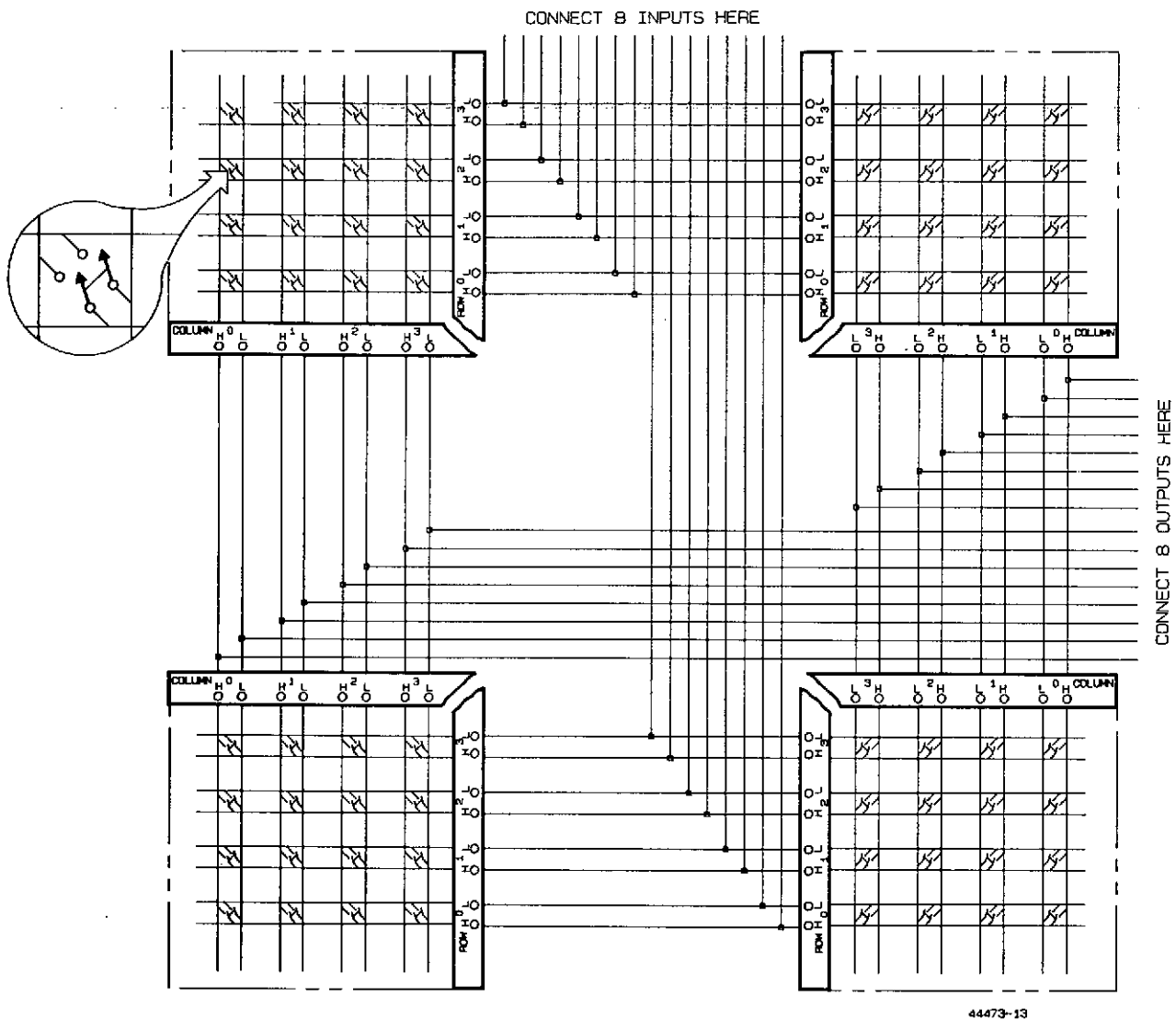
Figure 9-11. 8x8 Matrix
