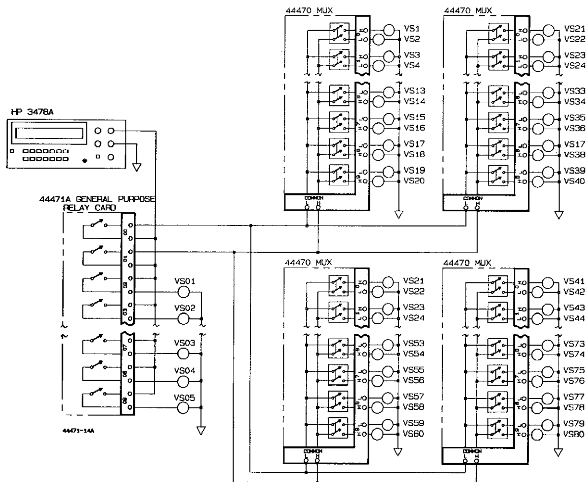
Figure 7-16. Single-ended Measurements
