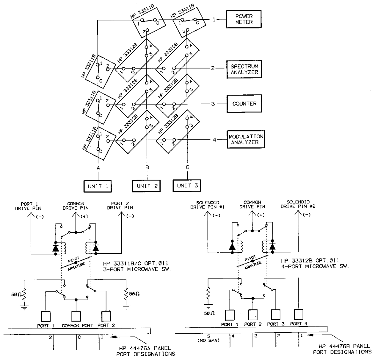
Figure 12-9. Matrix Application
