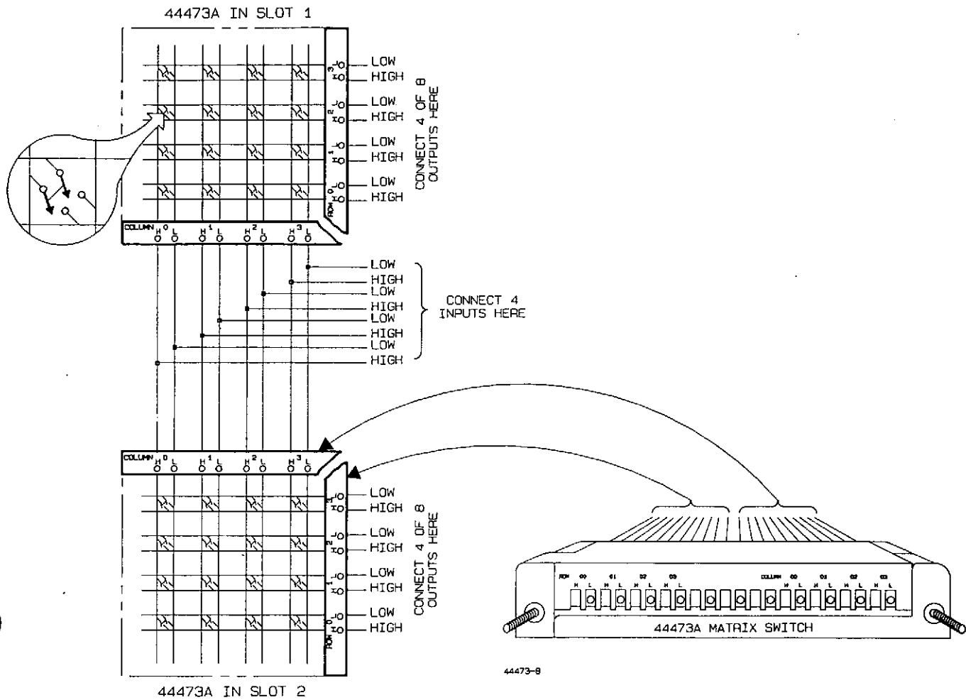
Figure 9-7. 4x8 Matrix
