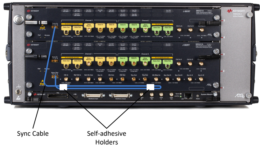
Figure 21 Synchronization cable routing
