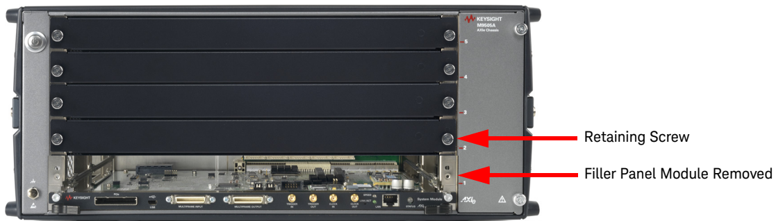
Figure 18 Filler panel module removed
