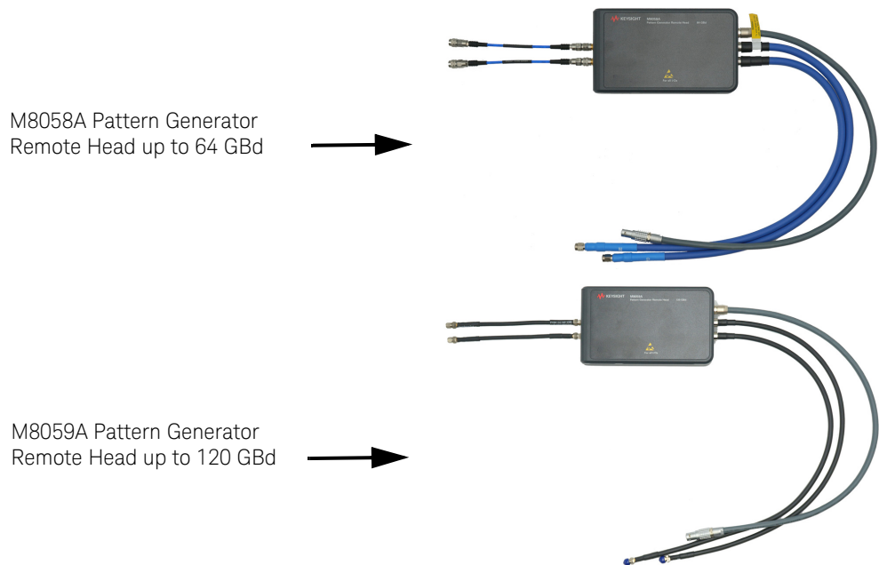
Figure 11 M8058A and M8059A Remote Heads for M8042A Pattern Generator
