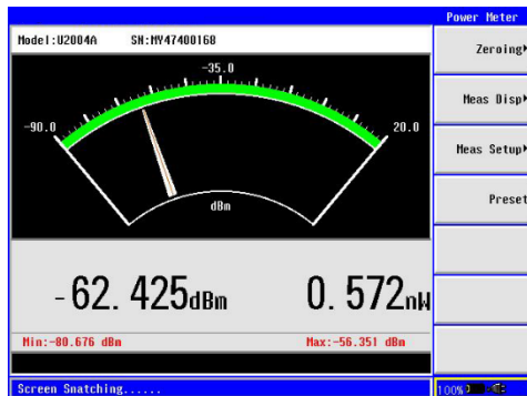
Figure 9. N9340B HSA HHSA turns into a power-meter measurement
