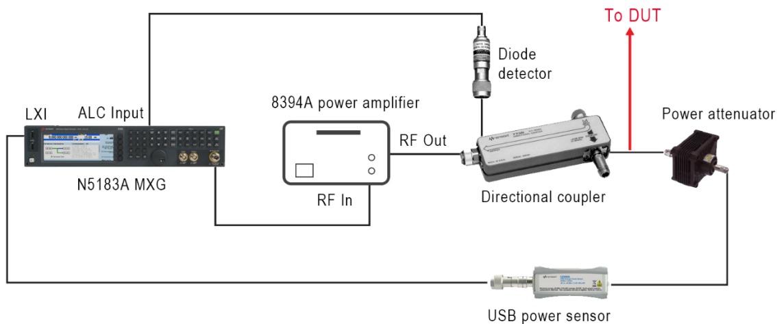
Figure 14. Power meter servo configuration
