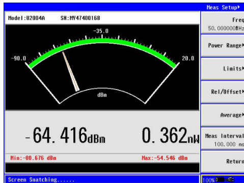
Figure 13. Measurement Setup menu with meter-view display measurement.
