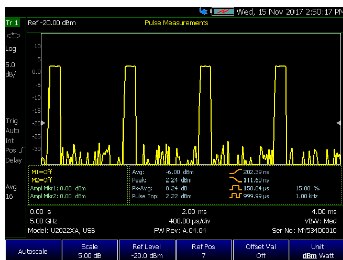
Figure 22. Pulse Measurement mode requires U2020 X-Series USB peak and average power sensors to measure the RF pulse signal.
