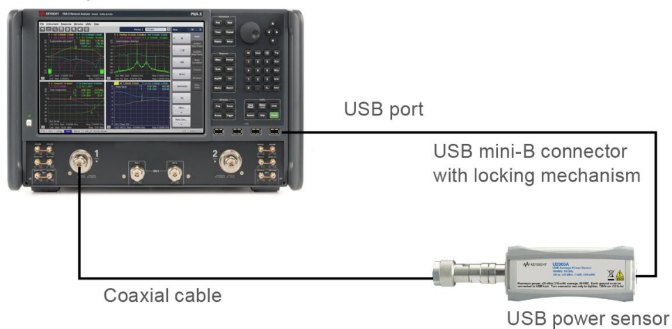
Figure 3. USB power sensor connecting directly to a PNA USB port through a USB mini-B connector.
