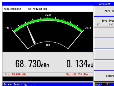
Figure 10. External and internal zeroing are performed to reduce the zero offset and noise impact in order to measure power accurately.
