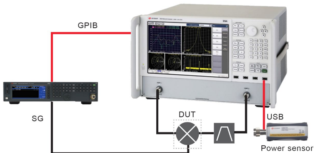
Figure 7. Scalar Mixer Calibration (SMC) setup using a USB power sensor
