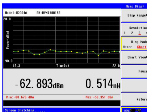
Figure 12. Measurement display in chart format.
