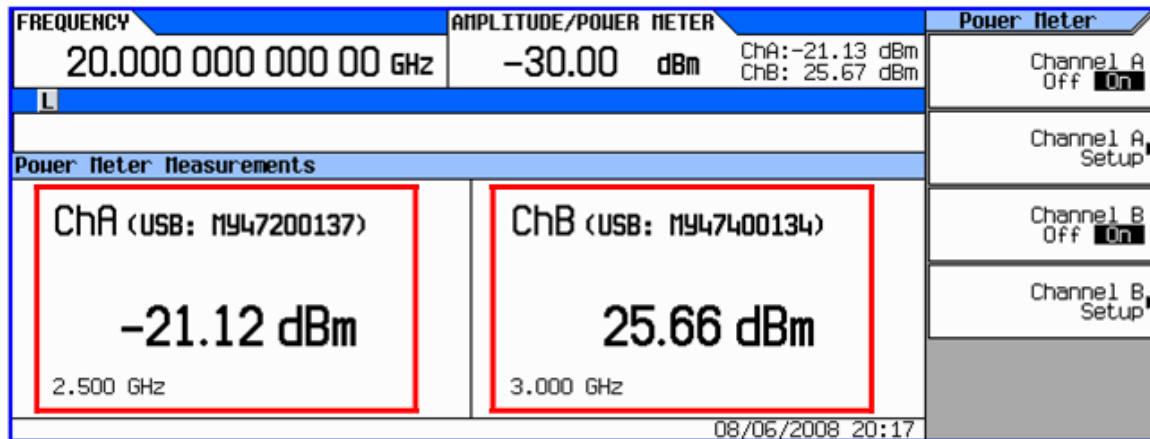
Figure 17. Dual power meter display function on MXG signal generator.
