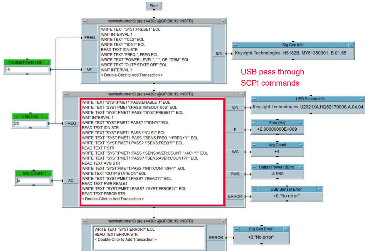
Figure 20. USB pass through SCPI commands (highlighted in red box) using the X-Series signal generator
