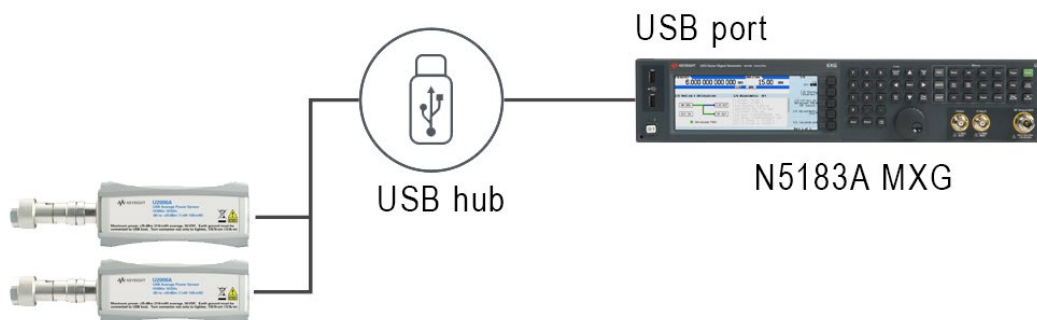
Figure 16. Connection diagram of two USB power sensors on MXG via external USB hub
