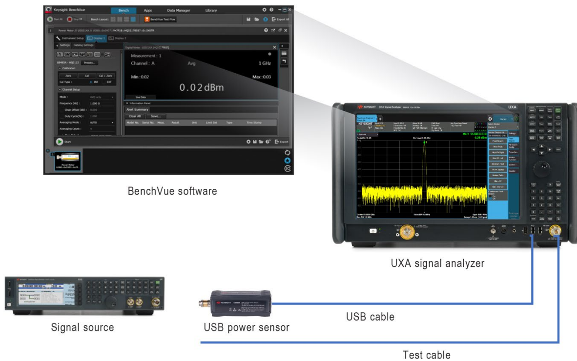
Figure 23. Power measurement with the USB power sensor and BenchVue software running on the UXA
