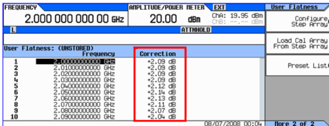
Figure 15. Correction factors automatically performed and displayed on the MXG.
