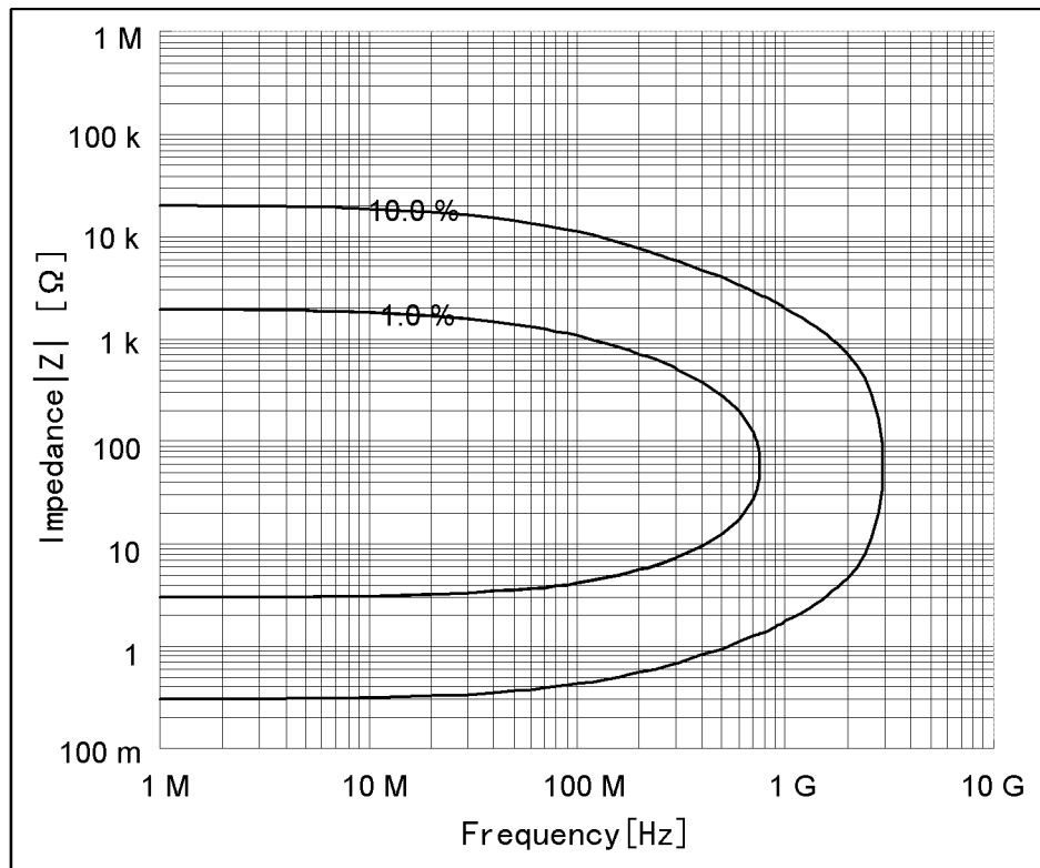
Additional Error for Impedance
