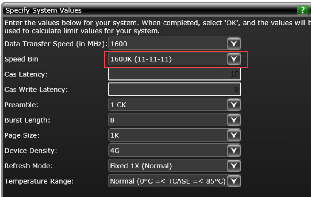
Screen 2 showing the Speed Bin system value changed to 11-11-11
