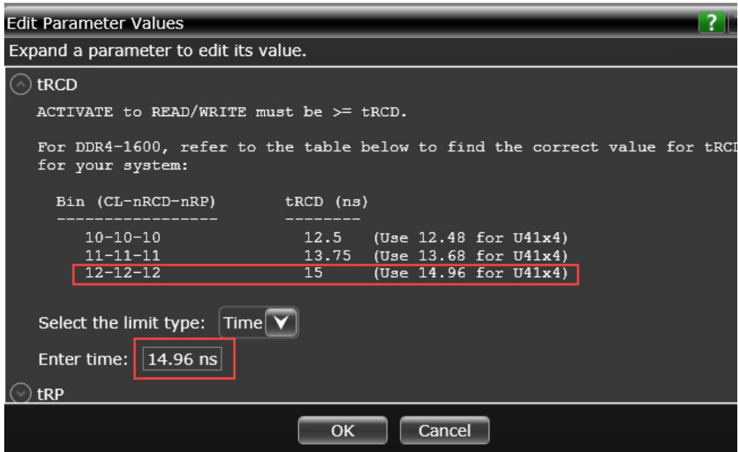
Screen 1 showing the default value of the tRCD parameter
