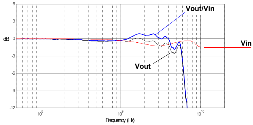
Figure 142 Graph of Vin and Vout of probe with a 25Ω source and Vout/Vin frequency response.
