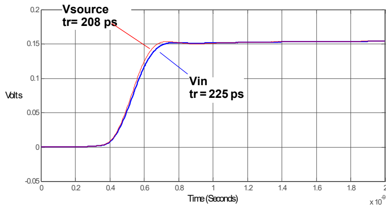
Figure 129 Graph of 25Ω 200 ps step generator with and without probe connected.
