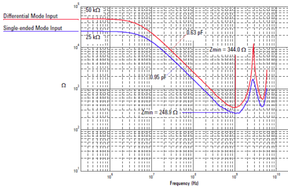
Figure 87 Magnitude plot of probe input impedance versus frequency.
