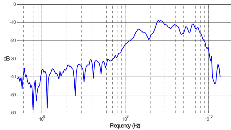
Figure 214 Graph of V_{out}/V_{in} frequency response when inputs driven in common (common mode rejection).
