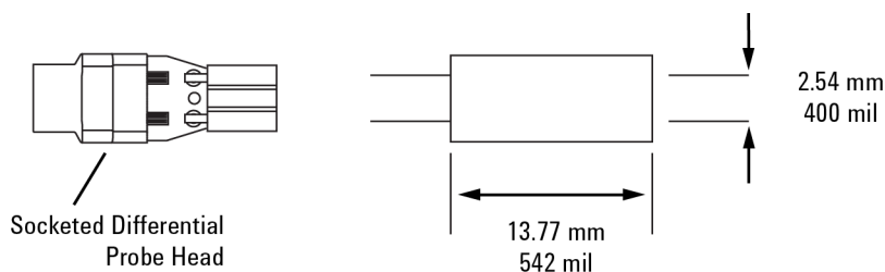
Figure 44 01130-63201 Header Adapter Dimensions
