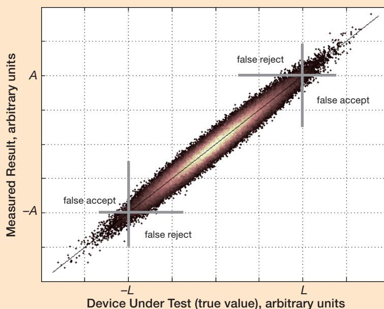
Figure 2. False accept and false reject regions based on specified tolerance limits ( -L , L ) and acceptance limits ( -A , A ).
