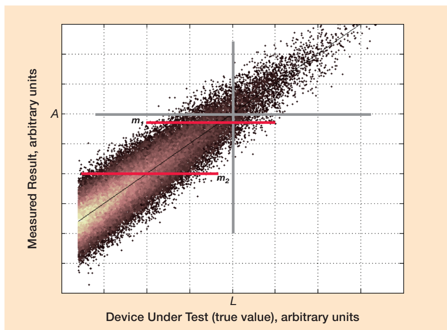
Figure 3. Conditional risk for tolerance limit, L , and acceptance limit, A .
