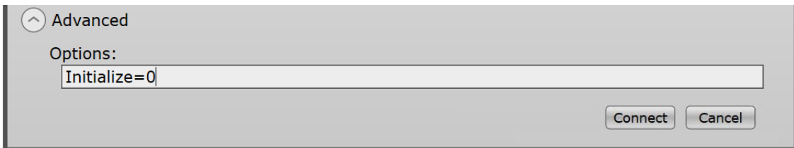
Figure 42 Setting option 'Initialize=0' to perform firmware update through SFP
