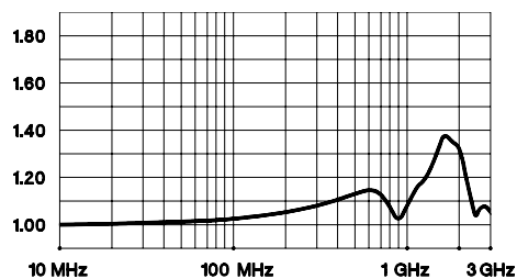
VSWR (50Ω)
