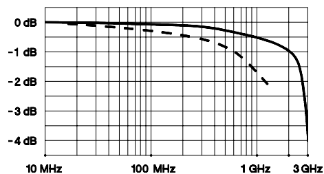
挿入損失 (50Ω)
