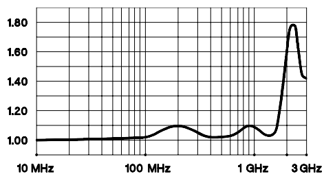
VSWR (75Ω)
