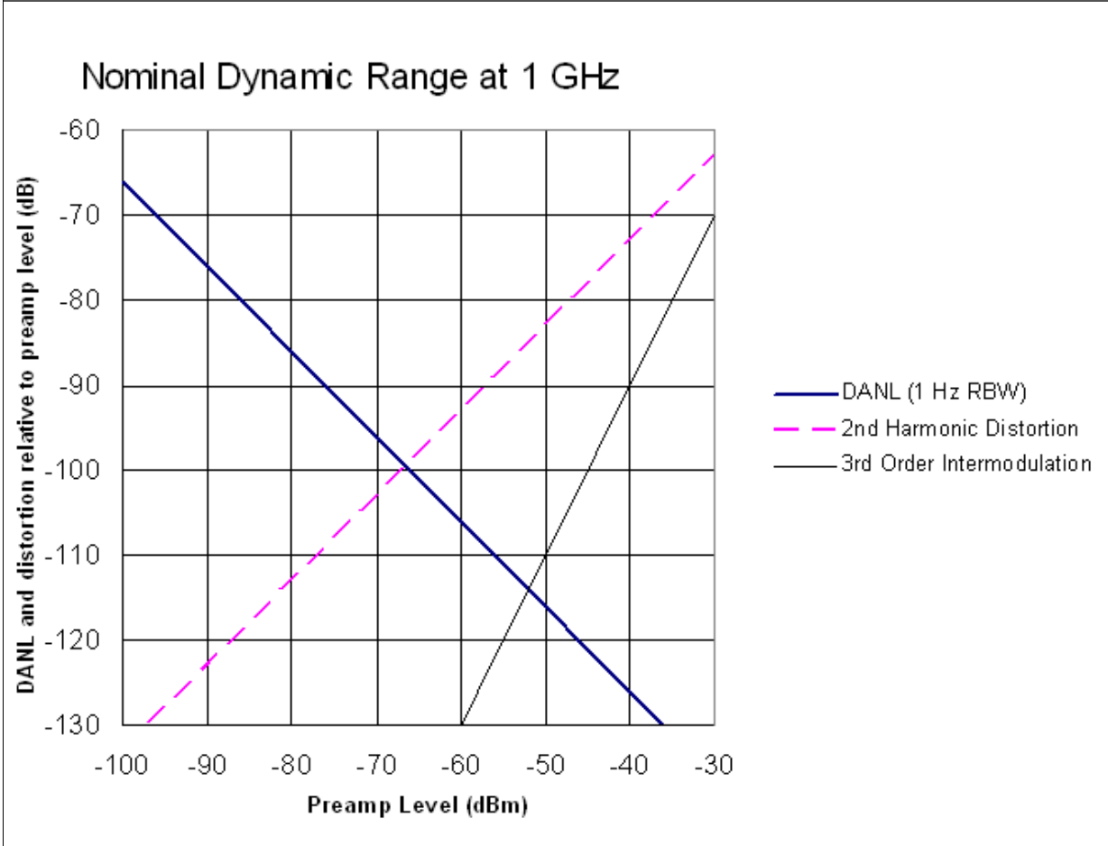
Nominal Dynamic Range at 1 GHz, Preamp On (Plot)
