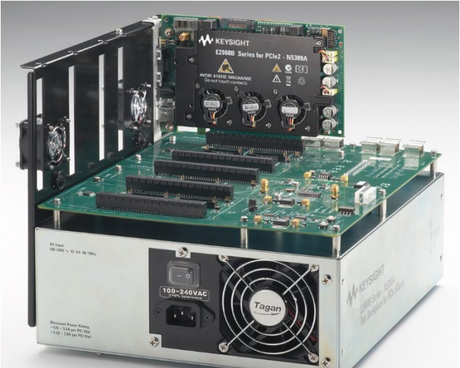
Figure 18. Passive backplane.
