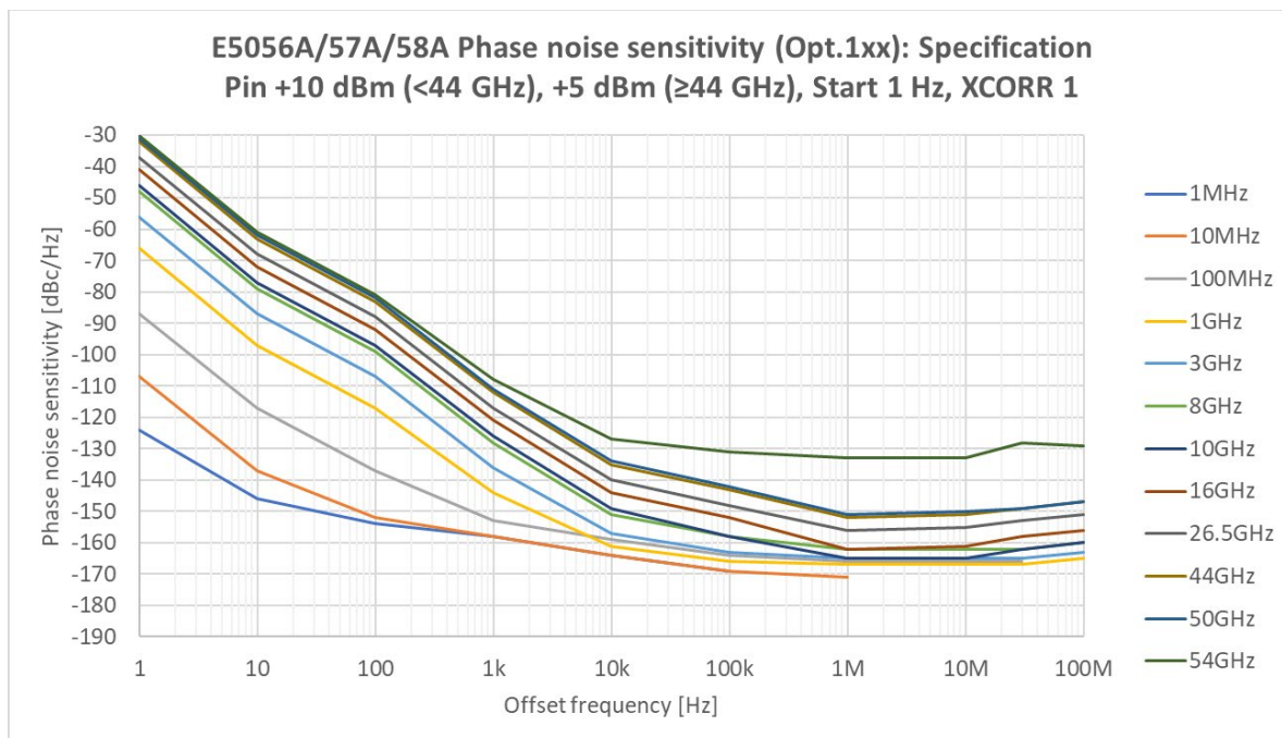
Figure 7. SSB Phase noise sensitivity (E5056A/57A/58A Option 1xx): Specification, +10 dBm (< 44 GHz), +5 dBm ( \geq 44 GHz) input, Auto Range OFF, Max. input level = signal level + 3 dB, Auto Range On, start offset frequency = 1 Hz, Cross correlation factor = 1)
