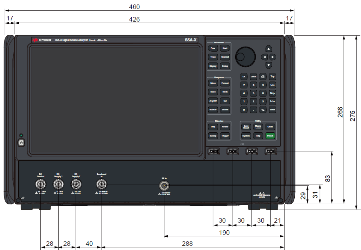
Figure 23. Front view: E505xA Option 100/200 (mm)
