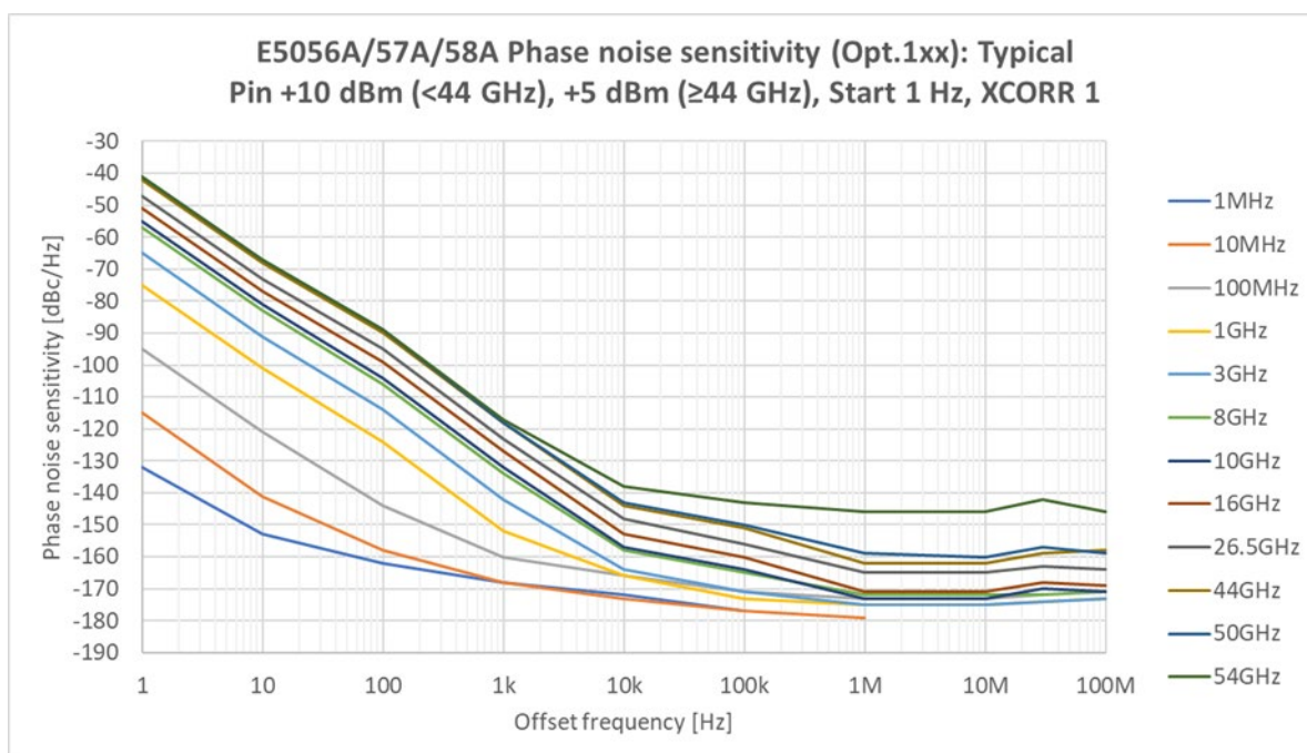
Figure 8. SSB Phase noise sensitivity (E5056A/57A/58A Option 1xx): Typical, +10 dBm (< 44 GHz), +5 dBm ( \geq 44 GHz) input, Auto Range On, start offset frequency = 1 Hz, Cross correlation factor = 1)
