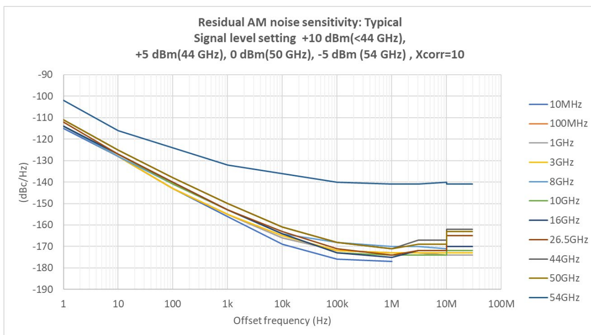
Figure 16. Residual AM phase noise sensitivity (dBc/Hz) (E5055A/56A/57A/58A): Typical, Cross correlation factor = 10, Fast XCORR mode OFF, signal level setting = +10 dBm (< 44 GHz), +5 dBm (44 GHz), 0 dBm (50 GHz), -5 dBm (54 GHz), Auto range ON, Path delay compensation 0 sec, start offset = 1 Hz 1
