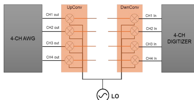
Figure 1: 4-channel coherent radar simulator and analyzer
