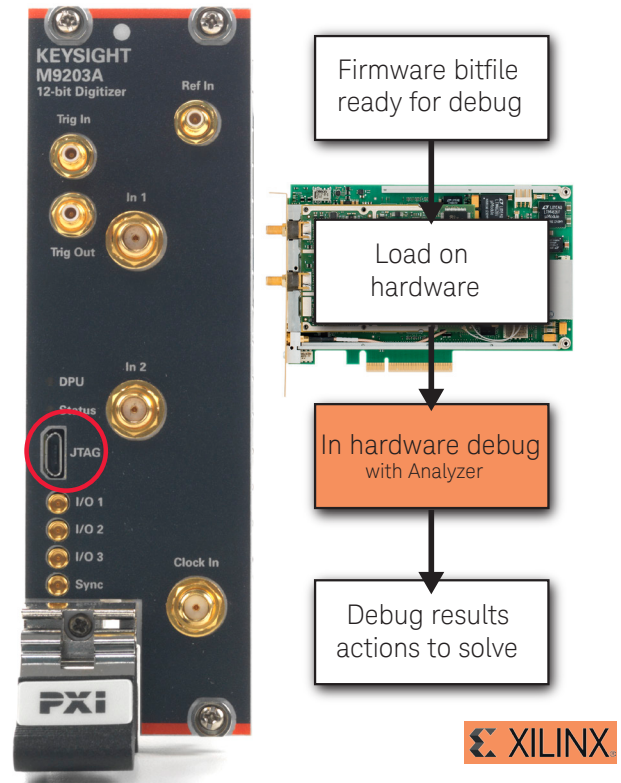
Figure 4. In the PCIe and AXIe high-speed digitizers front-panel, a micro USB connector allows in-system debugging.
