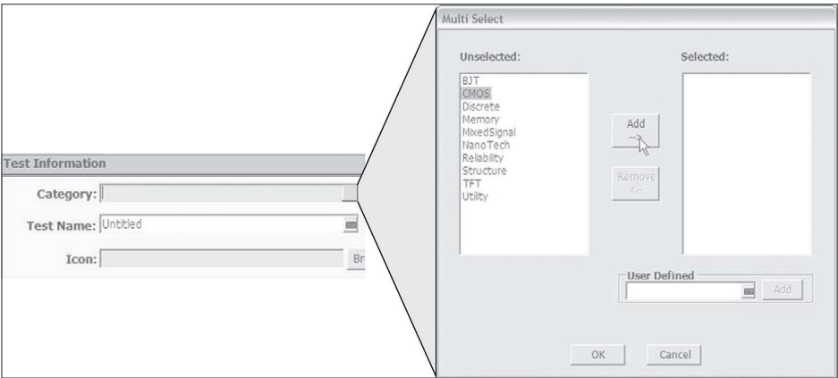
Figure 7. Selecting categories
