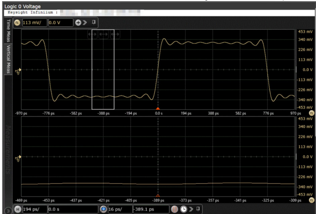
Figure 27 Reference Image for Crosstalk Source VMA (p-p) for Logic 0
