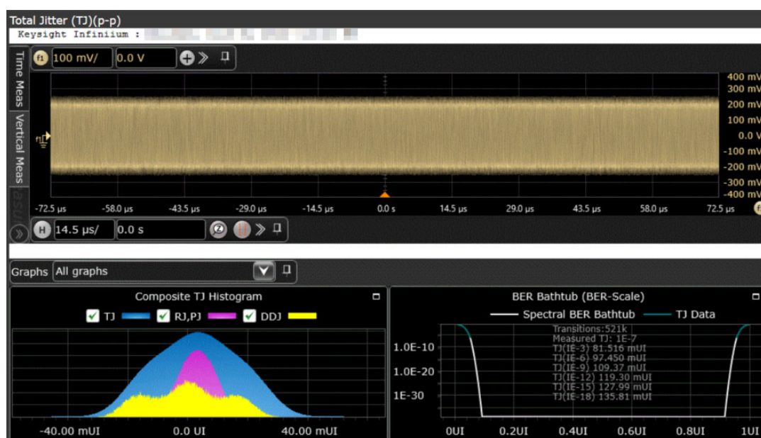
Figure 25 Reference Image for Total Jitter (TJ) (p-p) Test
