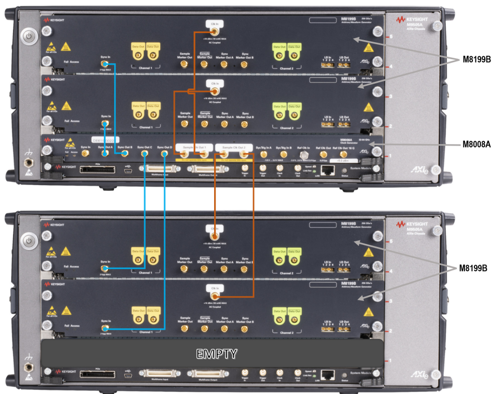
Figure 24 Connecting M8008A clock generator to four M8199B AWG modules
