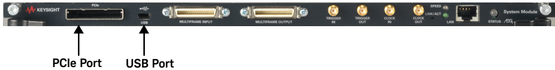
Figure 2 AXIe Embedded System Module
