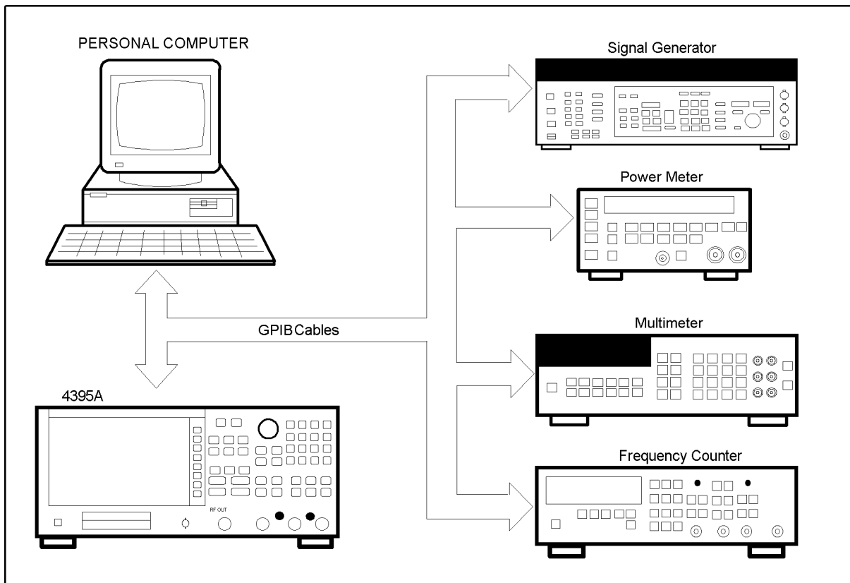
Figure 5-1. Adjustment Hardware Setup
