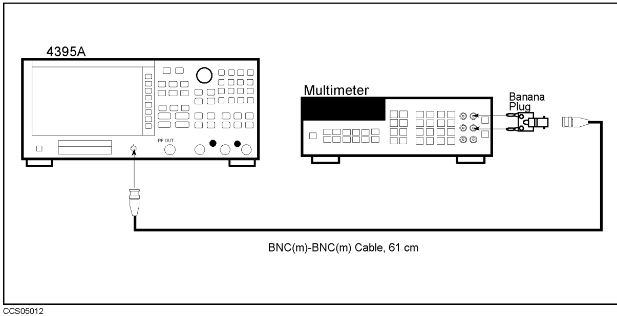
Figure 5-20. DC Bias Adjustment Setup 2
