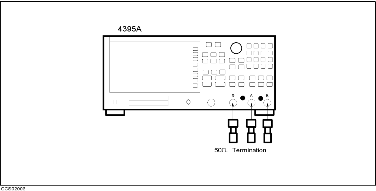
Figure 2-9. Receiver Noise Level Test Setup
