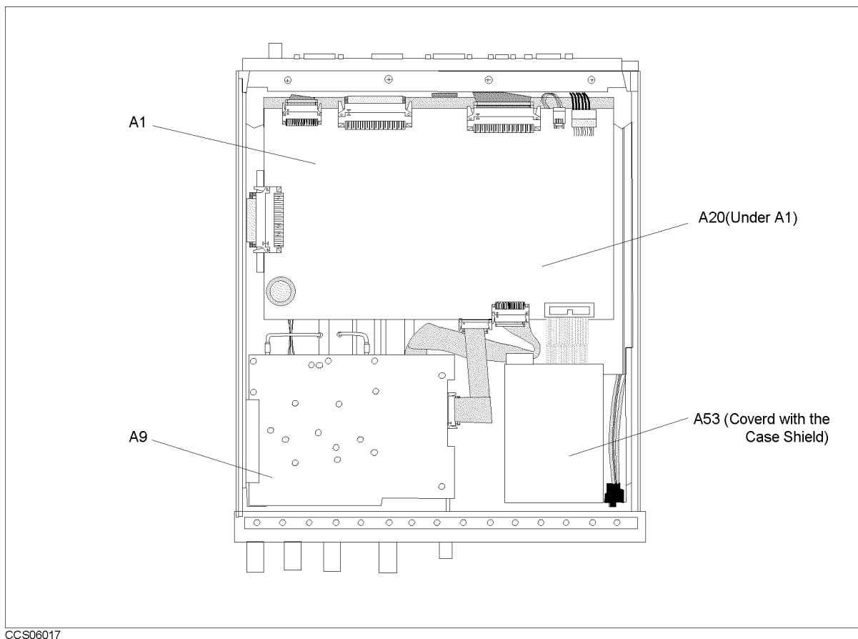
Figure 10-2. Bottom View (Major Assemblies)
