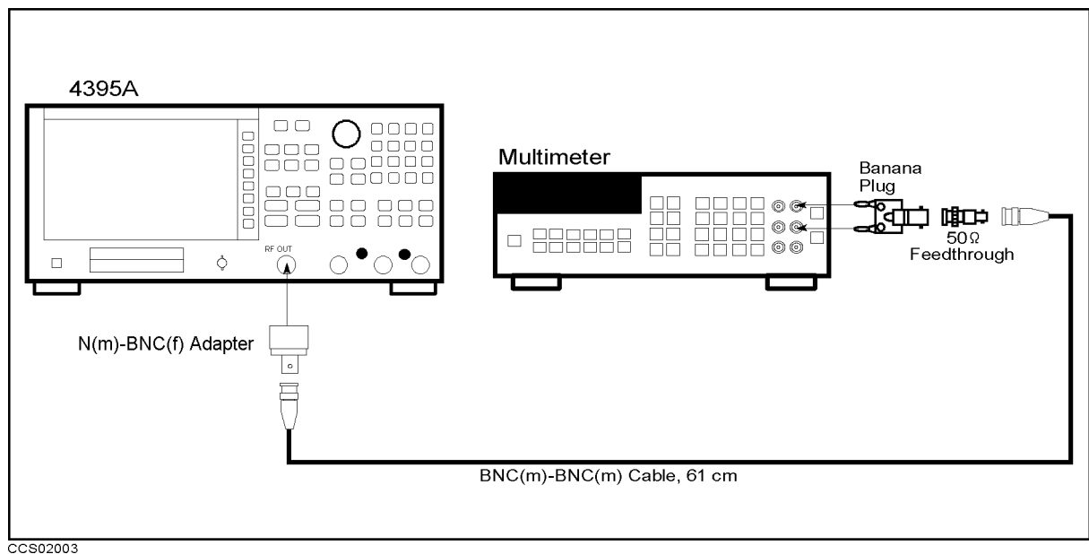
Figure 2-3. Source Level Flatness Test Setup
