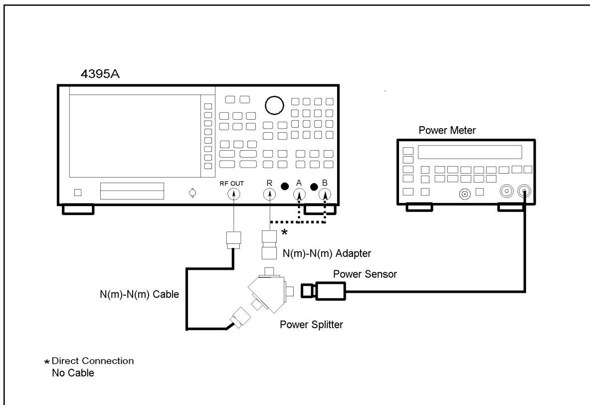
Figure 2-13. Absolute Amplitude Accuracy Test Setup 2
