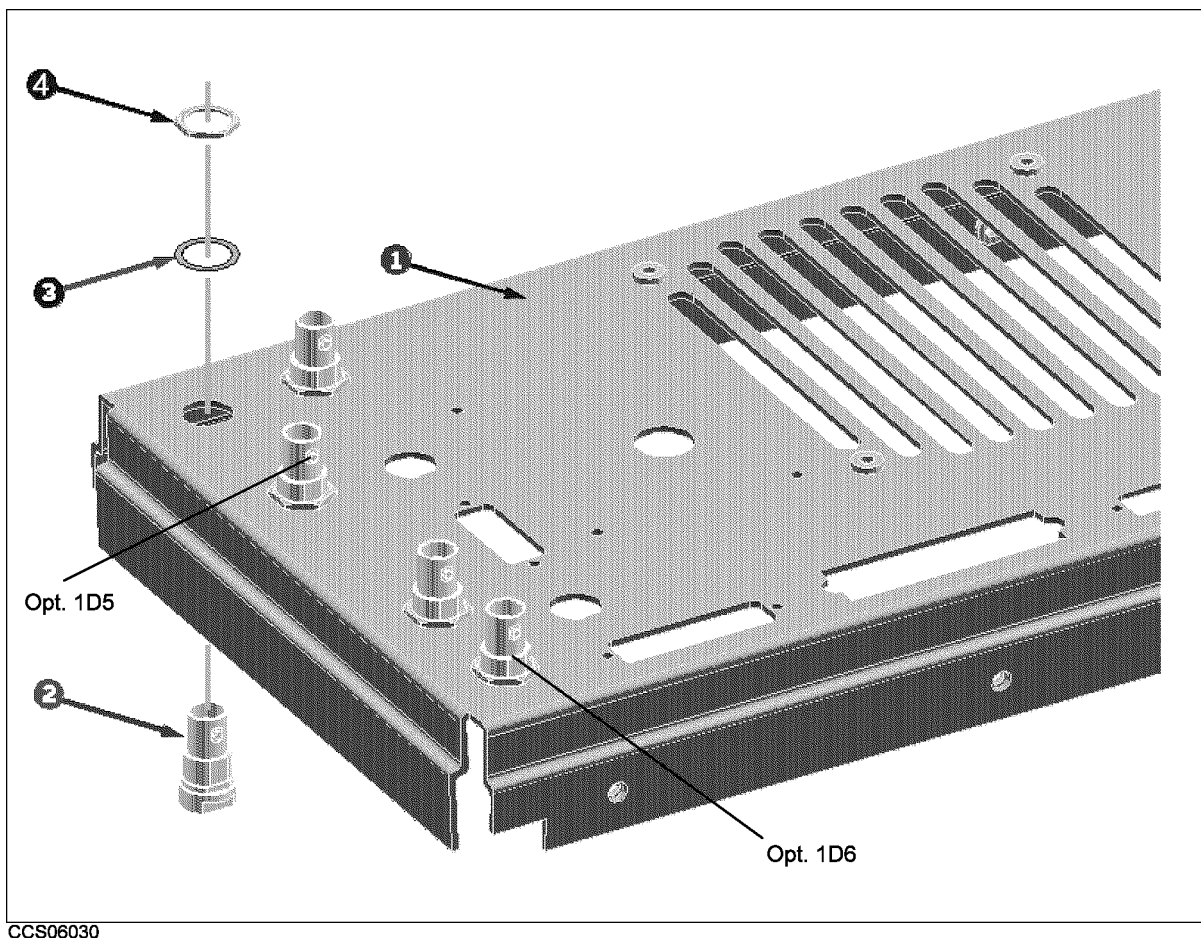
Figure 10-16. Rear Assembly Parts 1/8
