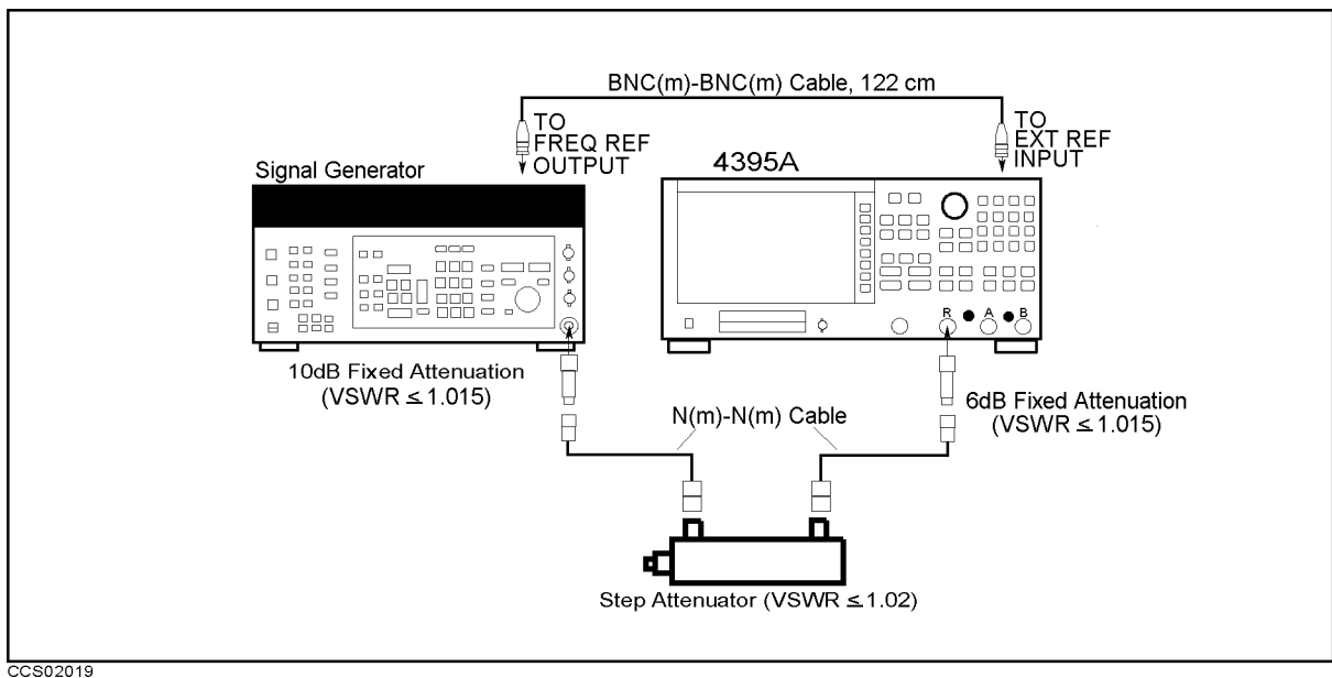
Figure 2-21. Amplitude Fidelity Test Setup 1
