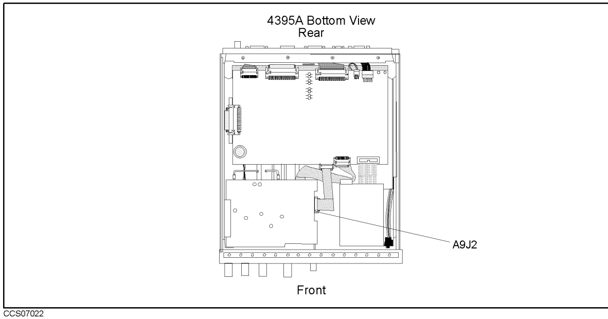
Figure 7-5. A1 CPU Connector Locations
