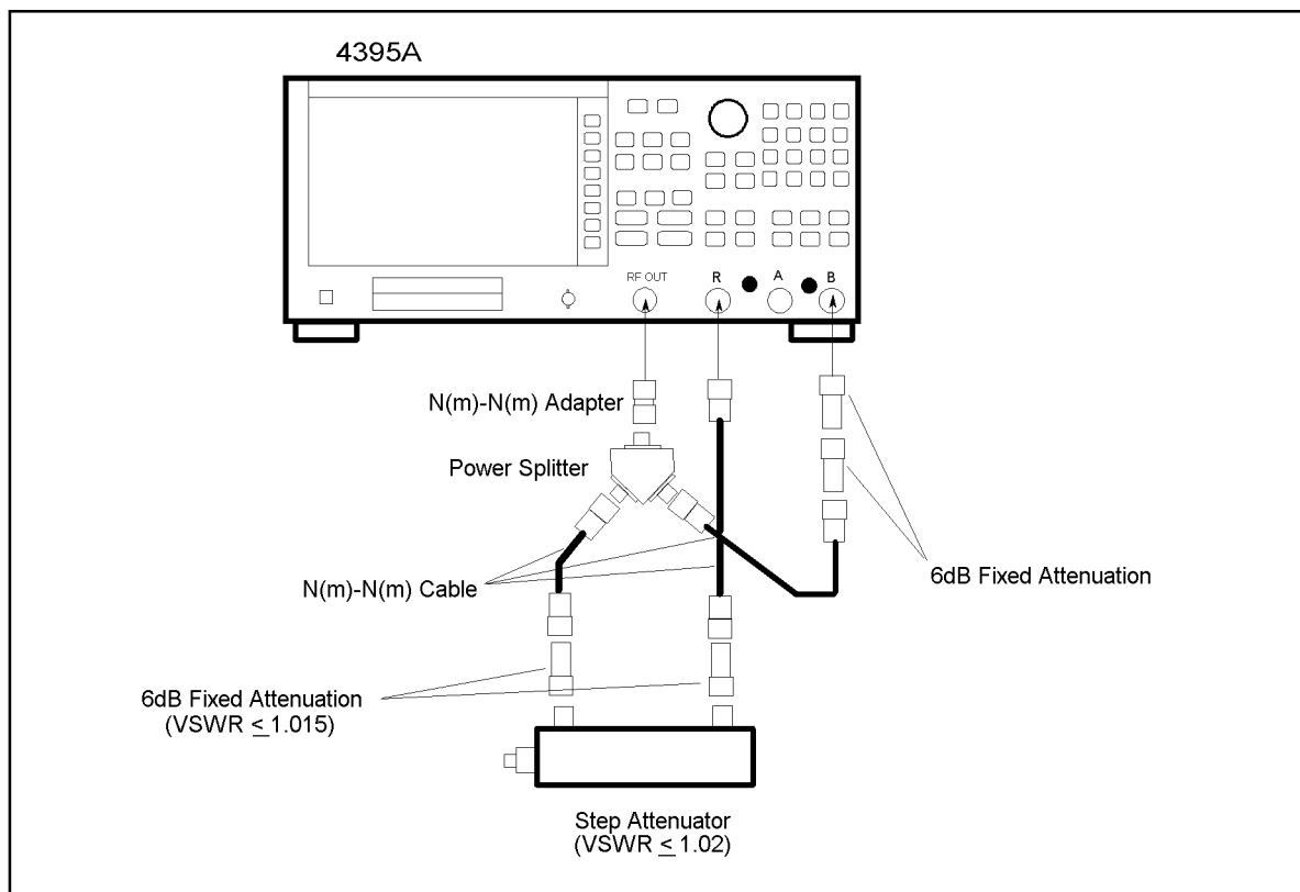
Figure 2-16. B/R Magnitude Ratio/Phase Dynamic Accuracy Test Setup 1
