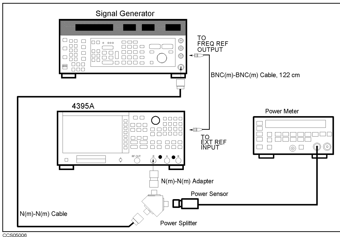
Figure 5-14. IF 8 dB/16 dB Gain Adjustment Setup
