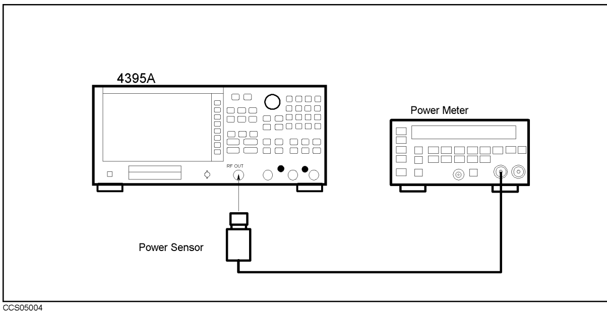
Figure 5-7. Source Power Adjustment Setup
