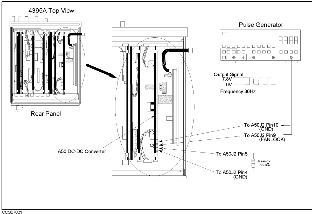
Figure 7-9. A50 DC-DC Converter Troubleshooting Setup
