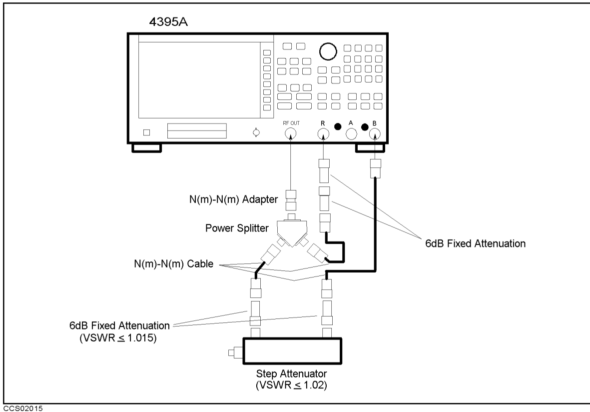
Figure 2-17. B/R Magnitude Ratio/Phase Dynamic Accuracy Test Setup 2
