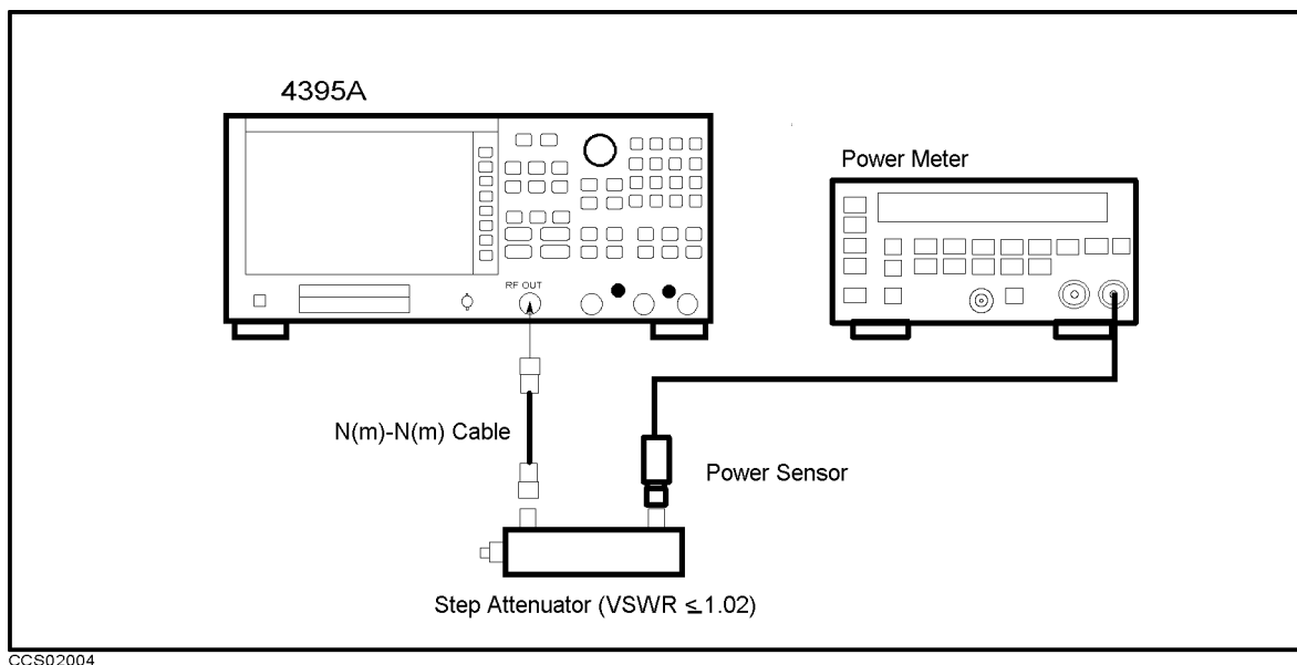
Figure 2-4. Non-sweep Power Linearity Test Setup
