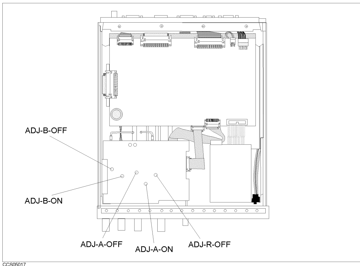
Figure 5-8. Input DC Offset Adjustment Location
