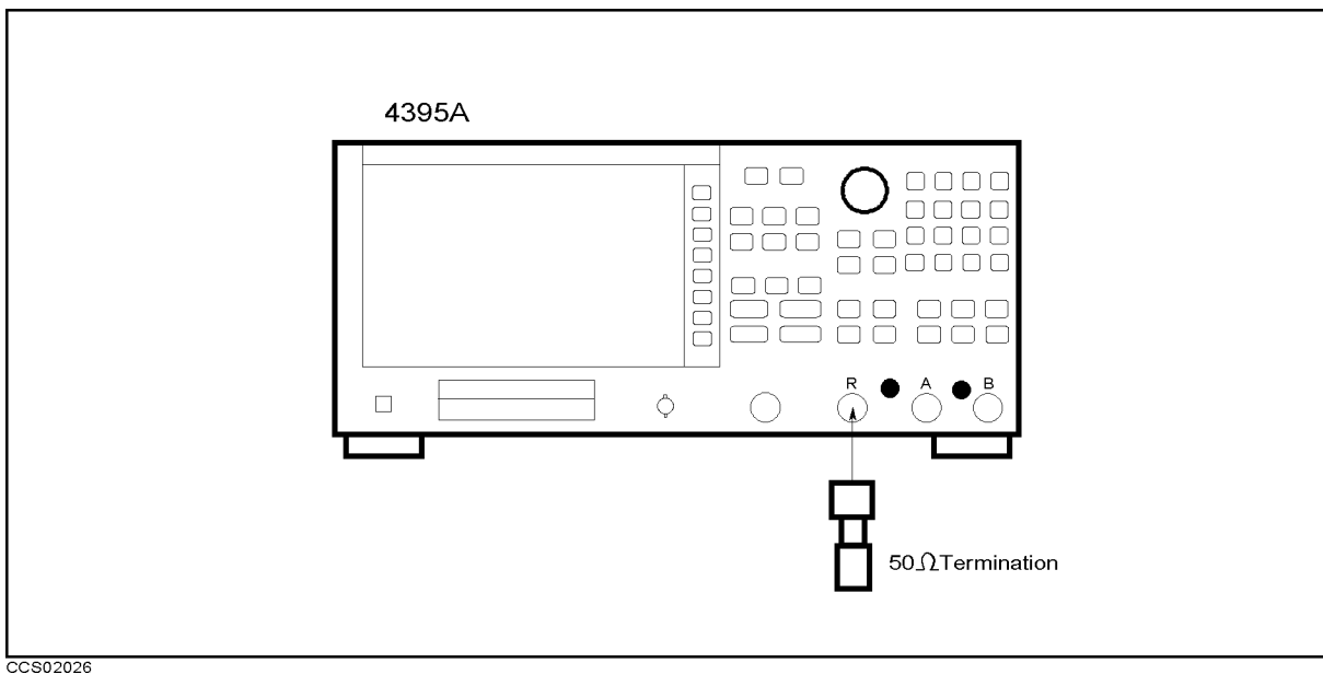
Figure 2-30. Residual Response Test Setup
