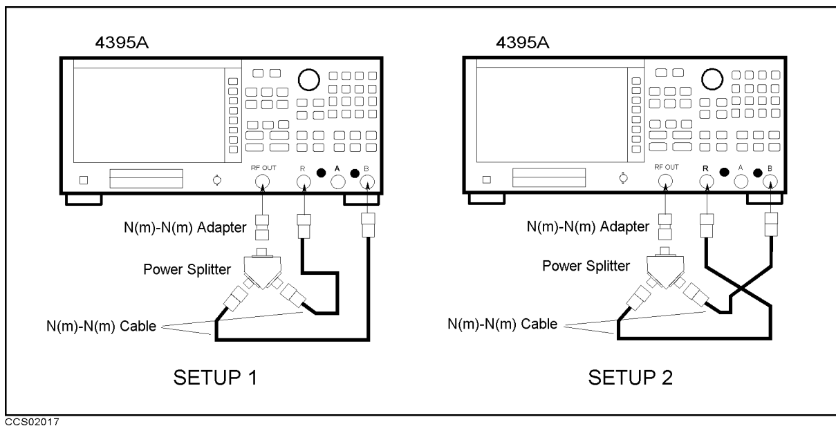
Figure 2-19. B/R Magnitude Ratio/Phase Frequency Response Test Setup
