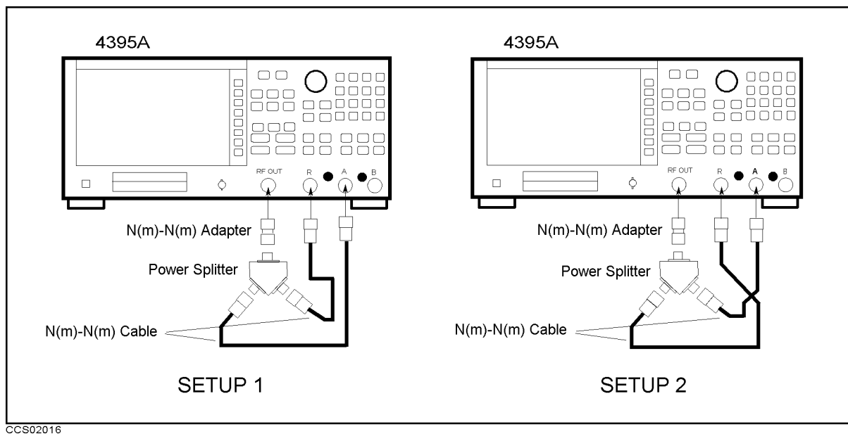
Figure 2-18. A/R Magnitude Ratio/Phase Frequency Response Test Setup
