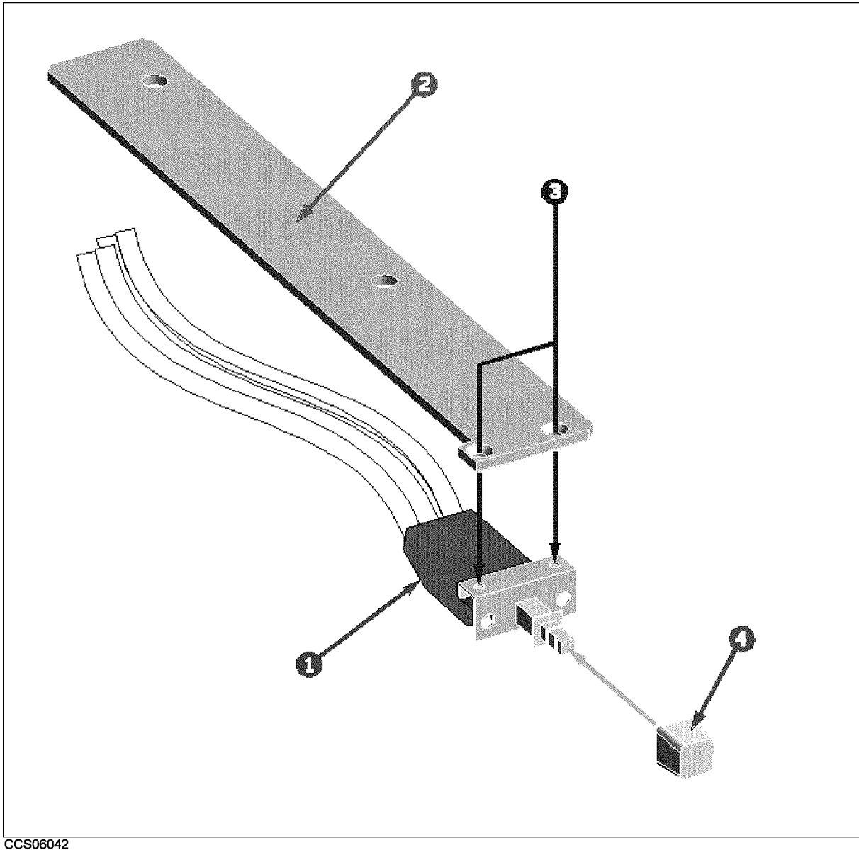
Figure 10-28. Main Frame Assembly Parts 5/23
