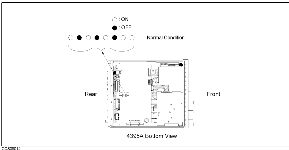
Figure 8-5. A1 Eight LEDs' Pattern
