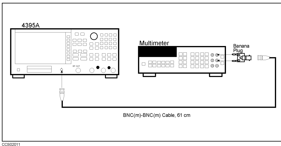
Figure 2-7. DC Bias Voltage Level Test Setup
