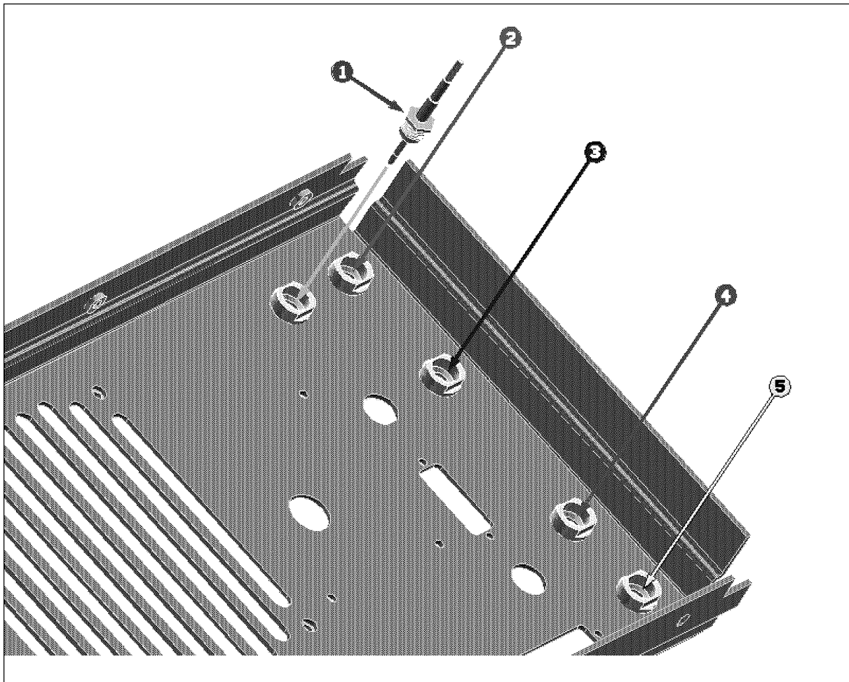
Figure 10-17. Rear Assembly Parts 2/8
