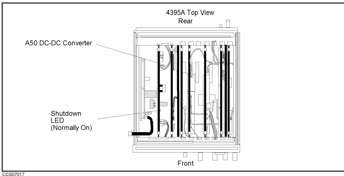
Figure 7-2. A50 SHUTDOWN LED Location
