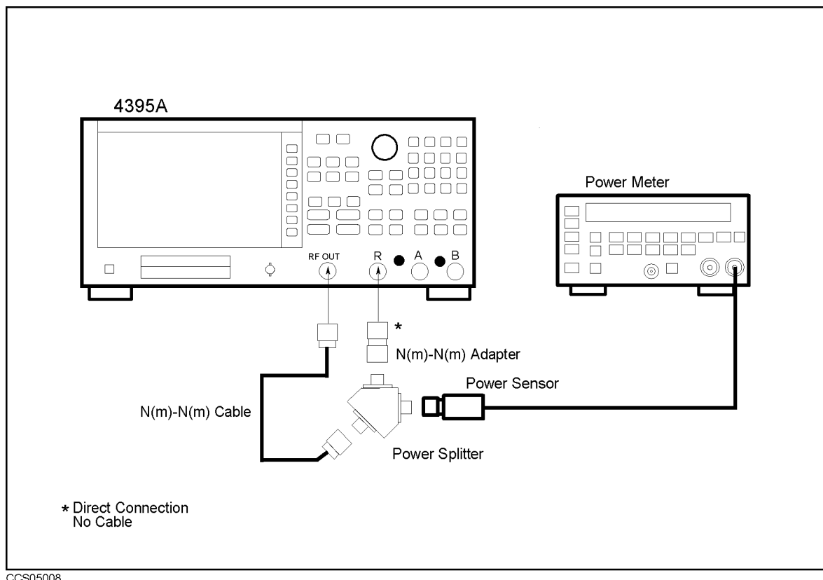
Figure 5-16. Receiver Flatness Adjustment Setup ( \geq 1 MHz)
