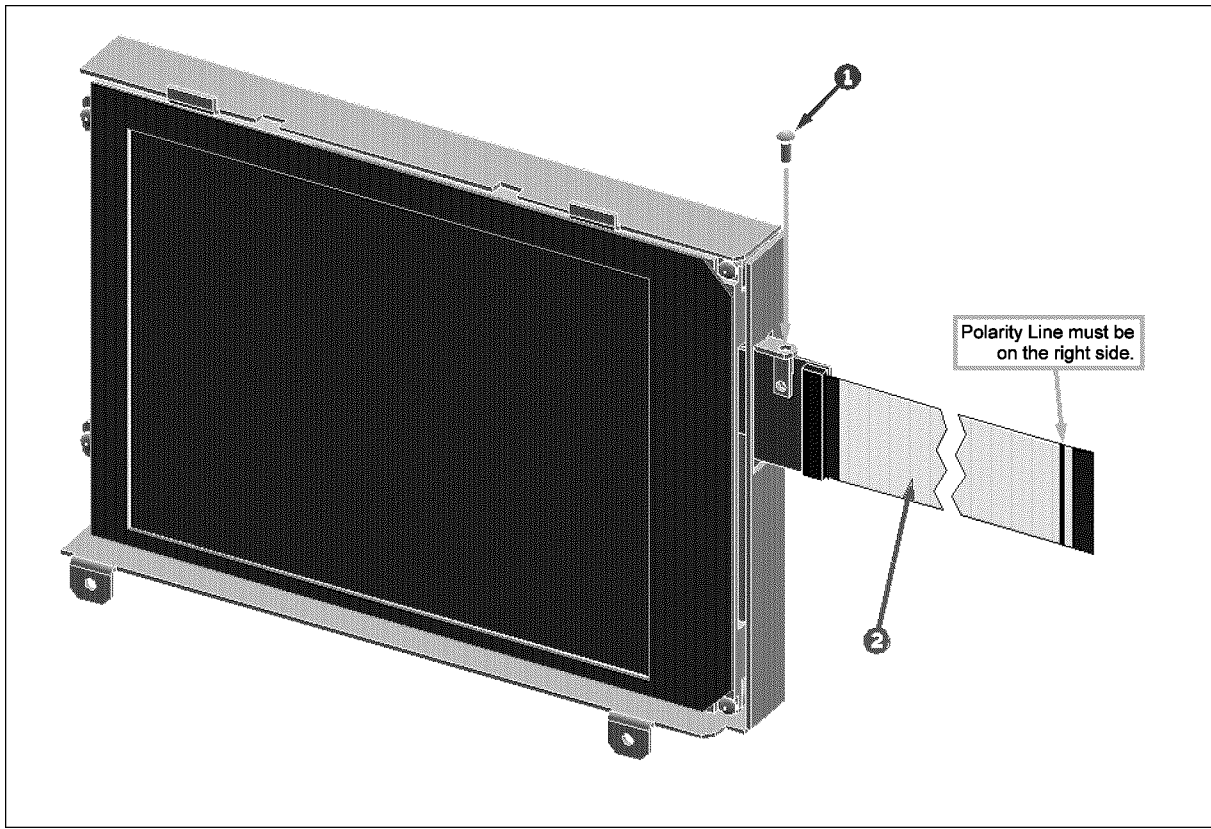
Figure 10-13. Front Assembly Parts 6/8
