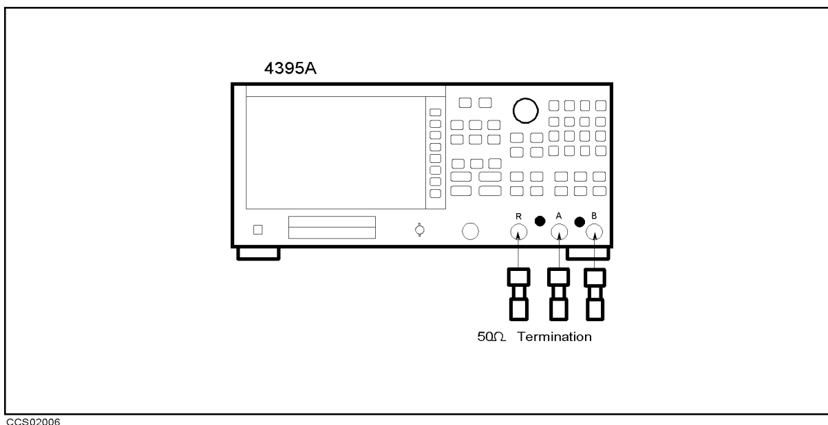
Figure 2-20. Average Noise Level Test Setup
