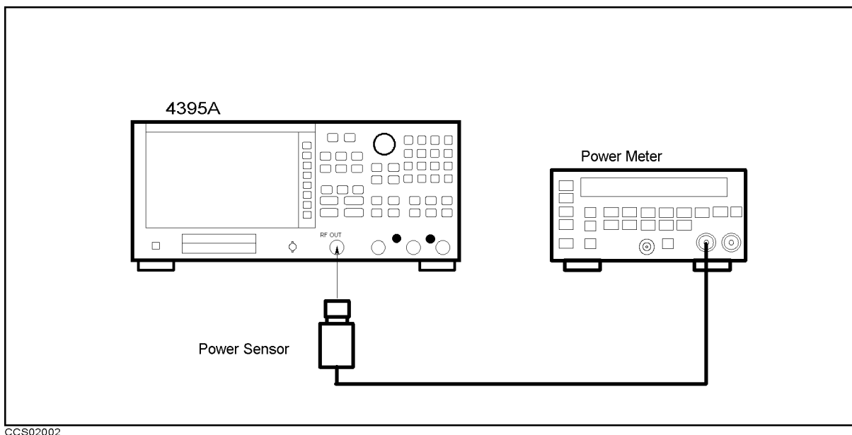
Figure 2-2. Source Level Accuracy Test Setup
