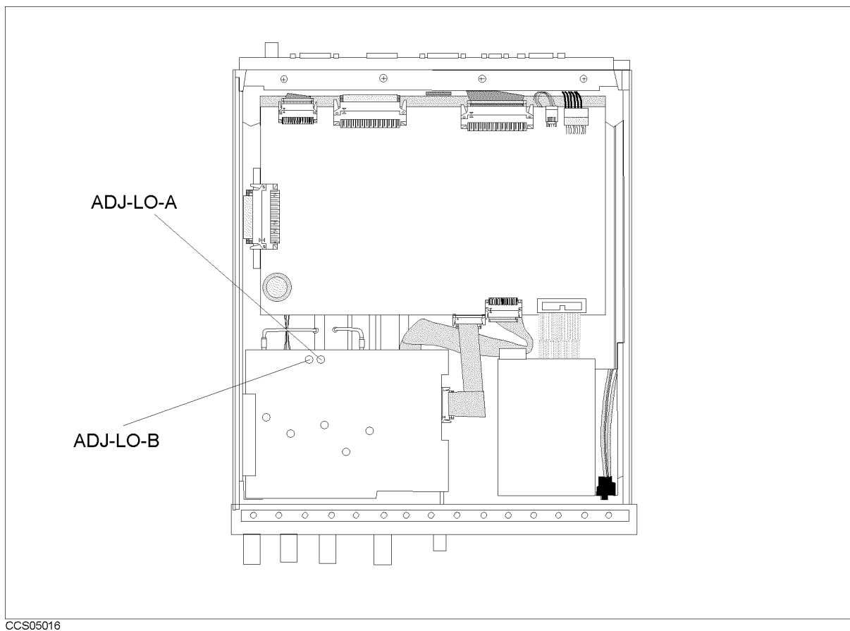
Figure 5-9. Input Local Null Adjustment Location
