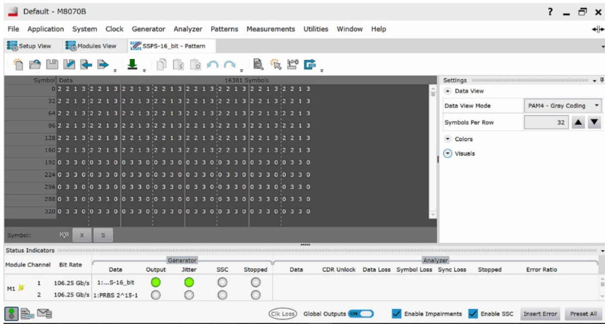
Figure 17. The pattern editor in the M8070B software allows editing NRZ bits and PAM4 symbols. The PAM4 symbol to bit mapping can be selected as Gray coded or custom with adjustable PAM4 levels. Quaternary PRBS, like QPRBS13-CEI or QPRBS31, according to CEI and IEEE standards can be selected as well as SSPRQ and PAM4 linearity test patterns.
