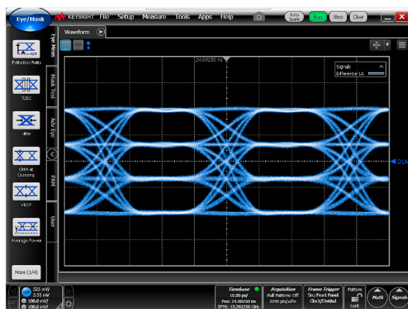
Figure 4. Clean 26.5625 Gbaud PAM4 output signal of pattern generator module M8045A with remote head M8057B using the internal clock source with 600 mV output amplitude and PRBS 2^{15}-1 . Measured with Infiniium DCA-X 86100D and N1045A and manual de-emphasis adjustment.
