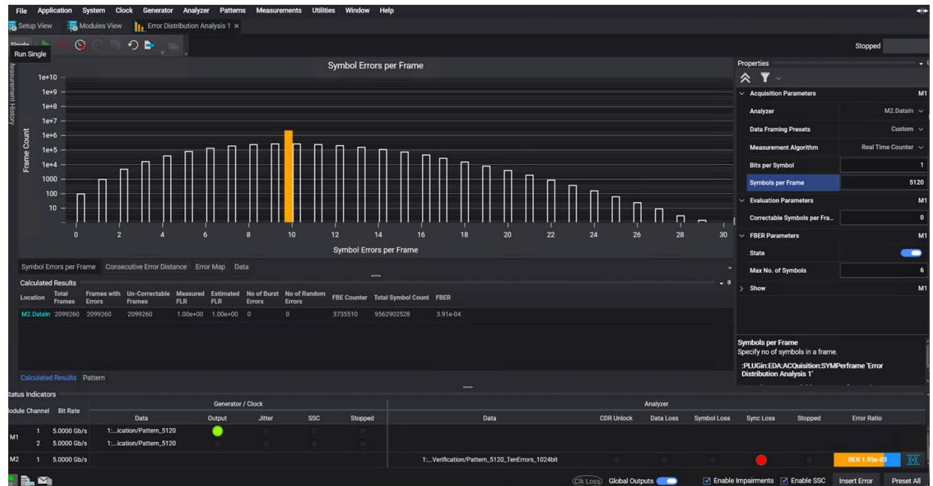
Figure 25. The error distribution analysis M8070EDAB provides multiple views to debug the error distribution. The figure shows an example of symbol errors per frame based on captured pattern streams, with the measured frame loss ratio, based on user-definable number of bits per symbol, correctable symbols per frame and frame length.
