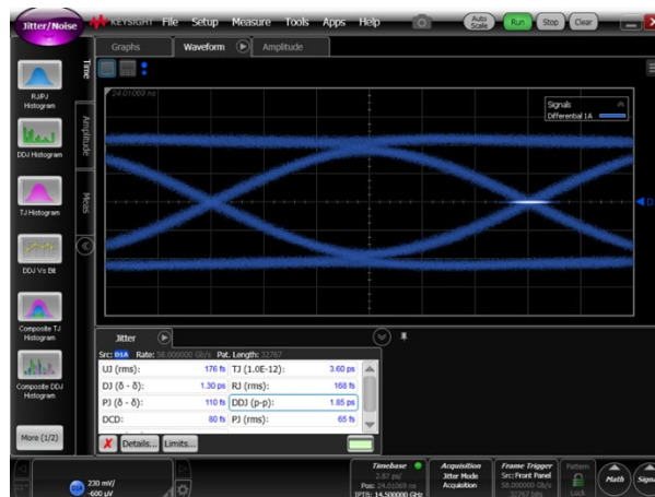
Figure 5. Clean 58 Gbaud NRZ output signal of pattern generator module M8045A with remote head M8057B using the internal clock source with 600 mV output amplitude and PRBS 2^{15}-1 . Measured with Infiniium DCA-X 86100D with N1045A and manual de-emphasis adjustment.
