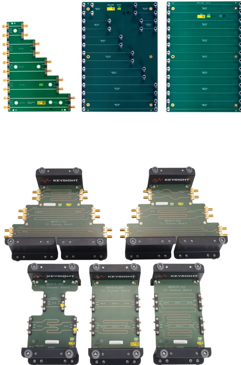
Figure 17. Emulate channel loss for receiver margin testing with Keysight's ISI channel boards
