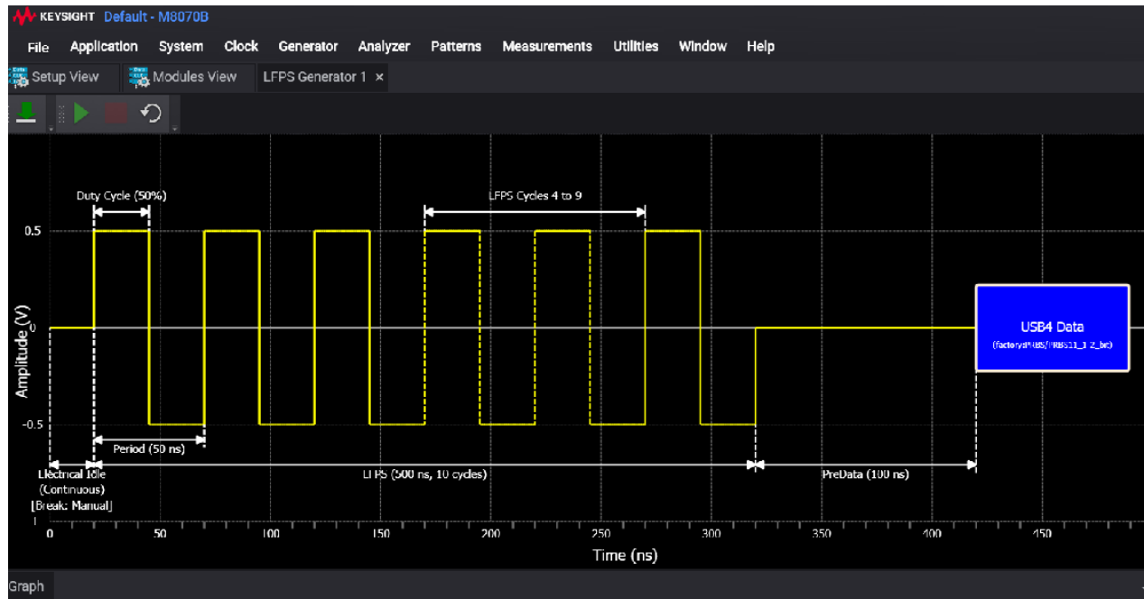
Figure 15. The USB4 LFPS generator utility.
