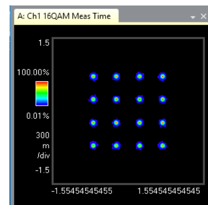
Figure 2. QAM16 at 64 GBaud
