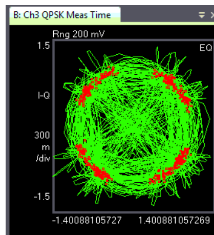
Figure 1. QPSK signal with emulated phase noise
