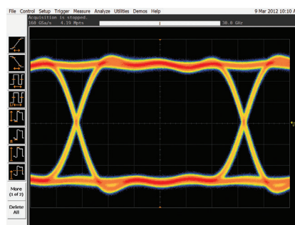
10 Gbps eye captured with 30 GHz of bandwidth
