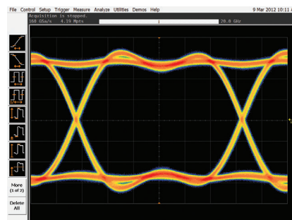
10 Gbps eye captured with 20 GHz of bandwidth
