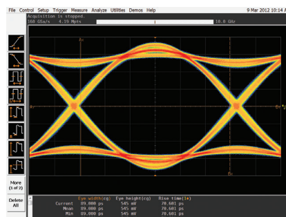
10 Gbps eye captured with 10 GHz of bandwidth
