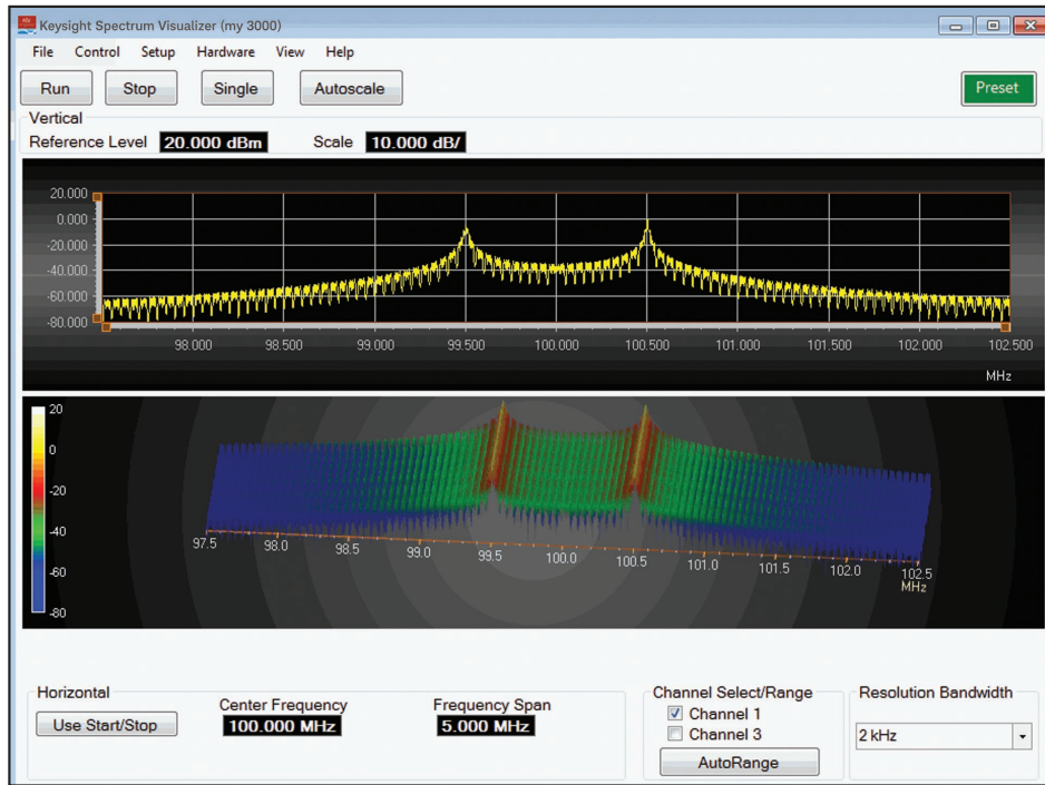
Figure 2. Waterfall view for ASV spectrogram measurement.
