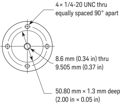
Flanged Shaft
