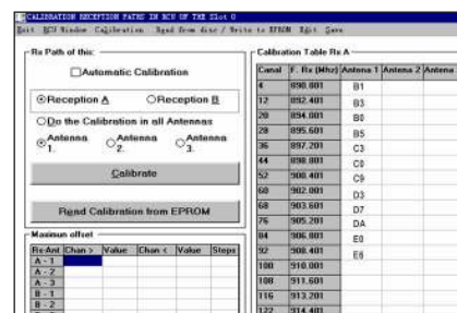
Figure 2. Base Station RX Level Calibration Software
