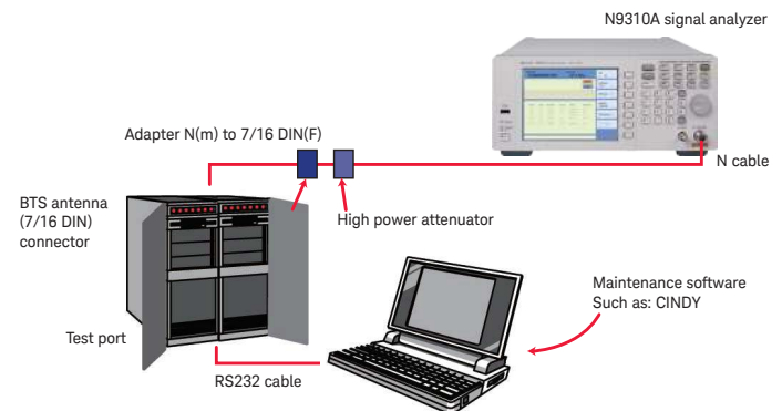
Figure 1. System connection
