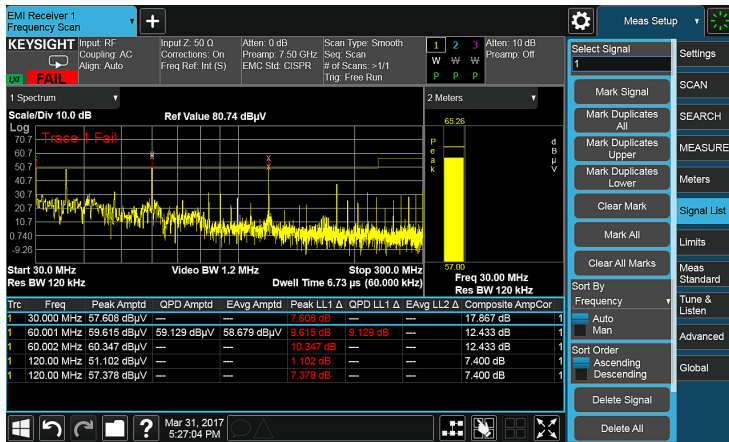
Figure 12. Duplicate ambient signals marked.
