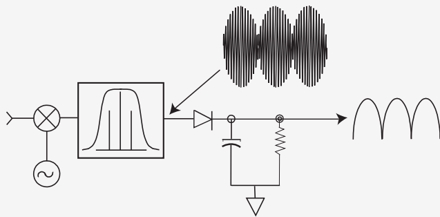
Figure D-1. Peak detector diagram.
