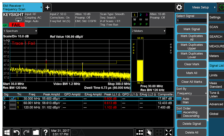
Figure 11. Mark ambient noise and delete it.
