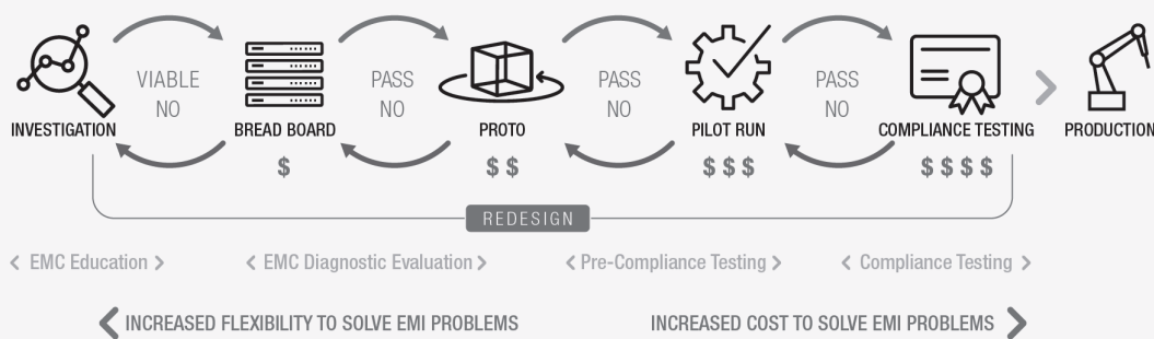
Figure 1. A typical product development cycle, including EMI testing.
