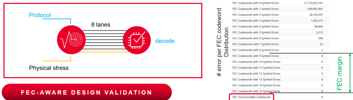
Figure 1. Principle of 400GAUI-8 FEC-aware layer 1 testing
