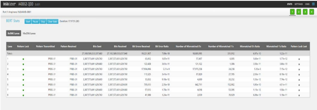
Figure 4. 400GAUI-8 lanes statistics in PRBS mode view
