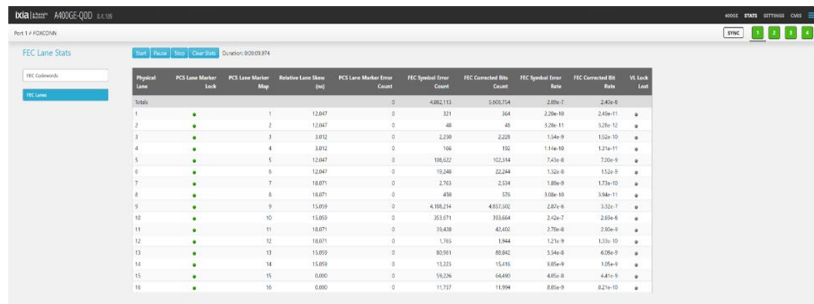
Figure 2. PCS lanes statistics in 400GE KP4 mode view
