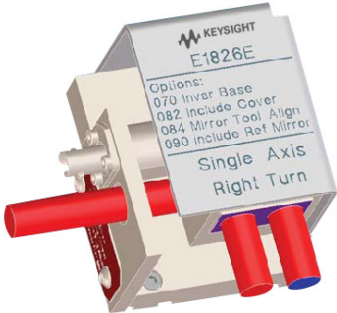
Keysight E1826E One-Axis Plane Mirror Interferometer Right Turn Configuration
