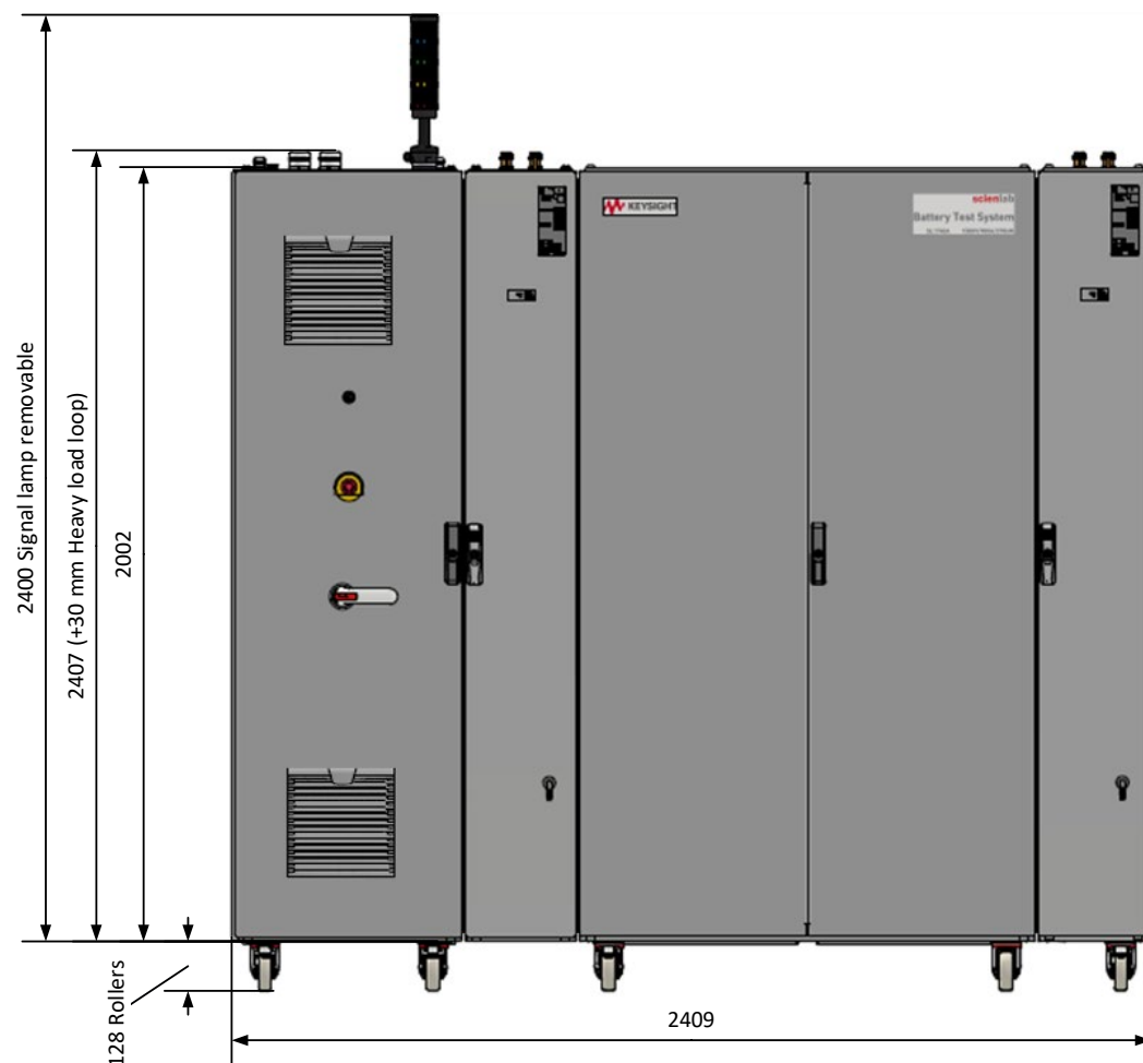
Figure 4. 300 kW System – front view incl. dimensions in mm
