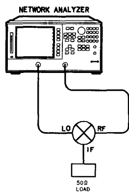
Figure 3-18. Connections for a Mixer Isolation Measurement
