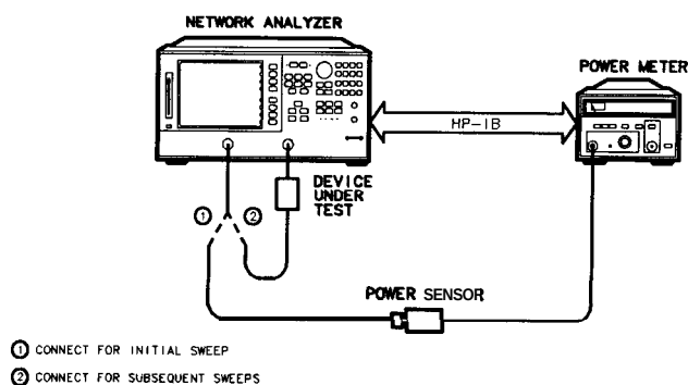
Figure 5-7. Continuous Correction Mode for Power Meter Calibration
