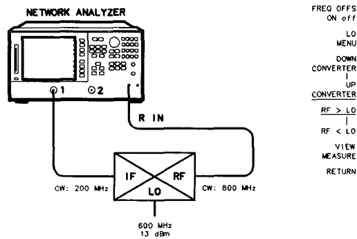
Figure 3-15. Measurement Setup Diagram Shown on Analyzer Display
