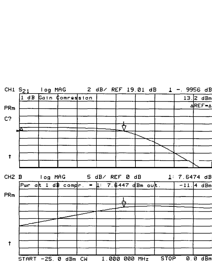
Figure 2-13. Gain Compression using Power Sweep
