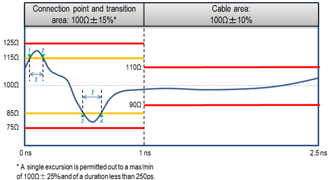
Figure 5-6 Connection point and transition area and Cable area limits for Differential Impedance
