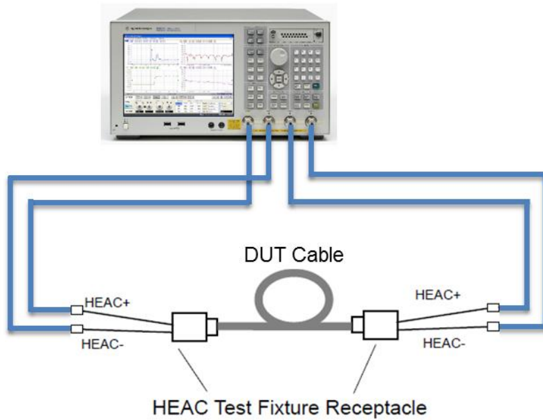
Figure 5-2 Measurement setup example
