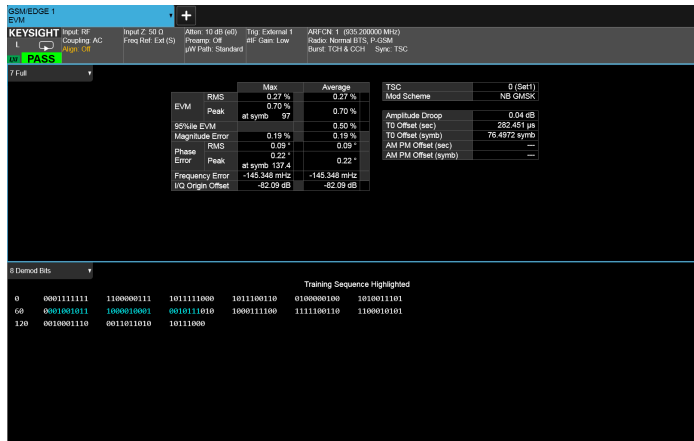
Figure 1. EVM and demodulated bits for GMSK modulation signals. Training sequences are highlighted.
