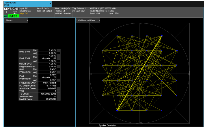
Figure 2. Constellation diagram and error summary of an HSR 32QAM EDGE Evolution signal.
