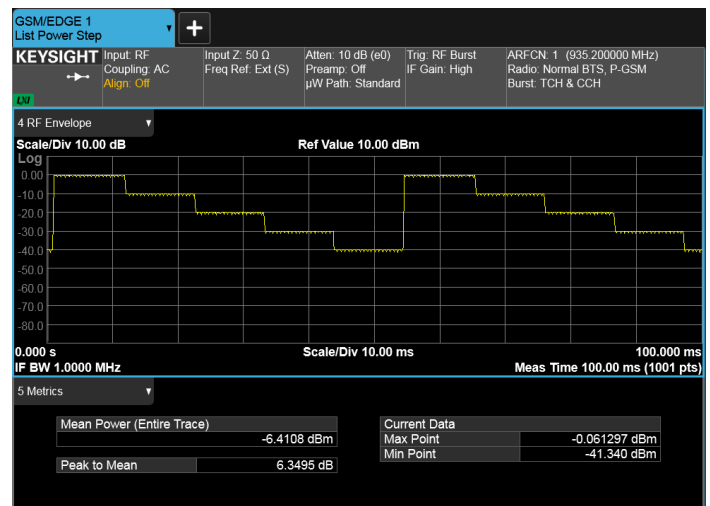
Figure 4. GSM list power step measurement.
